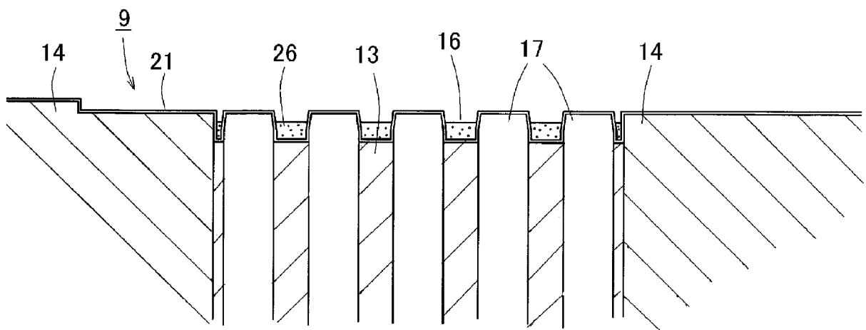
図6B
