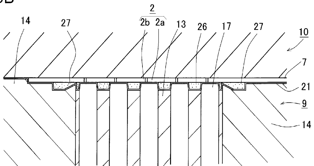
図9B
