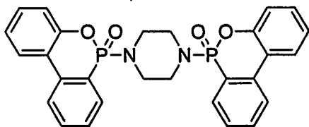
6,6'-(piperazine-1,4-diyl)bis(6H-dibenzo[c,e][1,2]oxaphosphinine 6-oxide) (PB-DOPO)
