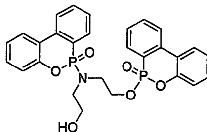
6-((2-hydroxyethyl)(2-((6-oxido-6 H -dibenzo[ c,e ] [1,2]oxaphosphinin-6-yl)oxy)ethyl)amino)-6 H -dibenzo[ c,e ] [1,2]oxaphosphinine 6-oxide (DEA-DDOPO)
