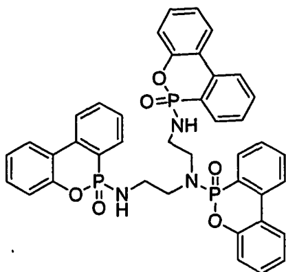
6-((3-((6-oxido-6H-dibenzo[c,e][1,2]oxaphosphinin-6-yl)(2-((6-oxido-6H-dibenzo[c,e][1,2]oxaphosphinin-6-yl)amino)ethyl)amino)propyl)amino)-6H-dibenzo[c,e][1,2]oxaphosphinine 6-oxide TDETA-DOPO
