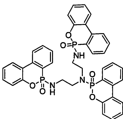
6-((3-((6-oxido-6 H -dibenzo[ c,e ][1,2]oxaphosphinin-6-yl)(2-((6-oxido-6 H - dibenzo[ c,e ][1,2]oxaphosphinin-6-yl)amino)ethyl)amino)propyl)amino)-6 H - dibenzo[ c,e ][1,2]oxaphosphinine 6-oxide TDETA-DOPO
