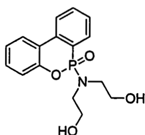
6-(bis(2-hydroxyethyl)amino)-6H-dibenzo[c,e][1,2]oxaphosphinine 6-oxide (BHEA-DOPO)
