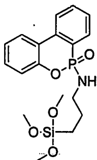
6-((3-(trimethoxysilyl)propyl)amino)- 6 H -dibenzo[ c,e ][1,2]oxaphosphinine 6-oxide (TMSPA-DOPO)
