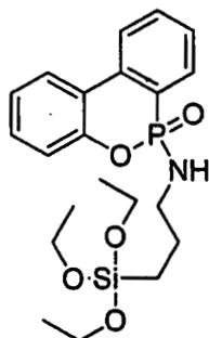
6-((3-(triethoxysilyl)propyl)amino)-6H-dibenzo[c,e][1,2]oxaphosphinine 6-oxide (TESPA-DOPO)
