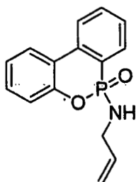
6-(allylamino)-6H-dibenzo[c,e][1,2] oxaphosphinine 6-oxide (AA-DOPO)
