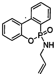
6-(allylamino)-6 H -dibenzo[ c,e ][1,2] oxaphosphinine 6-oxide (AA-DOPO)
