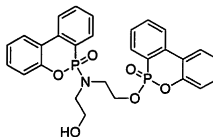
6-((2-hydroxyethyl)(2-((6-oxido-6H-dibenzo[c,e][1,2]oxaphosphinin-6-yl)oxy)ethyl)amino)-6H-dibenzo[c,e][1,2]oxaphosphinine 6-oxide (DEA-DDOPO)
