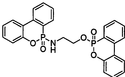
6-(2-((6-oxido-6 H -dibenzo[ c,e ][1,2]oxaphosphinin-6-yl)amino) ethoxy)-6 H -dibenzo[ c,e ][1,2]oxaphosphinine 6-oxide (EAB-DOPO)
