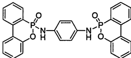
6,6'-(1,4-phenylenebis(azanediyl))bis(6 H -dibenzo[ c,e ][1,2] oxaphosphinine 6-oxide) (PDAB-DOPO)
