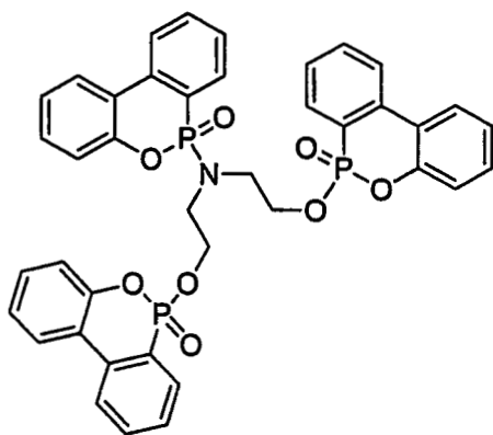
6,6'-((((6-oxido-6H-dibenzo[c,e][1,2]oxaphosphinin-6-yl)azanediyl)bis(ethane-2,1-diyl))bis(oxy))bis(6H-dibenzo[c,e][1,2]oxaphosphinine 6-oxide) (DEA-TDOPO)
