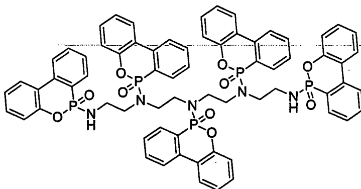
6,6'-((((6-oxido-6 H -dibenzo[ c,e ][1,2]oxaphosphinin-6-yl)azanediyl)bis(ethane-2,1-diyl))bis((2-((6- oxido-6 H -dibenzo[ c,e ][1,2]oxaphosphinin-6-yl)amino)ethyl)azanediyl))bis(6 H - dibenzo[ c,e ][1,2]oxaphosphinine 6-oxide)-(TEPA-PDOPO)
