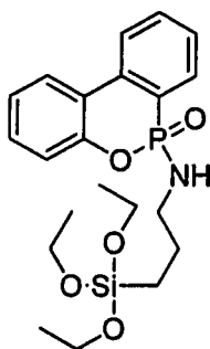
6-((3-(triethoxysilyl)propyl)amino)-6 H -dibenzo[ c,e ][1,2]oxaphosphinine 6-oxide (TESPA-DOPO)
