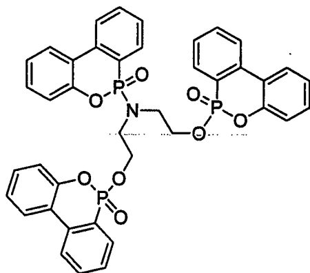
6,6'-((((6-oxido-6 H -dibenzo[ c,e ][1,2]oxaphosphinin-6- yl)azanediyl)bis(ethane-2,1-diyl))bis(oxy))bis(6 H - dibenzo[ c,e ][1,2]oxaphosphinine 6-oxide) (DEA-TDOPO)
