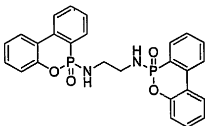
6,6'-(ethane-1,2-diylbis(azanediyl))bis(6H-dibenzo[c,e][1,2]oxaphosphinine 6-oxide) (EDAB-DOPO)
