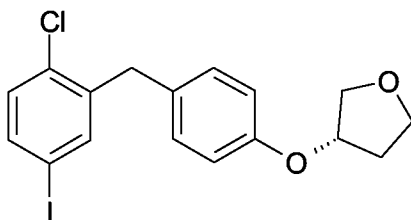
(S)-4-iodo-1-chloro-2-(4-tetrahydrofuran-3-yloxy-benzyl)-benzene
