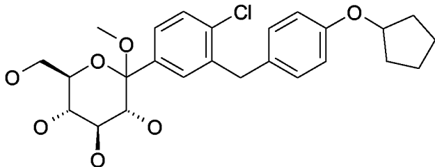
(2) 1-Chloro-4-(1-methoxy-D-glucopyranos-1-yl)-2-(4-cyclopentyloxy-benzyl)-benzene
