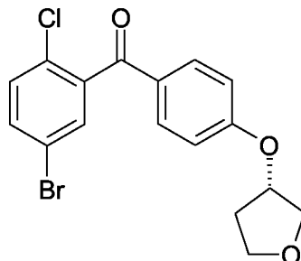
(5-bromo-2-chloro-phenyl)-(4-(S)-tetrahydrofuran-3-yloxy-phenyl)-methanone
