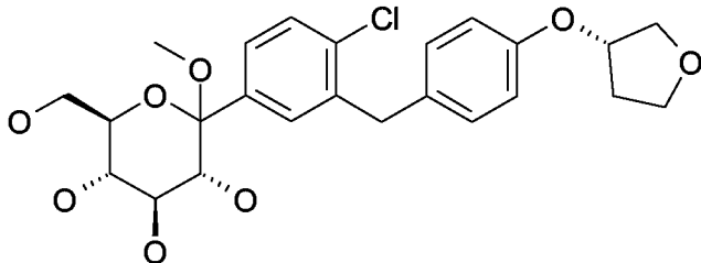
(2) 1-Chloro-4-(1-methoxy-D-glucopyranos-1-yl)-2-(4-cyclopentyloxy-benzyl)-benzene
