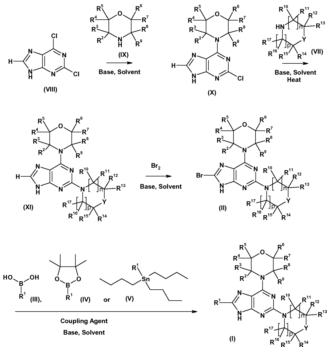
Scheme 1. General Procedure 1 for synthesis of purine compounds
