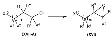
Scheme A2. Epoxidation via leaving group displacement.
