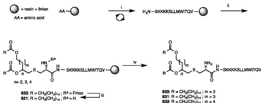
Scheme 2. (i) Iterative Fmoc-SPPS; (ii) ( R )-bis-pamitoylated Fmoc-Cys-OH 806 ( m=2 ) or 811 ( m=3 ) or 820 ( m=4 ), PyBOP, collidine, DMF; (iii) 20% piperidine/DMF; (iv)
