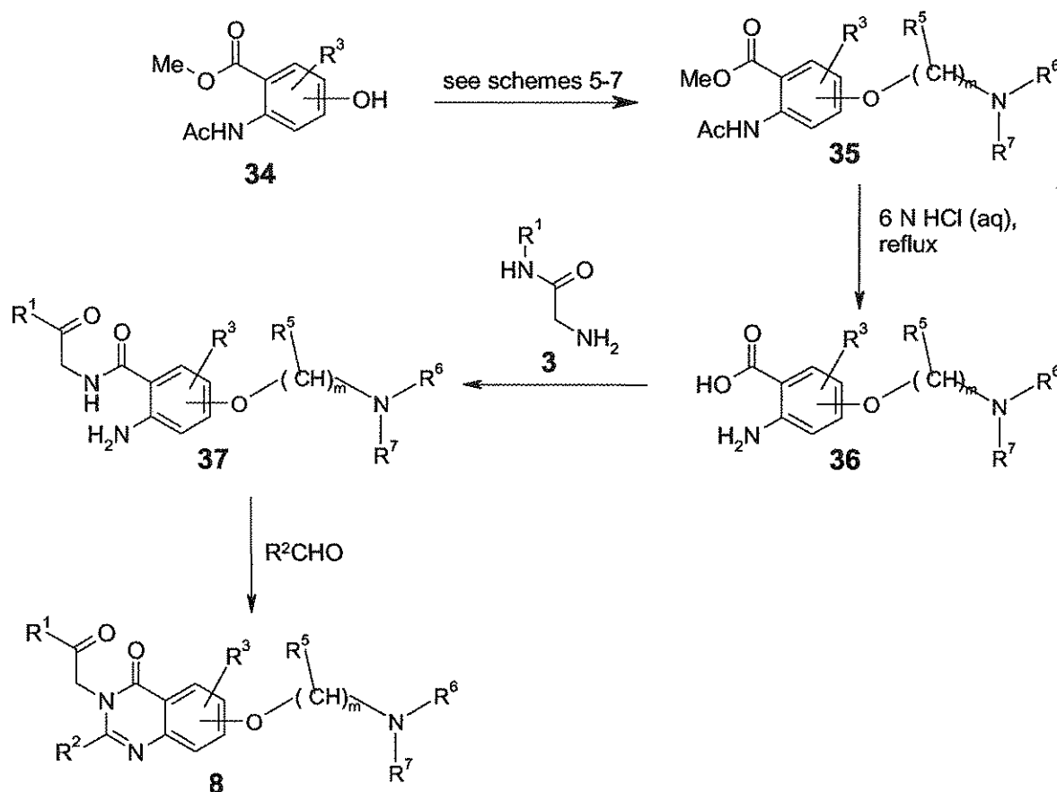
Scheme 12
