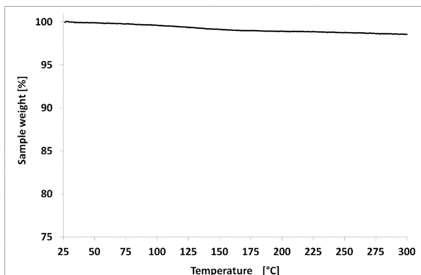
Figure 11: TGA scan of free base form NF5 (5 K/min)
