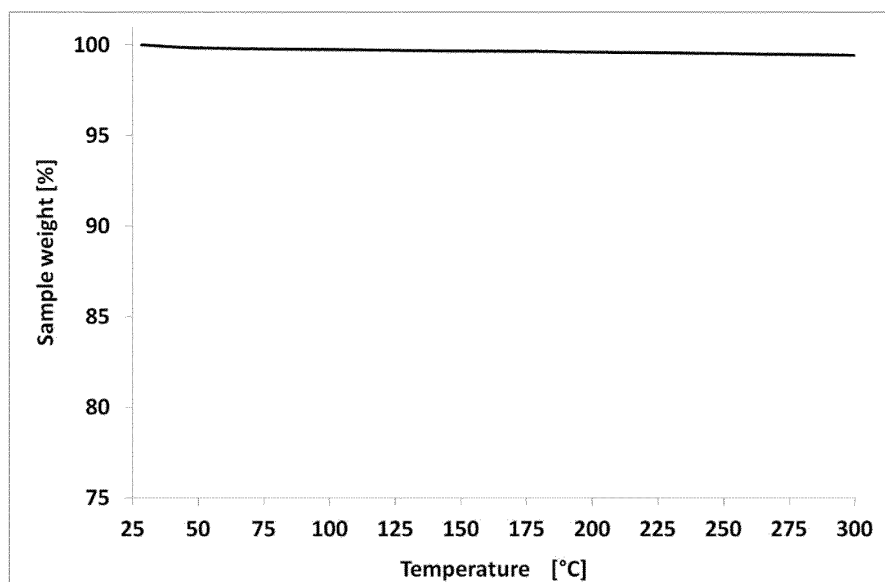
Figure 4: TGA scan of free base form A2 (5 K/min)
