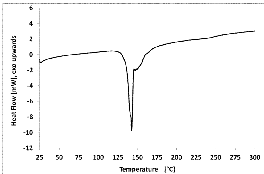
Figure 18: DSC scan of form Malonate-NF1 (5 K/min)
