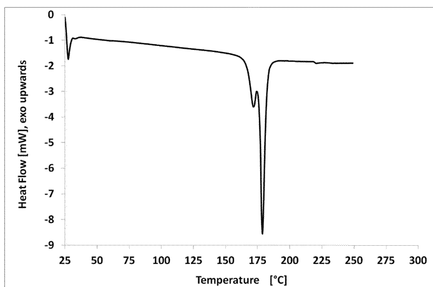
Figure 10: DSC scan of free base form NF5 (50 K/min)
