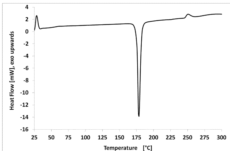
Figure 3: DSC scan of free base form A2 (50 K/min)
