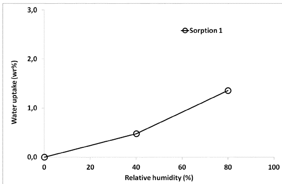
Figure 40: Water Vapour Sorption Isotherm (25 °C) of form Citrate-NF1
