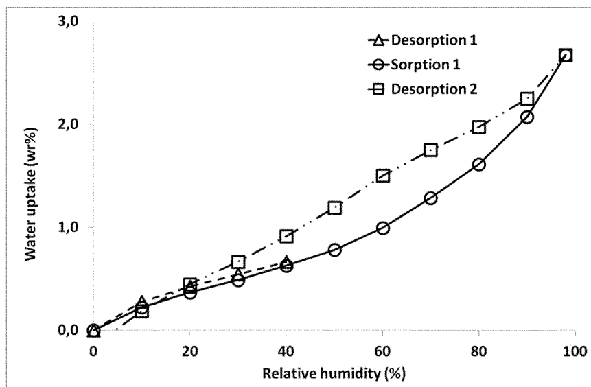
Figure 16: Water Vapour Sorption Isotherm (25 °C) of free base form NF6
