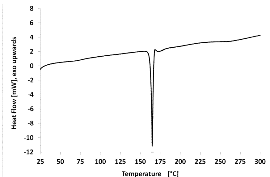
Figure 34: DSC scan of form Maleate-NF1 (5 K/min)
