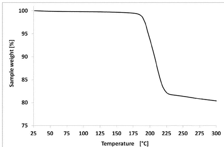
Figure 27: TGA scan of form Oxalate-NF1 (5 K/min)
