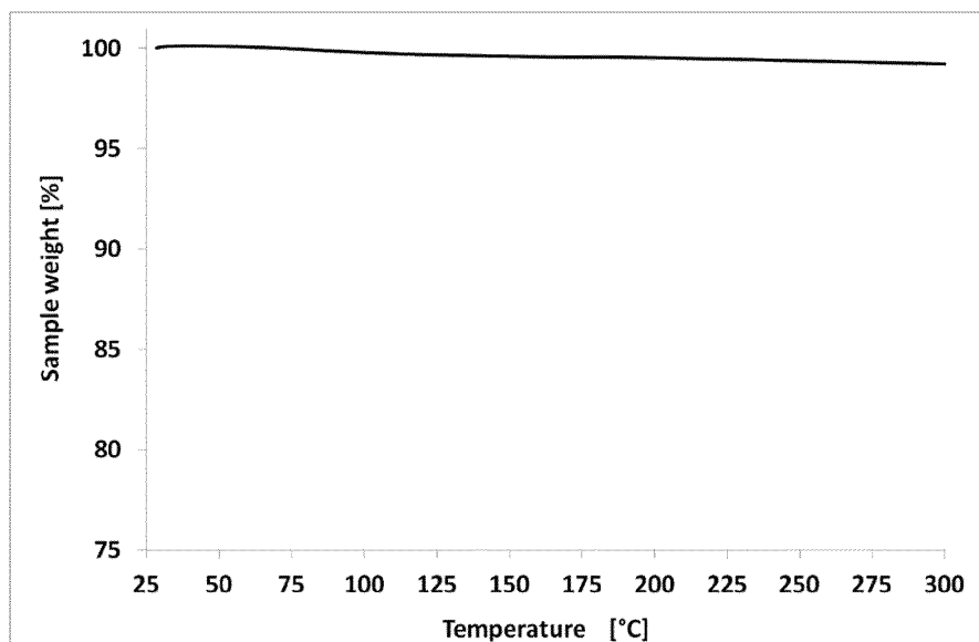
Figure 43: TGA scan of free base form A1 (5 K/min)
