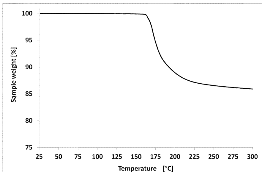
Figure 35: TGA scan of form Maleate-NF1 (5 K/min)
