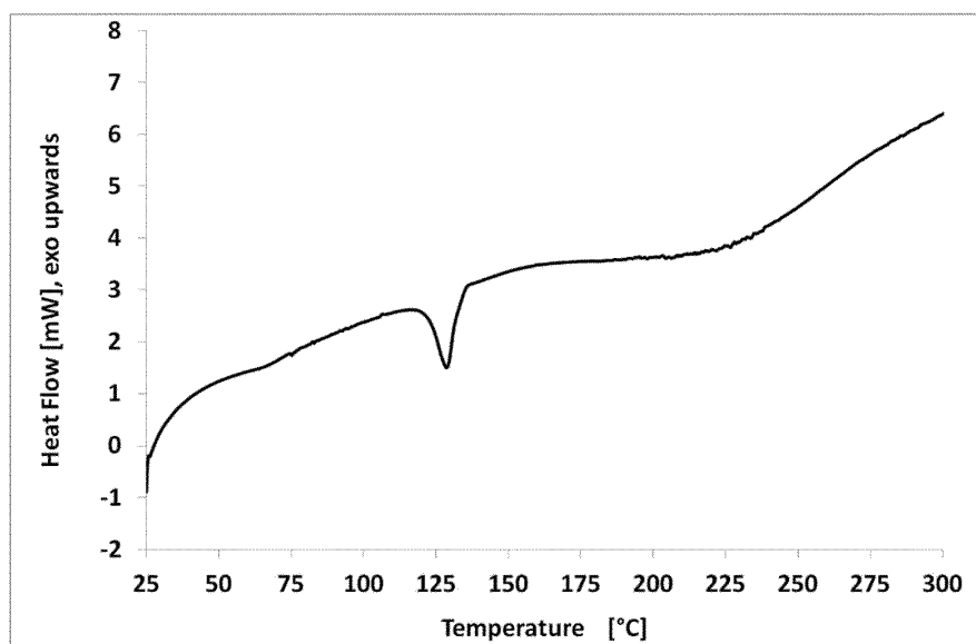
Figure 22: DSC scan of form Succinate-NF1 (5 K/min)
