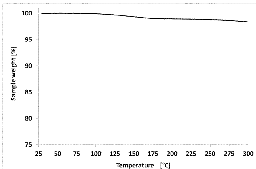
Figure 8: TGA scan of free base form NF4 (5 K/min)
