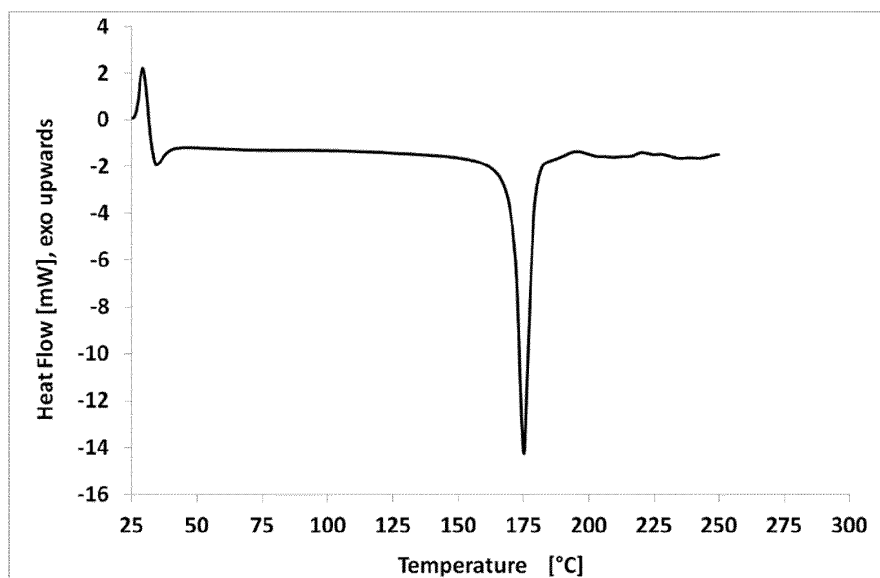
Figure 42: DSC scan of free base form A1 (50 K/min)
