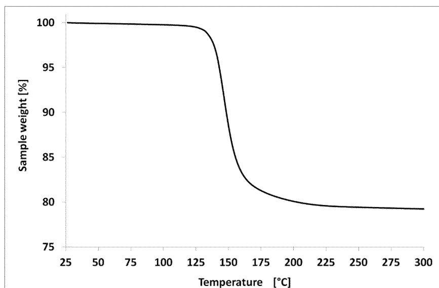
Figure 19: TGA scan of form Malonate-NF1 (5 K/min)
