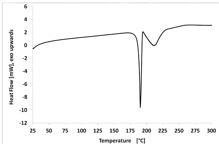
Figure 26: DSC scan of form Oxalate-NF1 (5 K/min)
