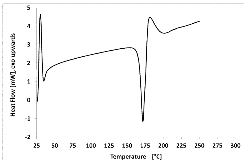
Figure 7: DSC scan of free base form NF4 (50 K/min)
