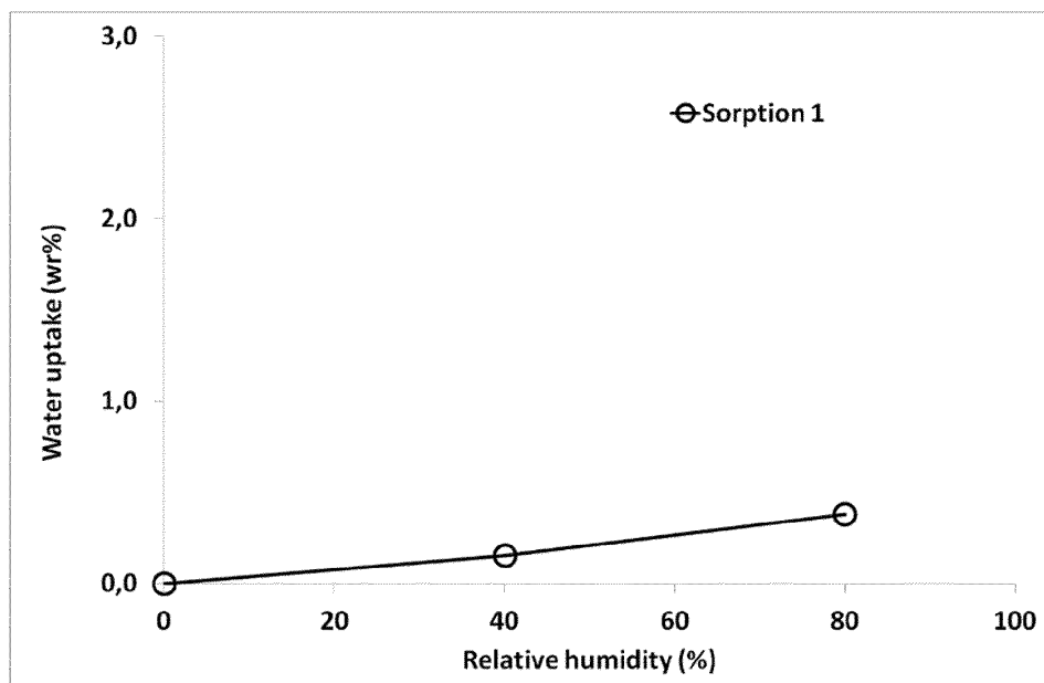
Figure 32: Water Vapour Sorption Isotherm (25 °C) of form Fumarate-NF1
