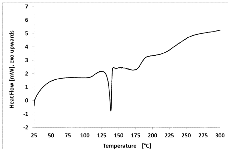
Figure 38: DSC scan of form Citrate-NF1 (5 K/min)
