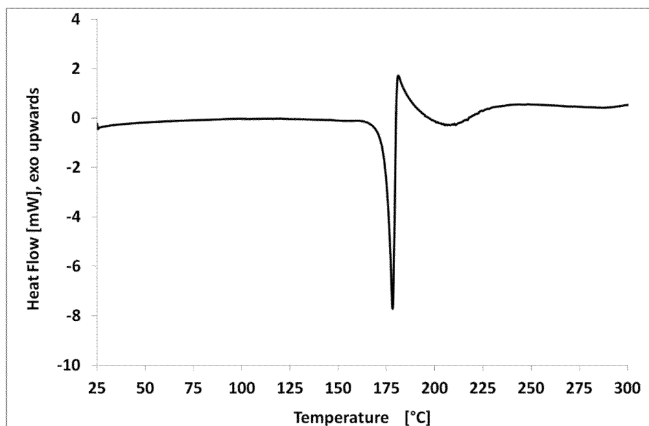
Figure 30: DSC scan of form Fumarate-NF1 (5 K/min)
