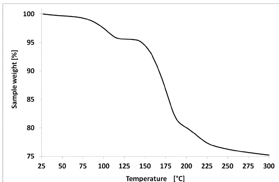
Figure 39: TGA scan of form Citrate-NF1 (5 K/min)
