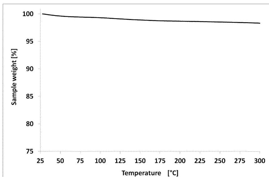
Figure 15: TGA scan of free base form NF6 (5 K/min)
