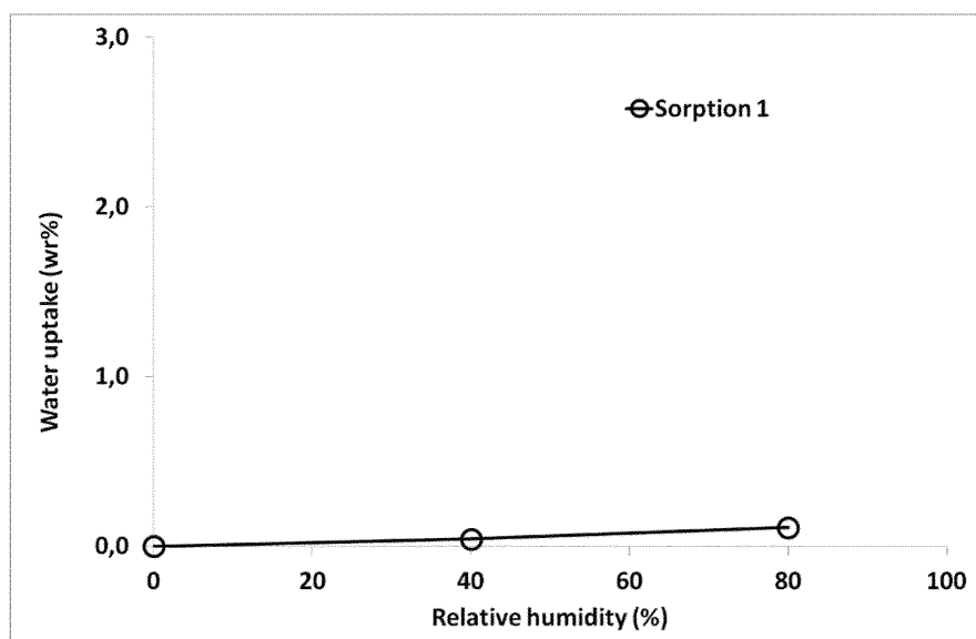
Figure 36: Water Vapour Sorption Isotherm (25 °C) of form Maleate-NF1
