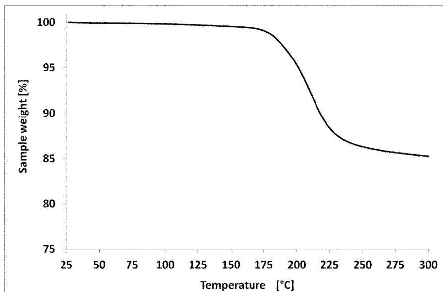
Figure 31: TGA scan of form Fumarate-NF1 (5 K/min)
