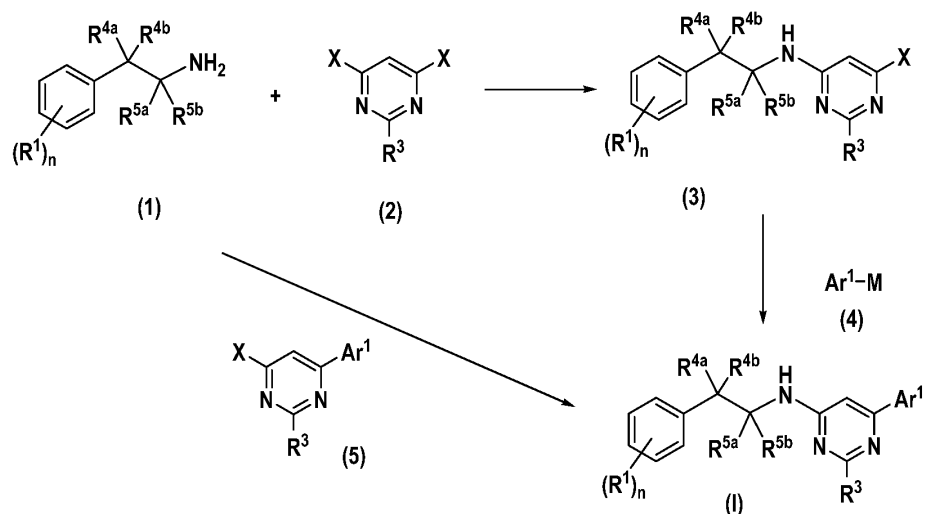
Scheme 1: General preparations of compounds of formula (I)
