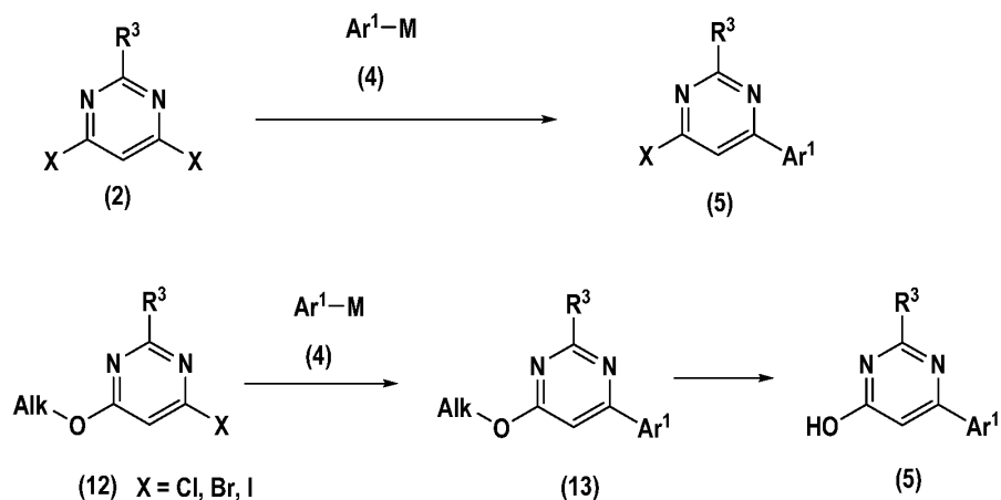
10 Scheme 3. Preparations of pyrimidines (5)
