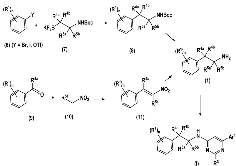
Scheme 2. Preparations of substituted \beta -aminoethyl aromatics (1)
