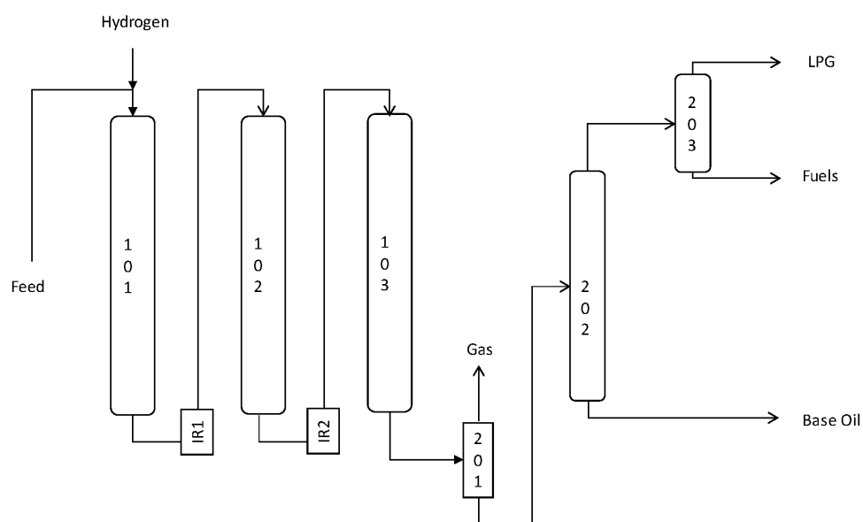
Figure 2 Simplified Process Flow Scheme
