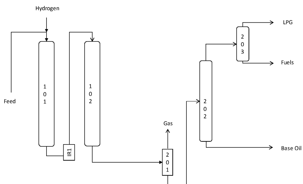
Figure 1 Simplified Process Flow Scheme
