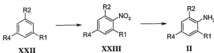
Scheme 10.
