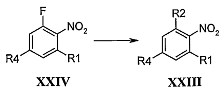
Scheme 11.
