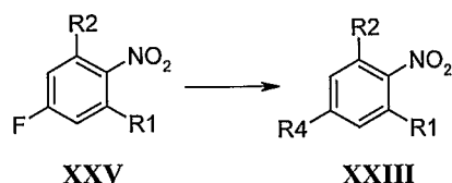
Scheme 12.
