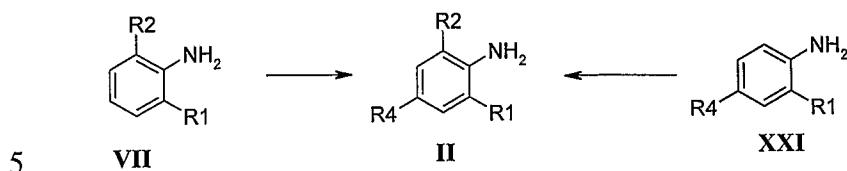
Scheme 9.
