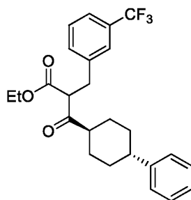
(IIIa)
