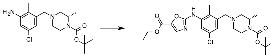
Scheme 9.10
