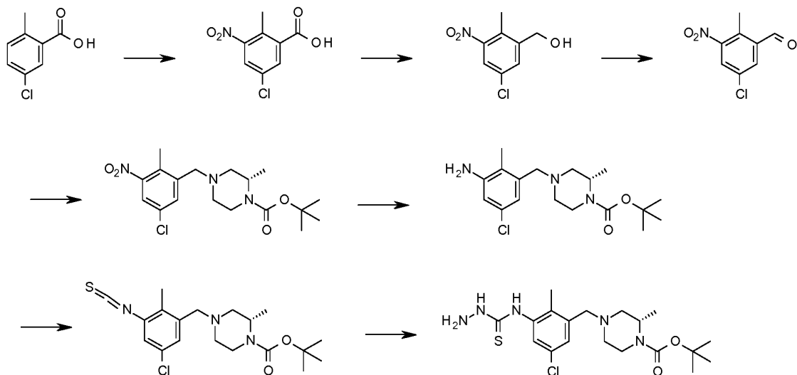
Scheme 9.1
