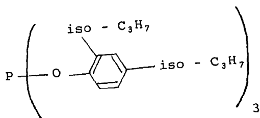
Exemplary Compound (2)-3
