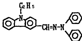
Exemplary Compound (5)-30
