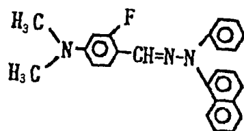
Exemplary Compound (5)-36
