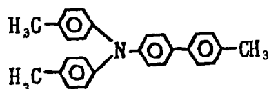
Exemplary Compound (4)-21
