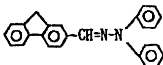
Exemplary Compound (5)-22
