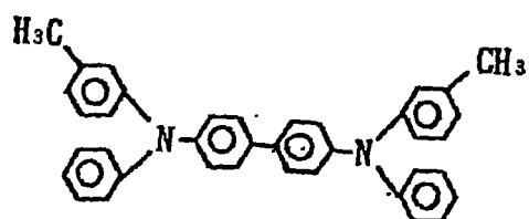
Exemplary Compound (4)-53
