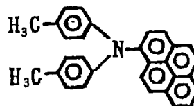
Exemplary Compound (4)-61
