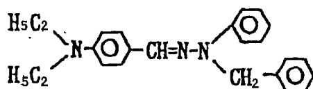
Exemplary Compound (5)-15
