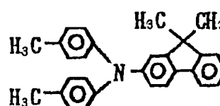
Exemplary Compound (4)-71
