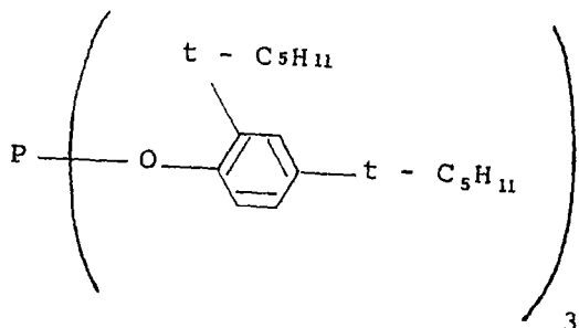
Exemplary Compound (2)-10
