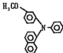
Exemplary Compound (4)-11
