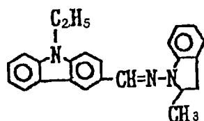
Exemplary Compound (5)-26
