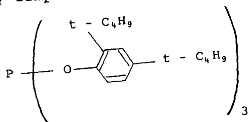
Exemplary Compound (2)-5
