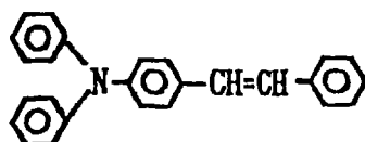
Exemplary Compound (3)-28
