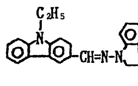
Exemplary Compound (5)-23
