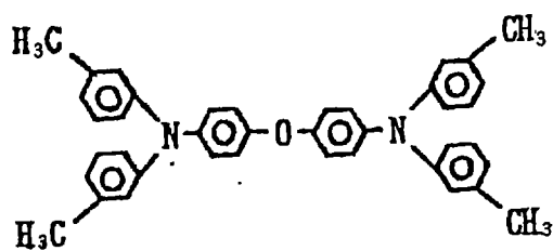
Exemplary Compound (4)-63
