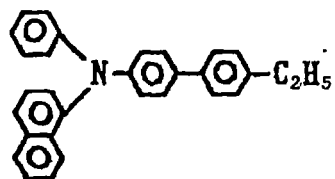
Exemplary Compound (4)-32
