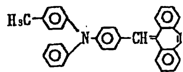
Exemplary Compound (3)-6
