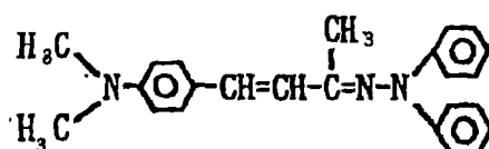
Exemplary Compound (5)-11
