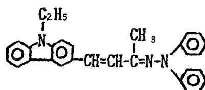
Exemplary Compound (5)-40
