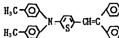
Exemplary Compound (3)-33
