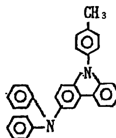
Exemplary Compound (4)-41
