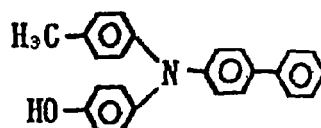
Exemplary Compound (4)-31
