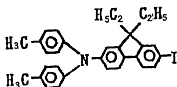
Exemplary Compound (4)-60
