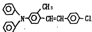
Exemplary Compound (3)-19
