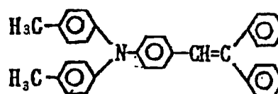
Exemplary Compound (3)-24
