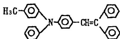
Exemplary Compound (3)-7
