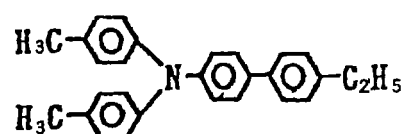
Exemplary Compound (4)-4
