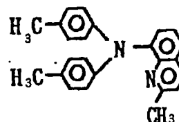
Exemplary Compound (4)-12
