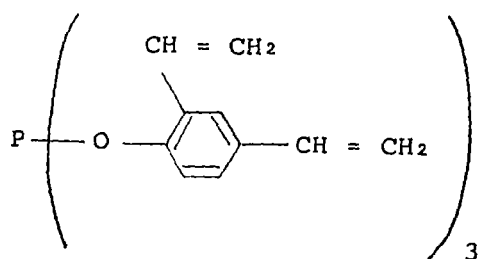
Exemplary Compound (2)-9
