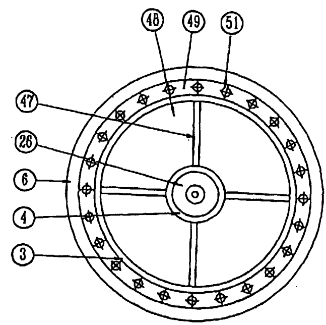
FIGURE-7 (REAR VIEW)
