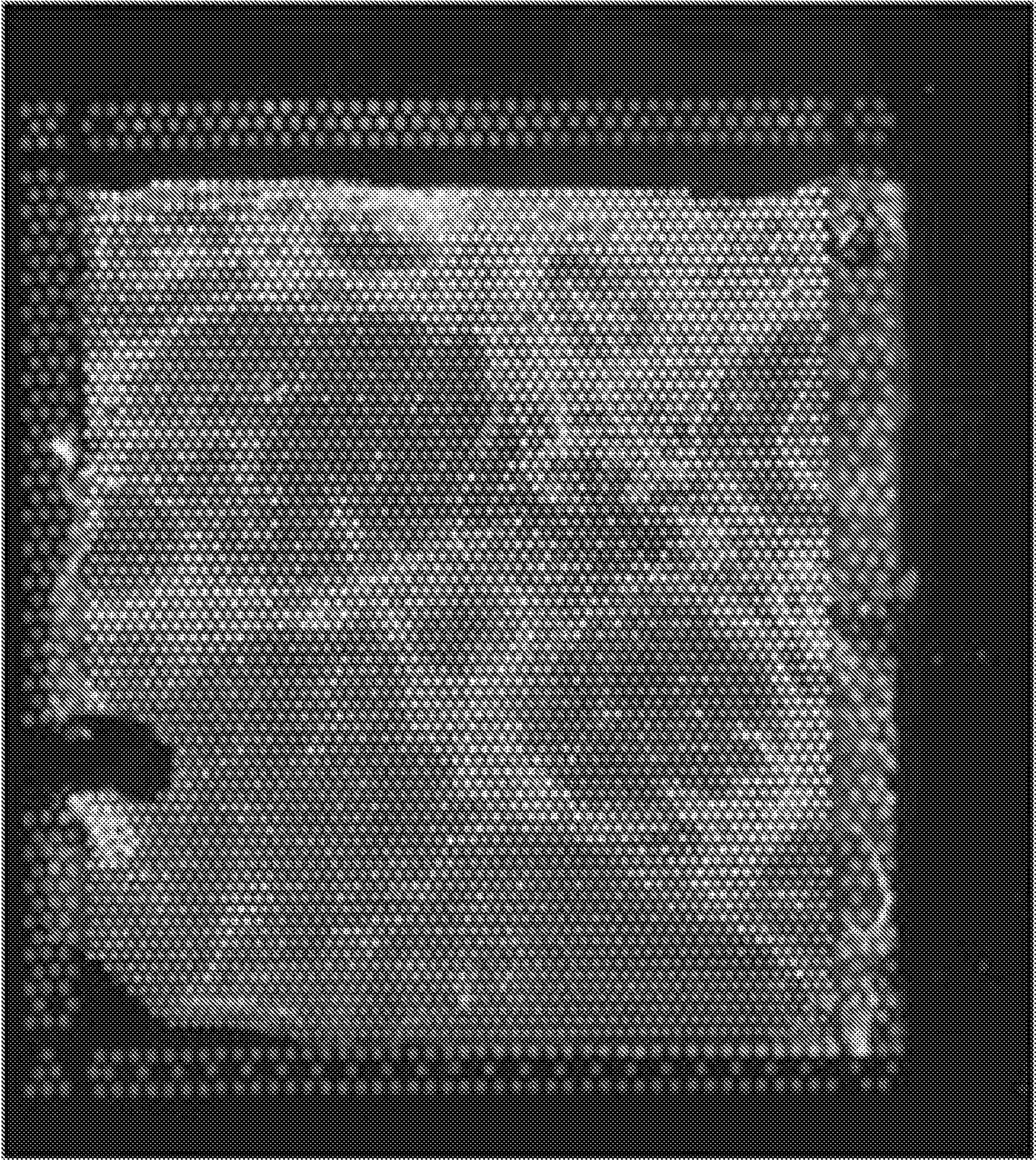
FIG. 16C: CD3 Protein Quantification
