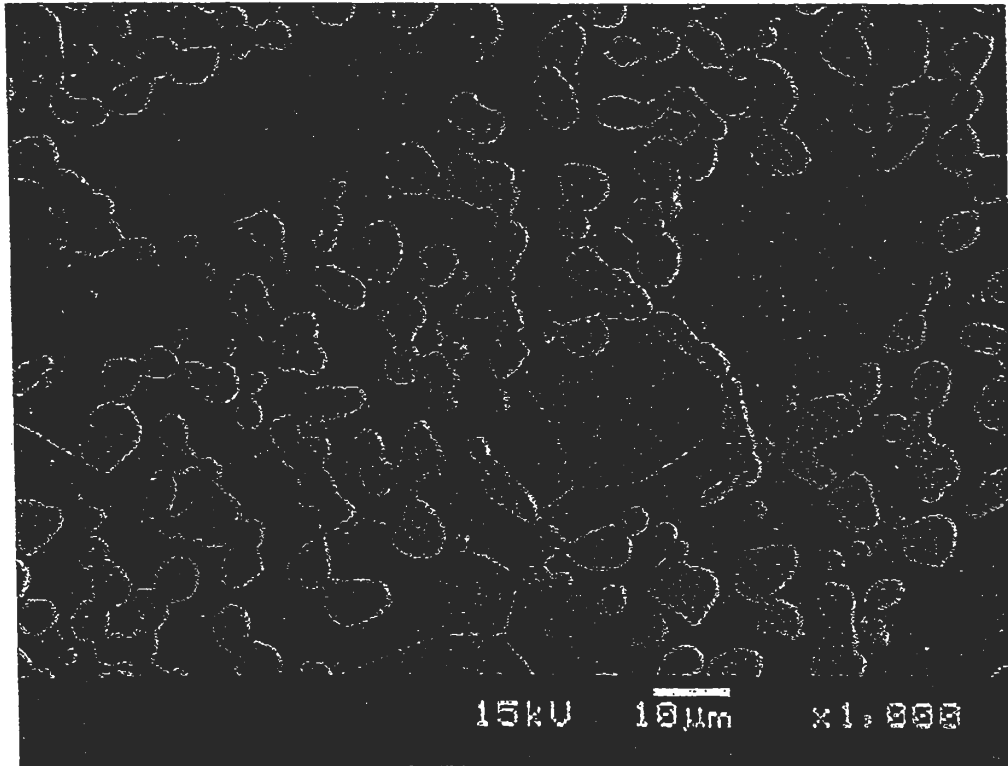
Figure 17. SEM secondary electron image of the as-cast Fe-(30.6 at. %)Co-(12.8 at. %)B alloy.
