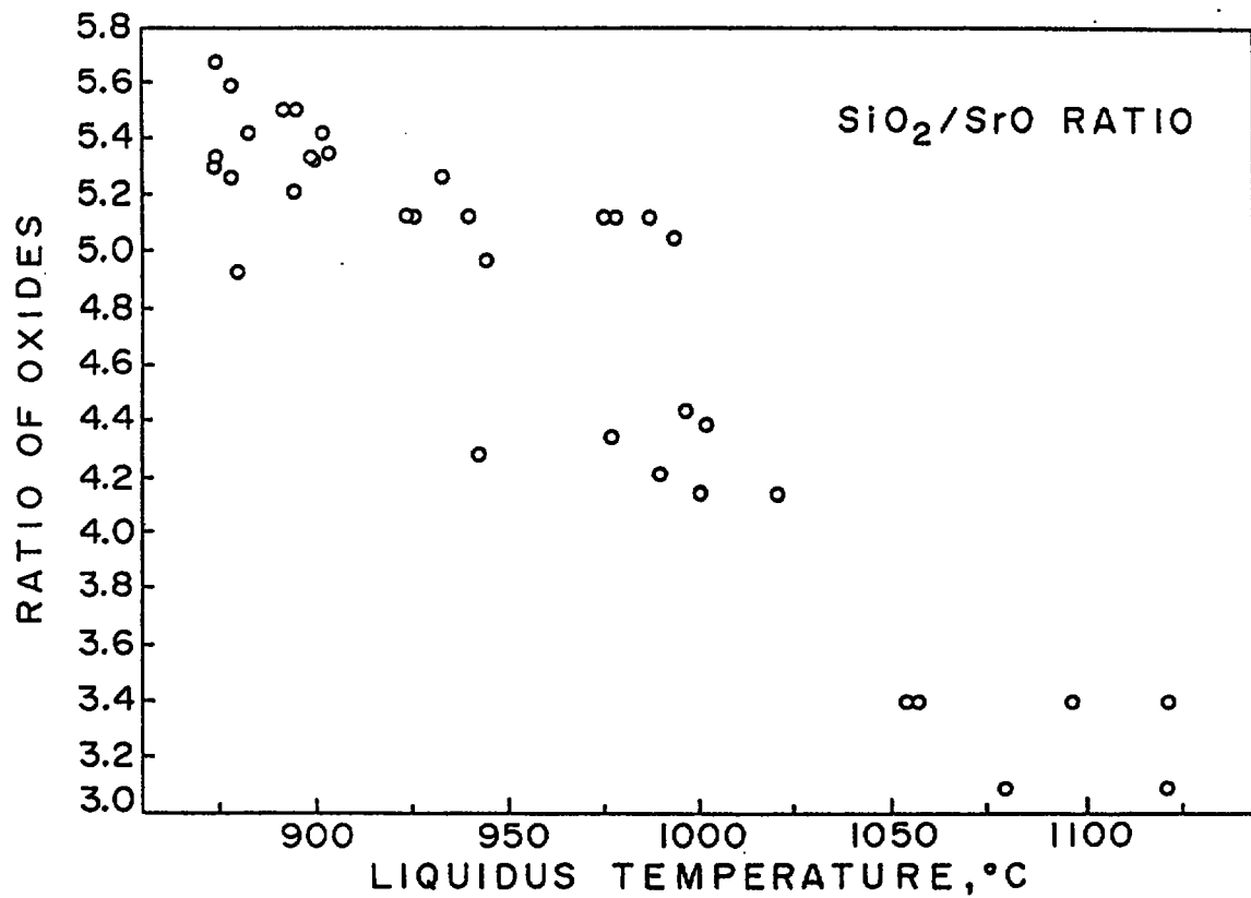
FIG.5-INCREASE \text{SiO}_2/\text{SrO} RATIO LOWERS LIQUIDUS
