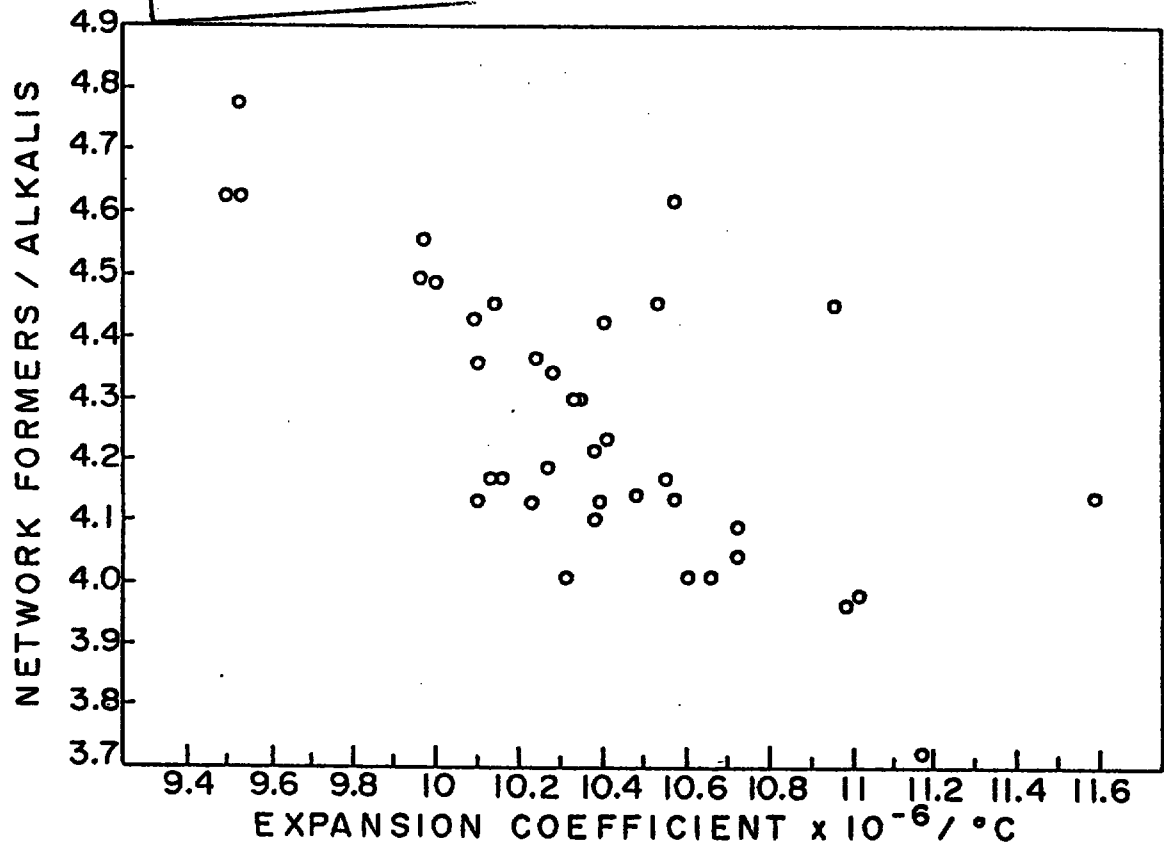
FIG.1-LOWER NETWORK /ALKALI RAISES EXPANSION
