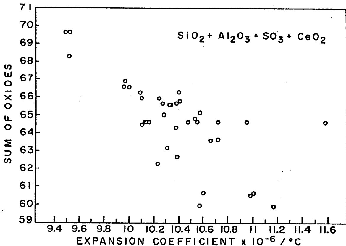
FIG.2 - DECREASES NETWORK RAISES EXPANSION
