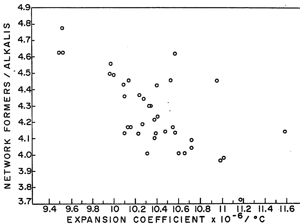
FIG.1 - LOWER NETWORK / ALKALI RAISES EXPANSION
