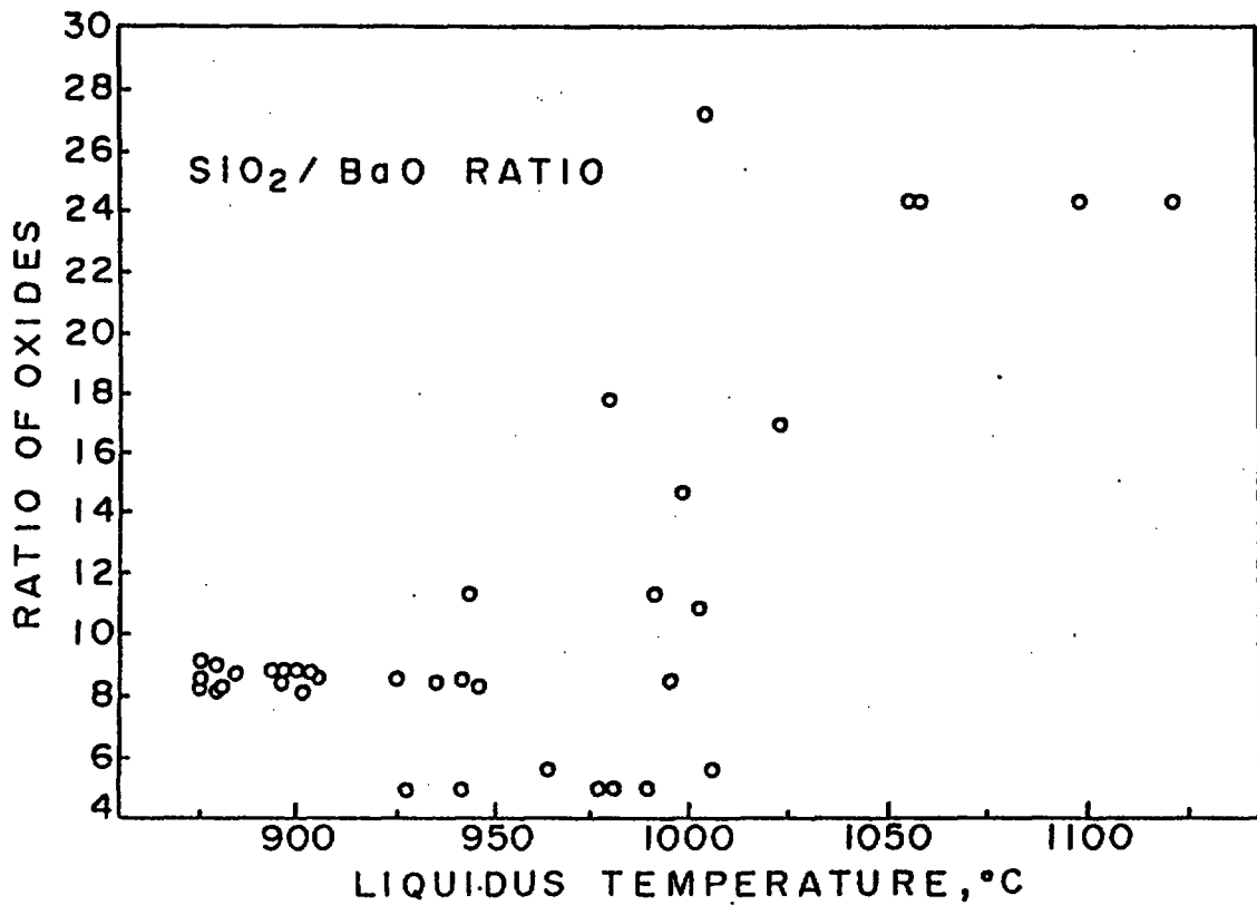
FIG.6- \text{SiO}_2/\text{BaO} RATIO BELOW 15; LOW LIQUIDUS
