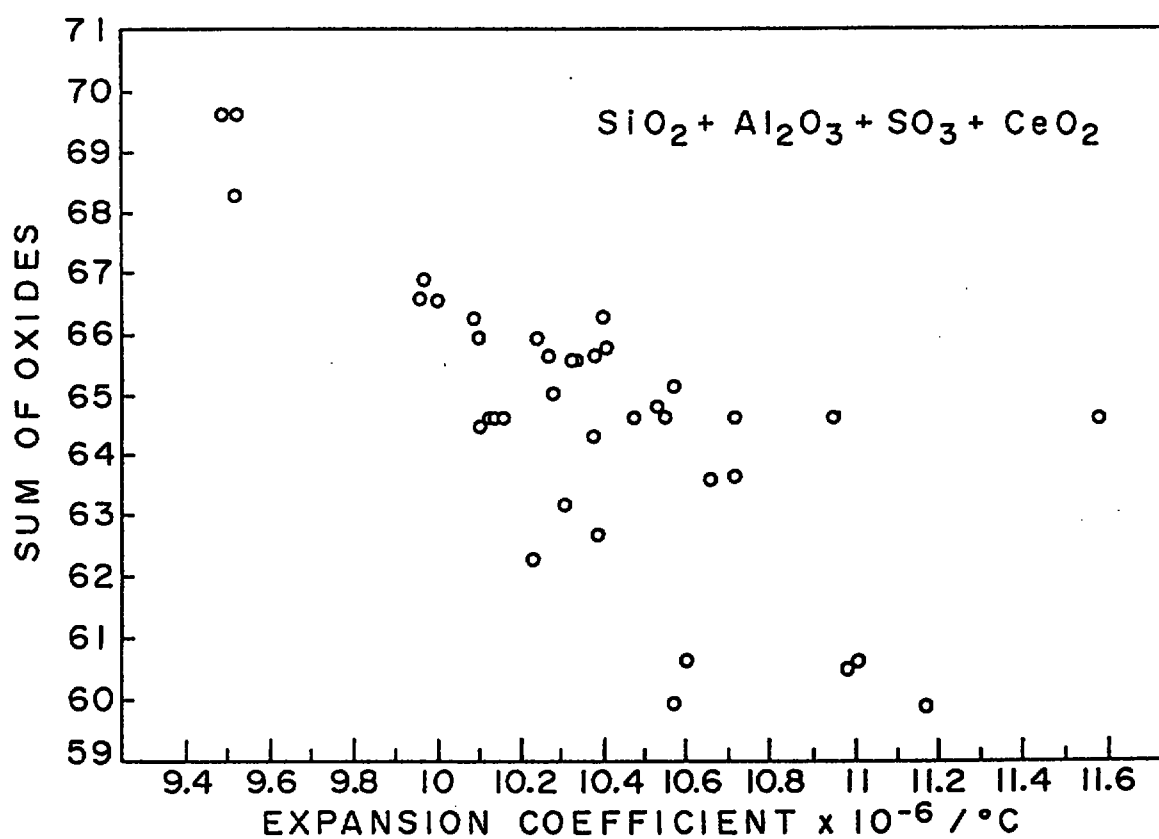
FIG.2 - DECREASES NETWORK RAISES EXPANSION
