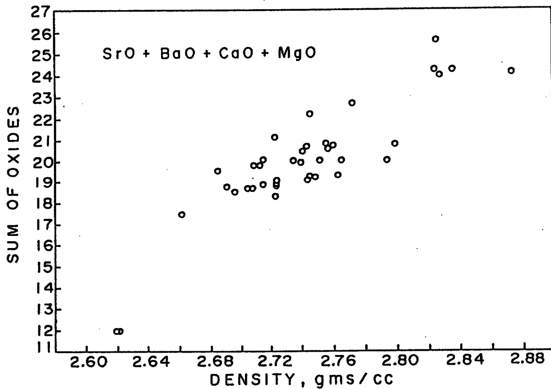
FIG.7-INCREASE ALKALINE EARTH'S RAISES DENSITY
