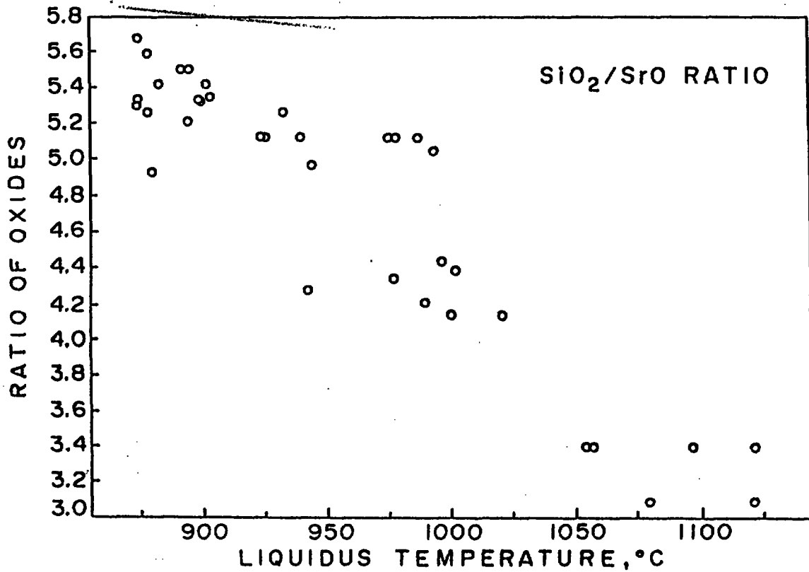
FIG.5-INCREASE \text{SiO}_2/\text{SrO} RATIO LOWERS LIQUIDUS
