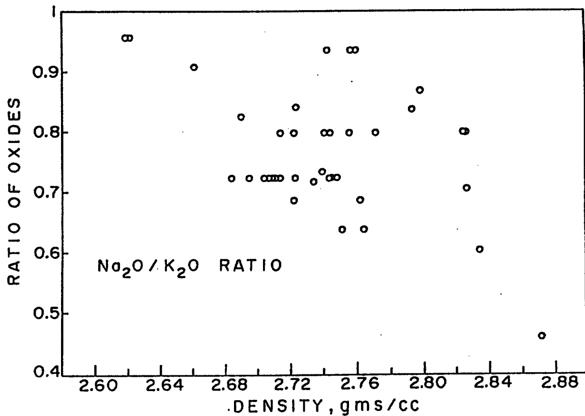
FIG.8-DECREASE Na 2 O/K 2 O RATIO RAISES DENSITY
