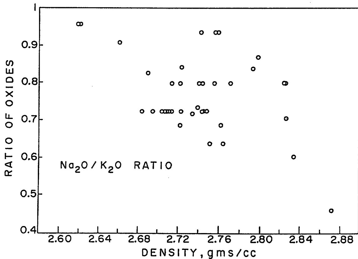
FIG.8-DECREASE \text{Na}_2\text{O}/\text{K}_2\text{O} RATIO RAISES DENSITY
