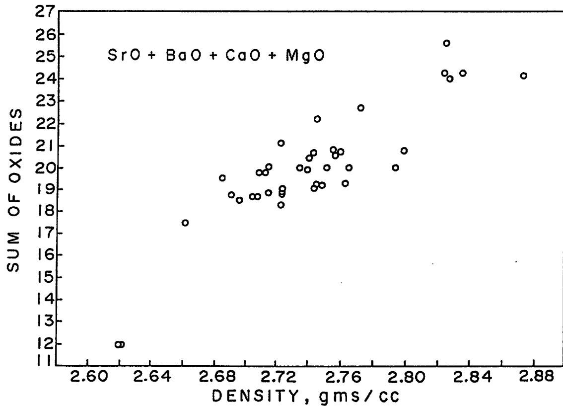
FIG.7-INCREASE ALKALINE EARTHS RAISES DENSITY
