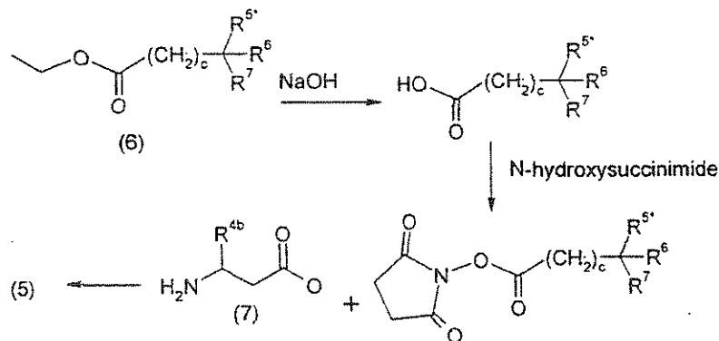
5 Compound (5) is formed by converting the ester compound (6) to the acid with a base, converting the acid to the dioxopyrrolidinyl ester with N-hydroxysuccinimide, then converting the dioxopyrrolidinyl ester with compound (7) to form compound (5). Compound (5) may have one or more R 4b substituents on the carbon atoms in the -(CH 2 ) b - and/or -(CH 2 ) c - portions.
