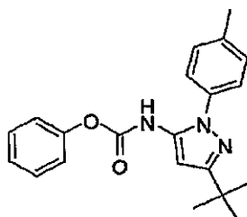
Phenyl 3-tert-butyl-1-p-tolyl-1H-pyrazol-5-ylcarbamate
