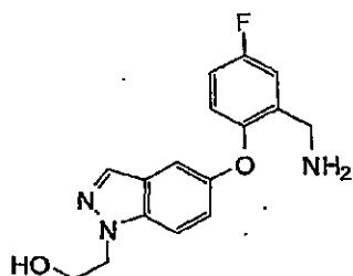
2-(5-(2-(Aminomethyl)-4-fluorophenoxy)-1H-indazol-1-yl)ethanol (79A)
