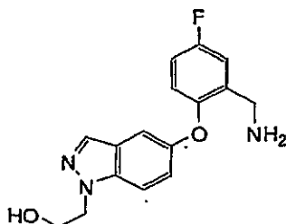
2-(5-(2-(aminomethyl)-4-fluorophenoxy)-1H-indazol-1-yl)ethanol (79A)
