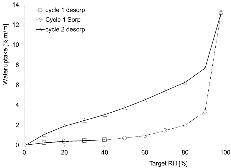
Fig. Form IIIId Water Vapour Sorption Isotherm (25 °C) of Form III
