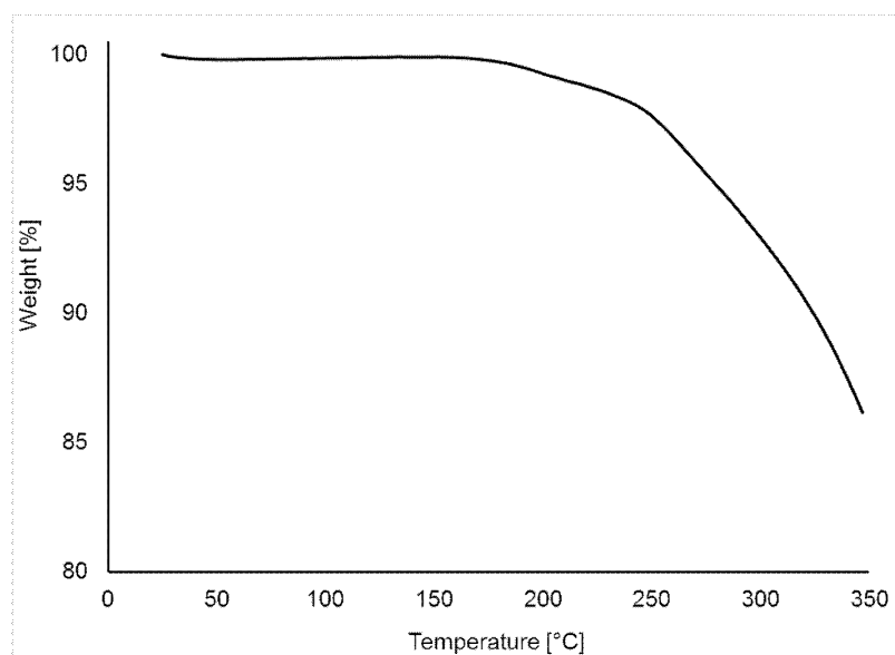
Fig. Form IIc TGA scan of Form II (5 K/min)
