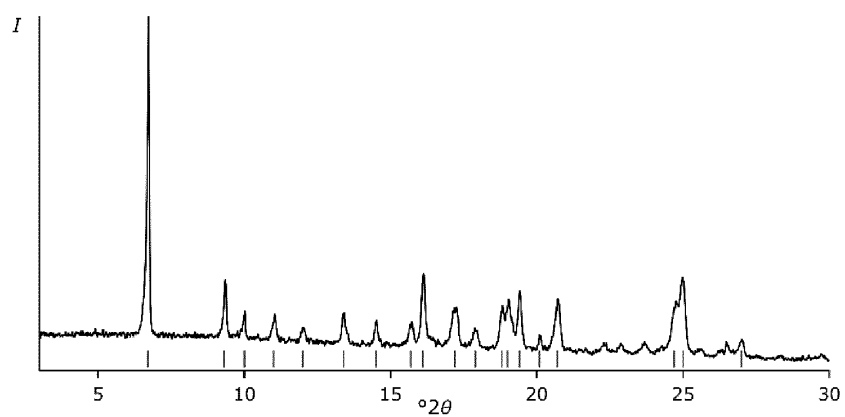
Fig. Form VIa Powder X-ray diffractogram of Form VI
