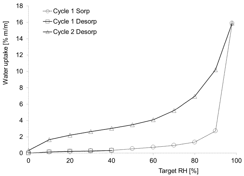
Fig. Form IVd Water Vapour Sorption Isotherm (25 °C) of Form IV
