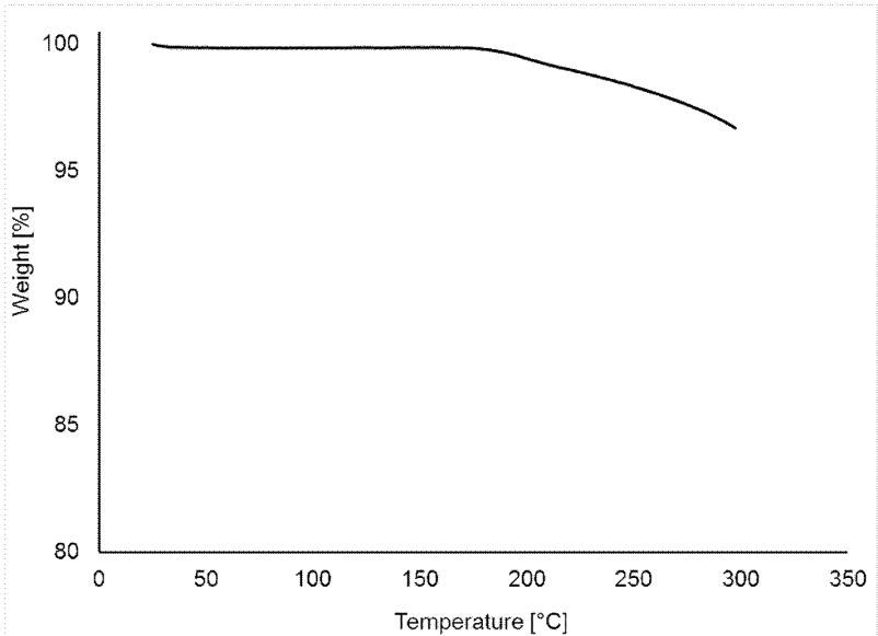
Fig. Form Vc TGA scan of Form V (5 K/min)
