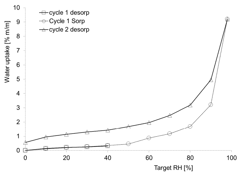
Fig. Form IIc Water Vapour Sorption Isotherm (25 °C) of Form II
