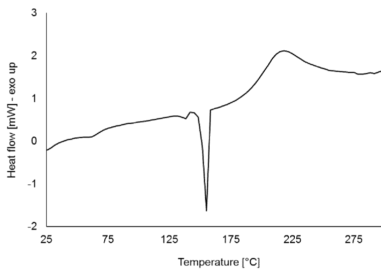
Fig. Form Ib DSC scan of Form I (5 K/min)
