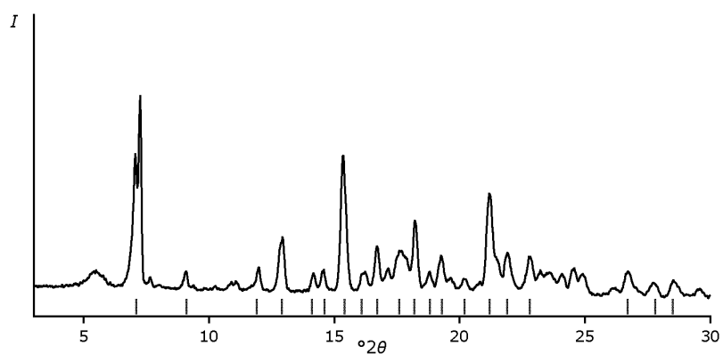
Fig. Form Ia Powder X-ray diffractogram of Form I
