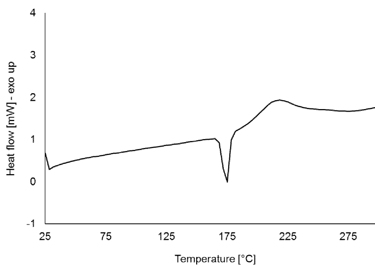
Fig. Form Vb DSC scan of Form V (5 K/min)
