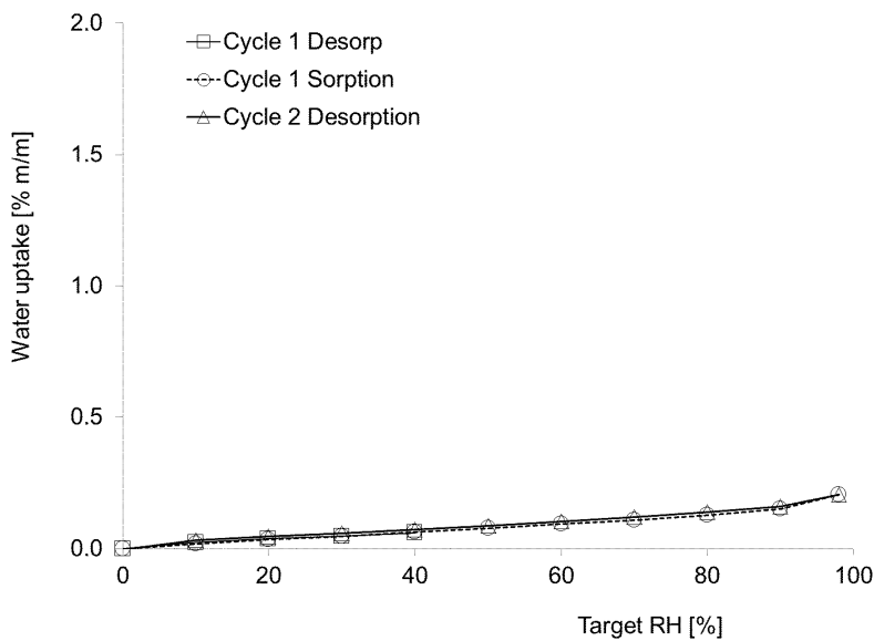
Fig. Form VIId Water Vapour Sorption Isotherm (25 °C) of Form VII
