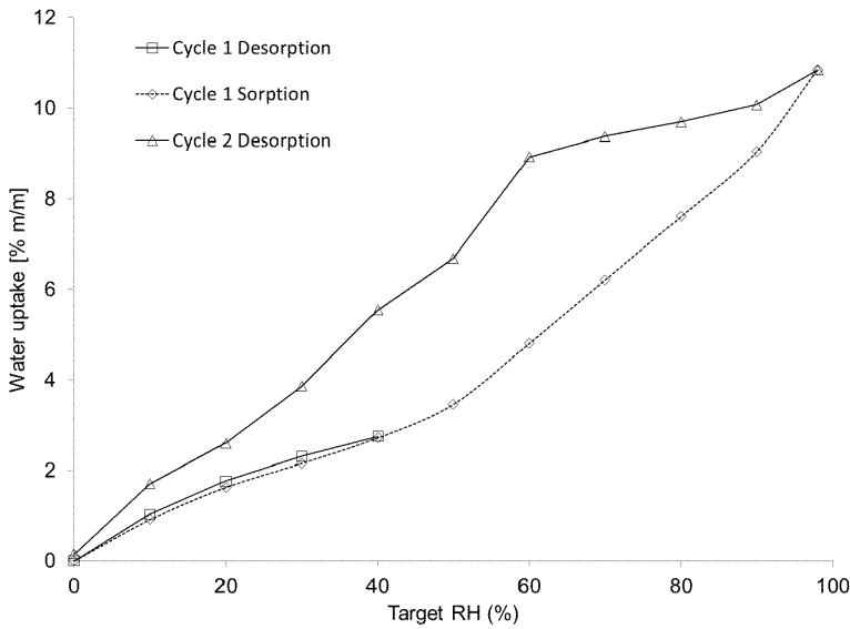
Fig. Tetraphosphated Water Vapour Sorption Isotherm (25 °C) of Tetraphosphate form
