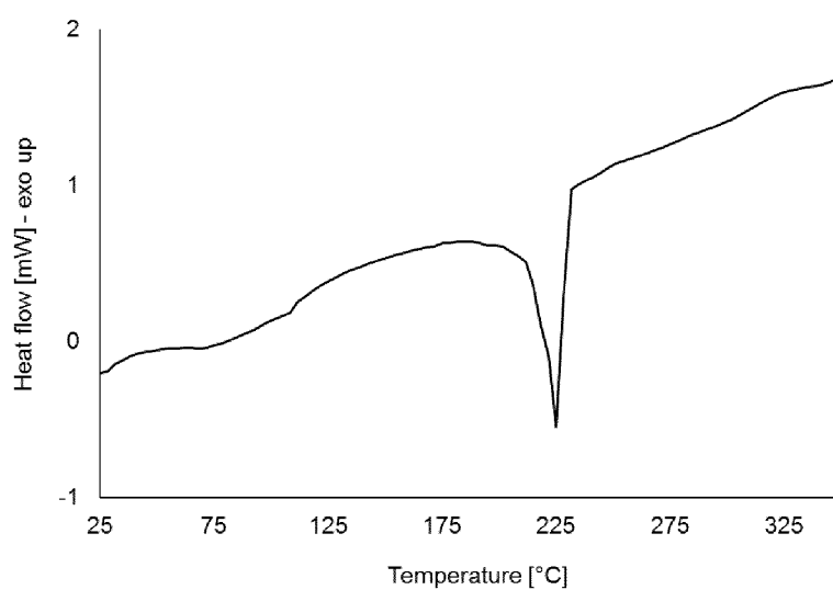
Fig. Tetraphosphateb DSC scan of Tetraphosphate form (5 K/min)
