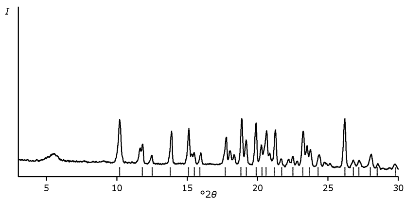
Fig. Form IIIa Powder X-ray diffractogram of Form III
