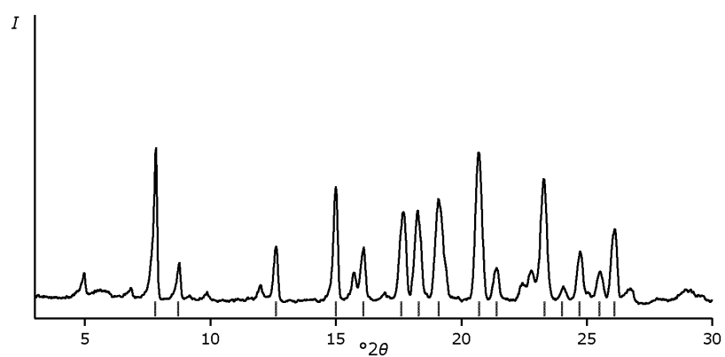
Fig. Form IIa Powder X-ray diffractogram of Form II
