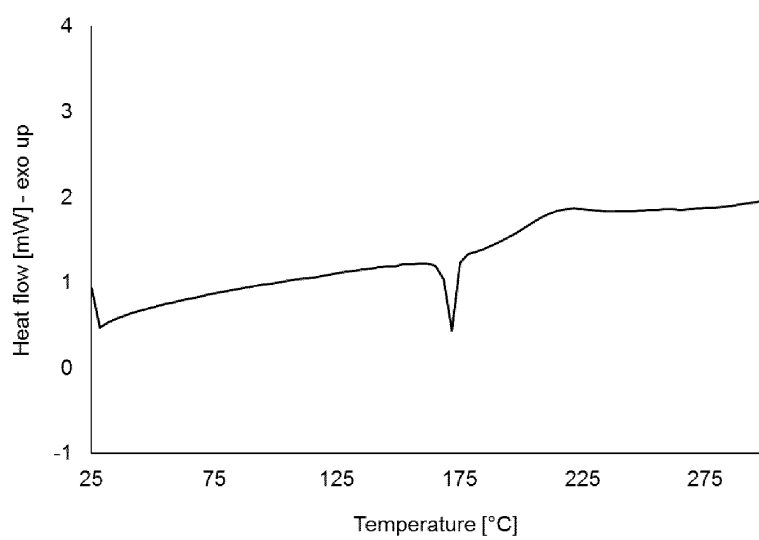
Fig. Form IVb DSC scan of Form IV (5 K/min)
