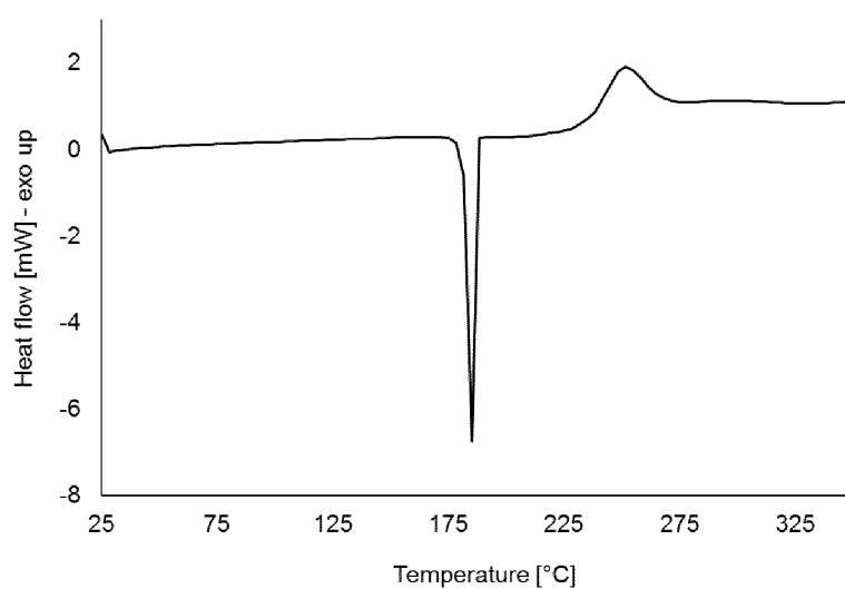
Fig. Form VIIb DSC scan of Form VII (5 K/min)
