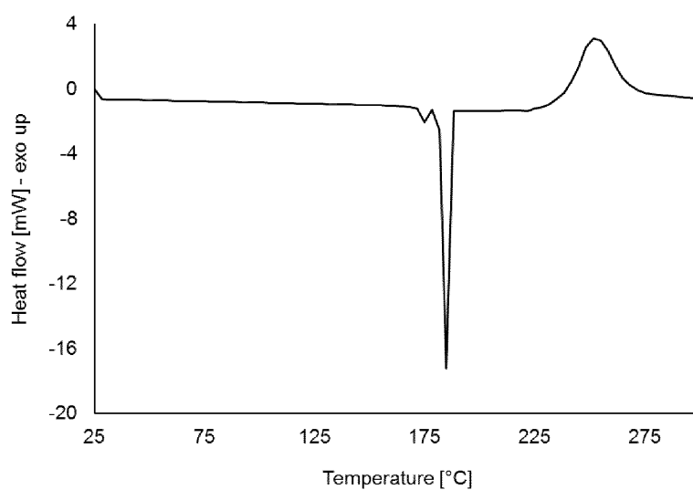
Fig. Form VIb DSC scan of Form VI (5 K/min)
