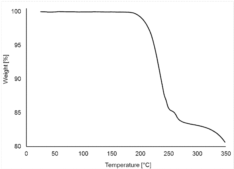
Fig. Form VIIc TGA scan of Form VII (5 K/min)
