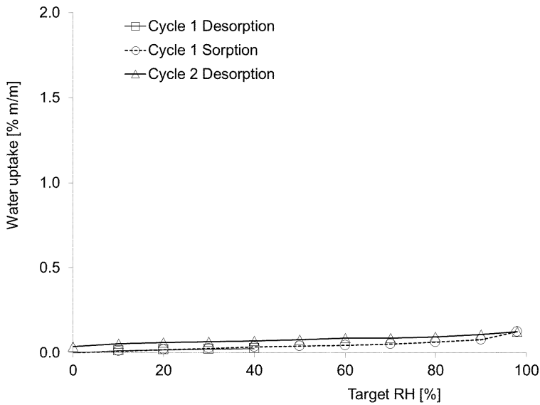
Fig. Form VIId Water Vapour Sorption Isotherm (25 °C) of Form VI
