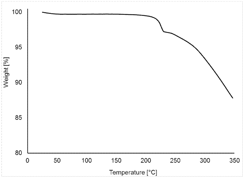
Fig. Form IIIc TGA scan of Form III (5 K/min)
