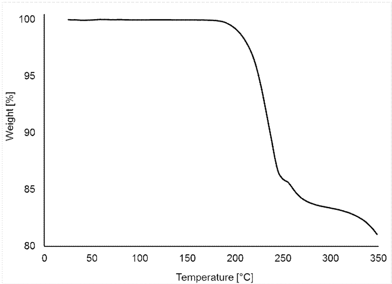
Fig. Form VIc TGA scan of Form VI (5 K/min)
