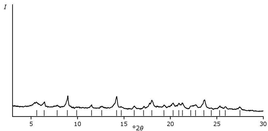
Fig. Tetraphosphatea Powder X-ray diffractogram of tetraphosphate form
