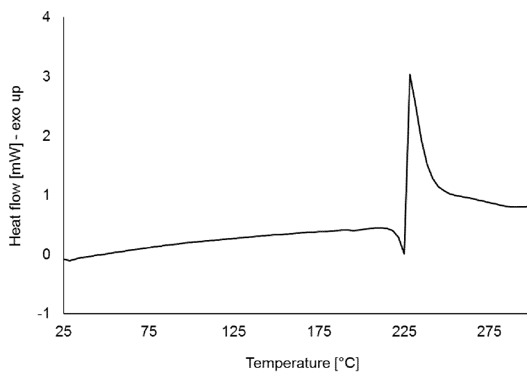
Fig. Form IIIb DSC scan of Form III (5 K/min)
