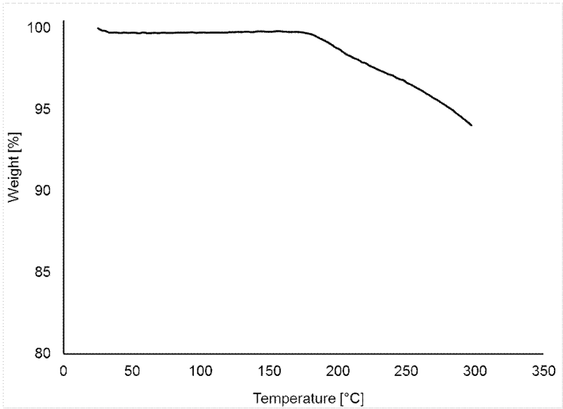
Fig. Form IVc TGA scan of Form IV (5 K/min)
