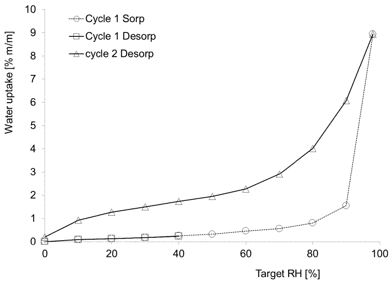
Fig. Form Vd Water Vapour Sorption Isotherm (25 °C) of Form V
