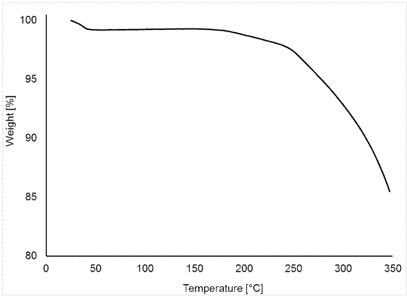
Fig. Form I c TGA scan of Form I (5 K/min)
