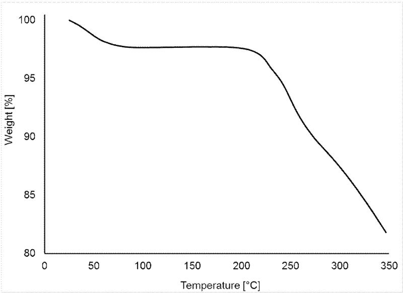
Fig. Tetraphosphate TGA scan of Tetraphosphate form (5 K/min)
