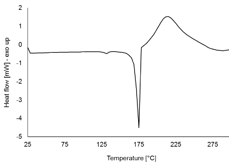
Fig. Form IIb DSC scan of Form II (5 K/min)
