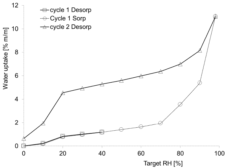
Fig. Form I d Water Vapour Sorption Isotherm (25 °C) of Form I
