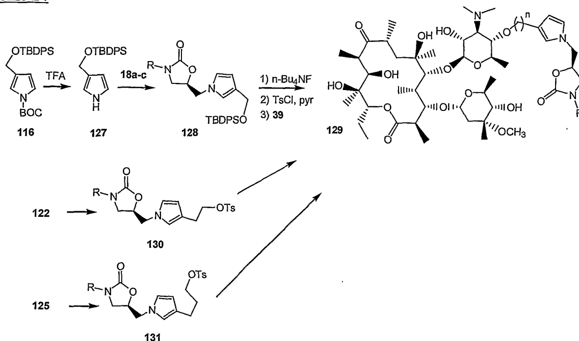
Scheme 24
