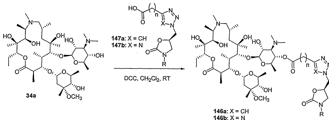
Scheme 30
