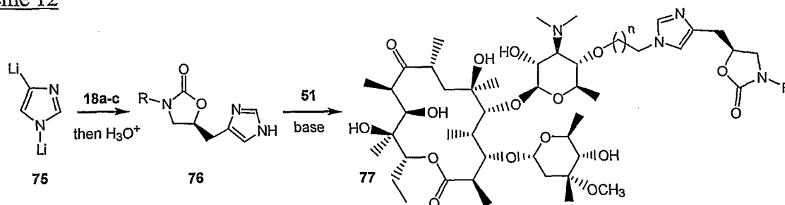
Scheme 12
