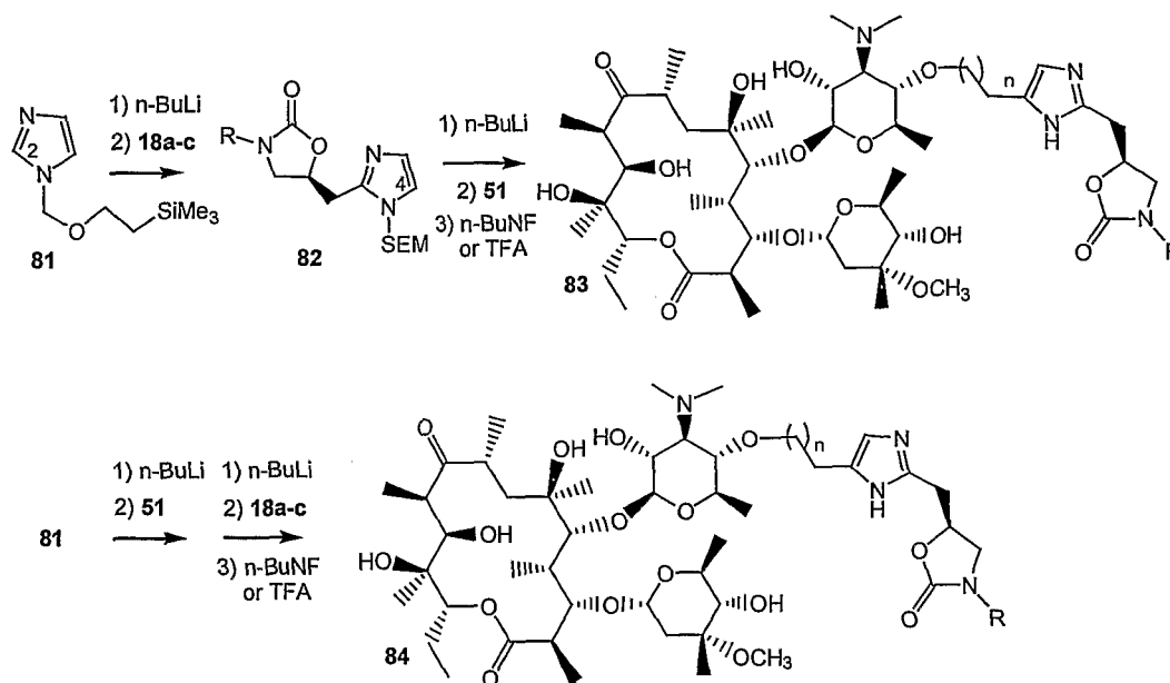
Scheme 14
