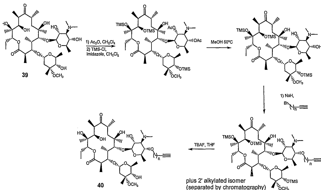
Scheme 3b
