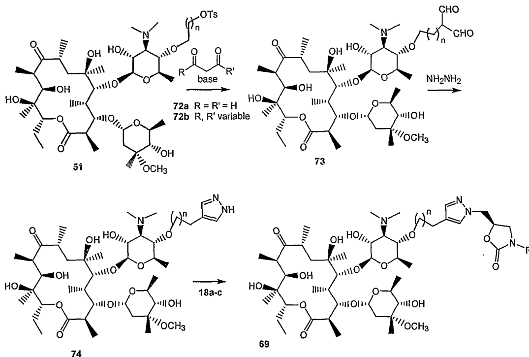
Scheme 11
