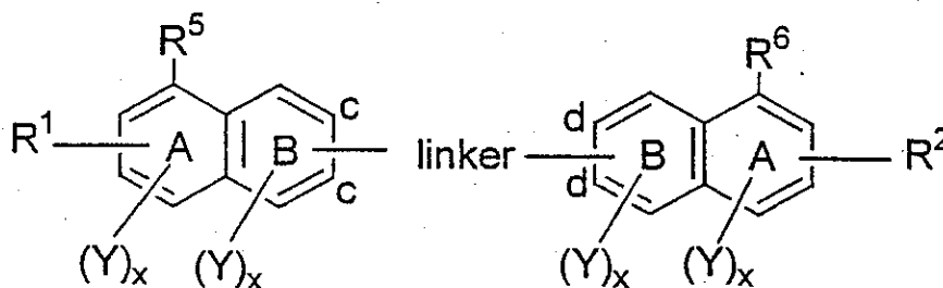
Formula I
