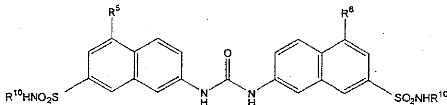
Formula III
