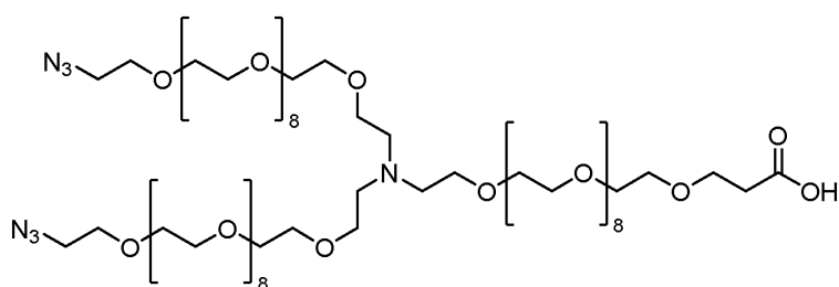
N-(acid-PEG 10 )-N-bis(PEG 10 -azide);
