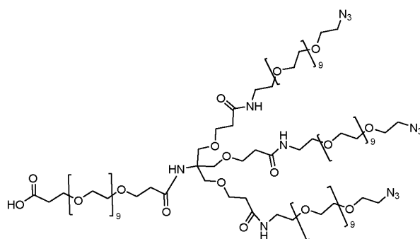
Methane-N-(PEG 10 -acid)-Tri(MeOPr-amide-PEG 10 -azide); and
