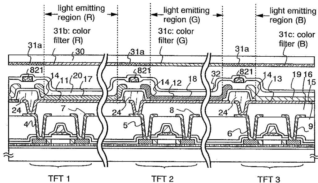
FIG. 10A sectional view of A-A'
