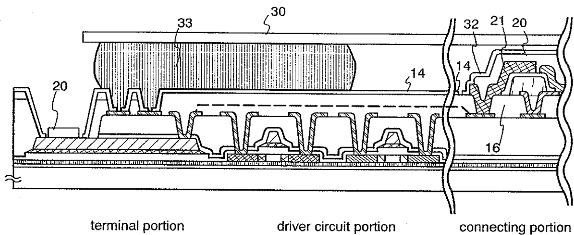
FIG. 1C sectional view of C-C'
