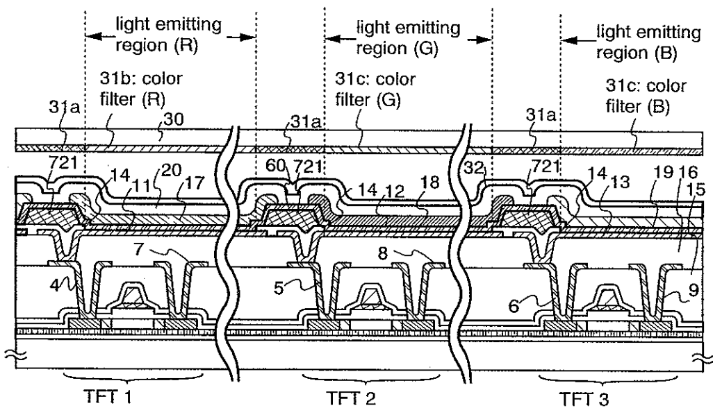
FIG. 9A sectional view of A-A'
