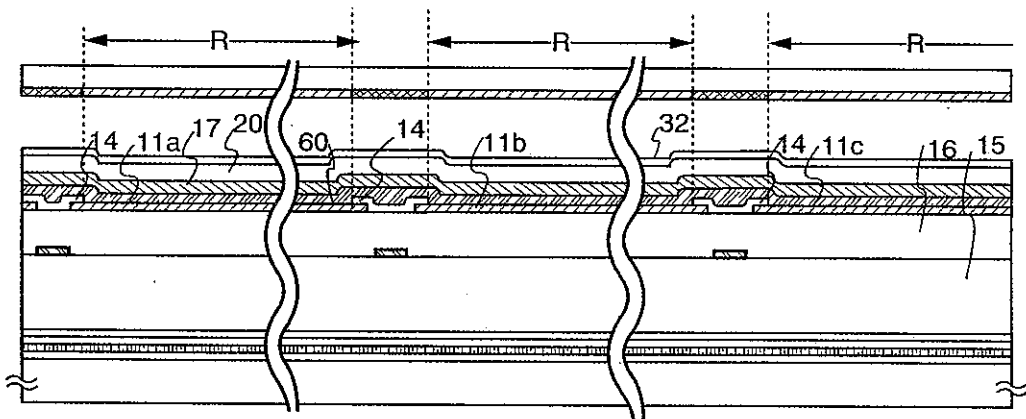
FIG. 9B sectional view of B-B'
