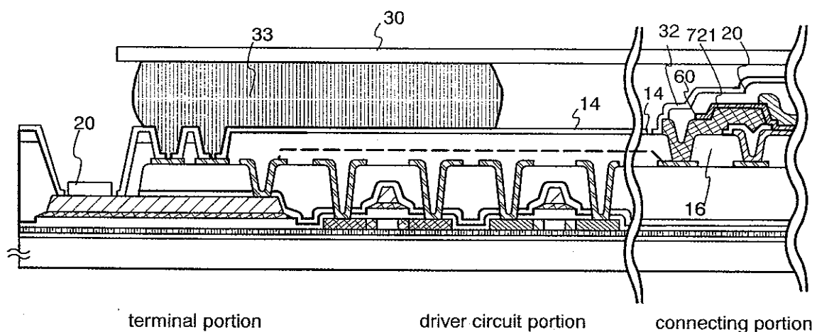
FIG. 9C sectional view of C-C'
