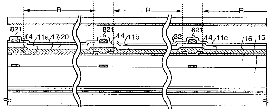
FIG. 10B sectional view of B-B'
