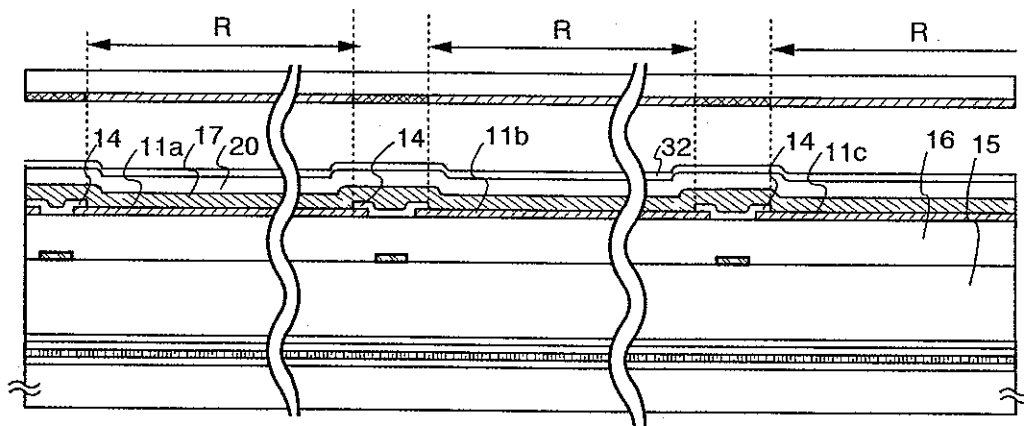
FIG. 1B sectional view of B-B'
