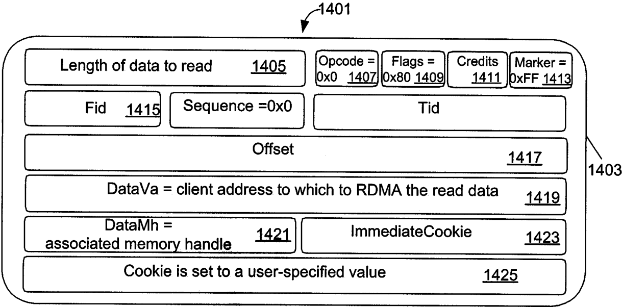
CLIENT READ MESSAGE (NO POLLING)
