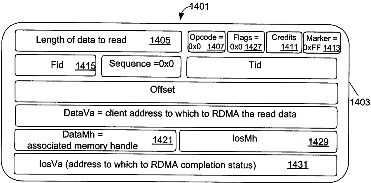
CLIENT READ MESSAGE (POLLING)
