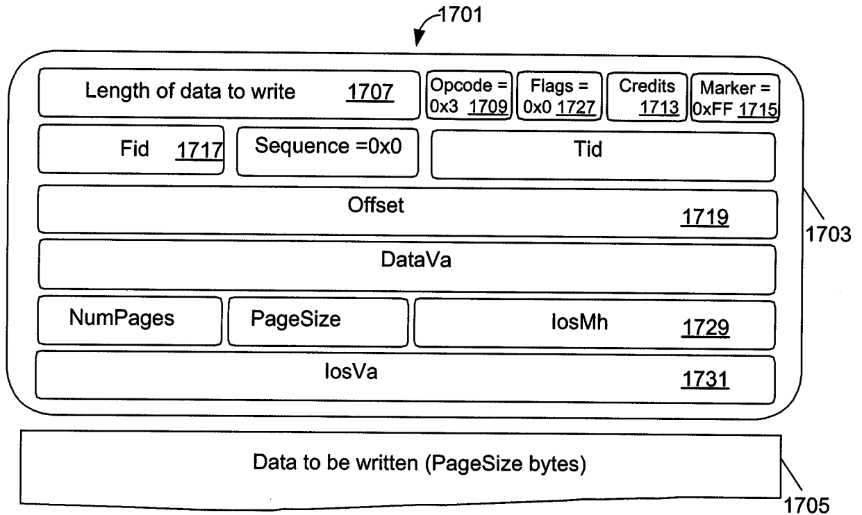
CLIENT VECWRITE MESSAGE, COLLAPSED (POLLING)
