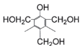
TriML-35XL
