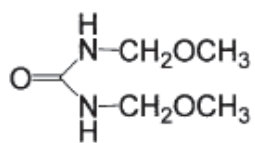
NIKALAC MX-290
