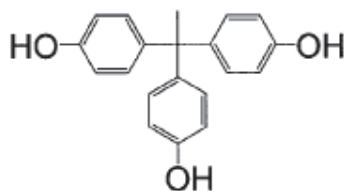
TrisP-HAP
