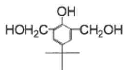
DML-PTBP
