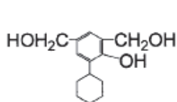
DML-OCHP
