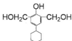
DML-PCHP
