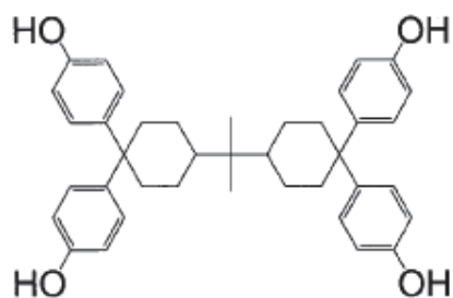
TekP-4HPBA
