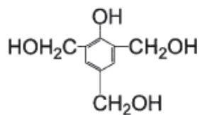
TriML-P
