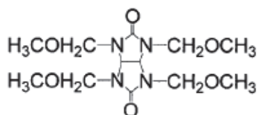
NIKALAC MX-270
