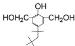
DML-POP
