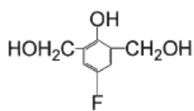
DML-PFP
