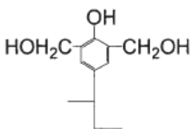
DML-PSBP
