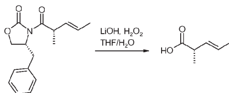
Compound 27c
