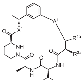
Formula (I-d)
