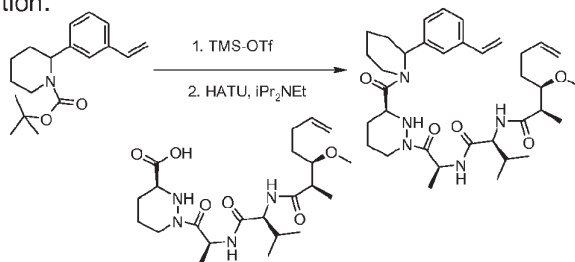
Compound 28g
