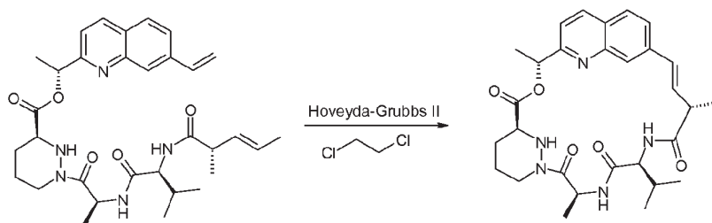
Compound 27
