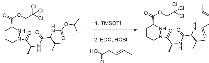
Compound 8c
