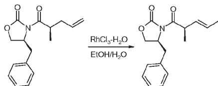
Compound 26a
