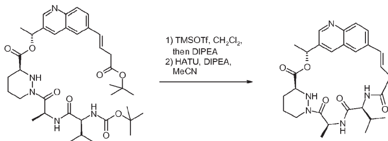
Compound 14
