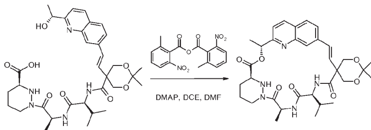
Compound 75
