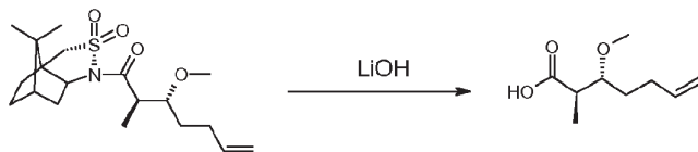
Compound 28d
