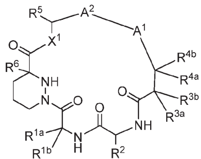
Formula I
