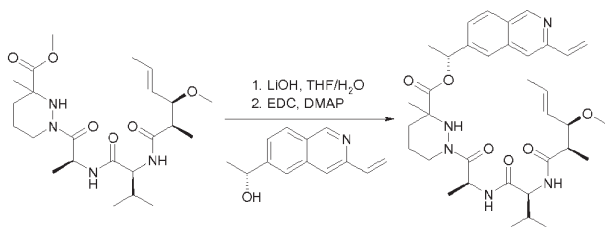
Compound 33g
