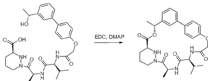
Compound 38
