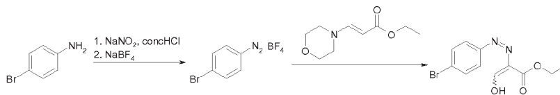
Compound 32b
