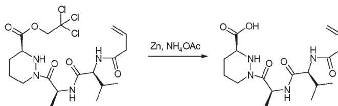
Compound 10b
