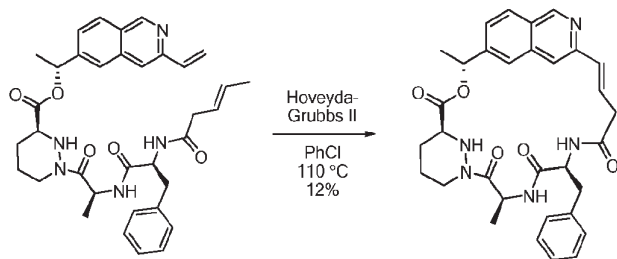
Compound 54
