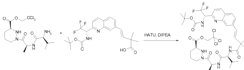
Compound 13d
