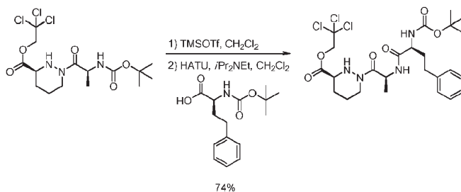
Compound 56a
