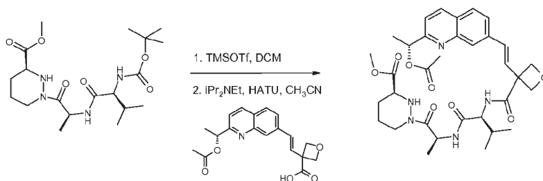
Compound 73e
