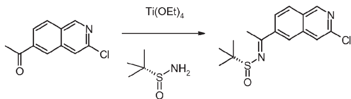
Compound 5c
