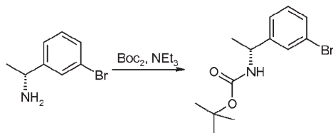
Compound 1g
