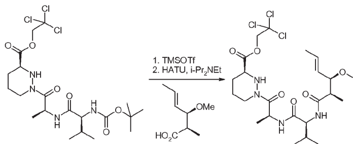
Compound 5j
