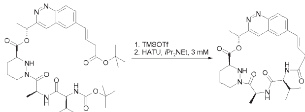
Compound 32
