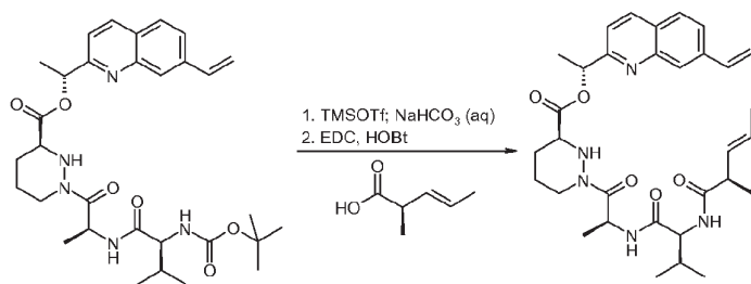
Compound 26e
