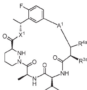
Formula (I-e)
