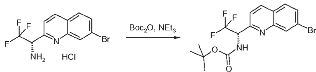
Compound 13a
