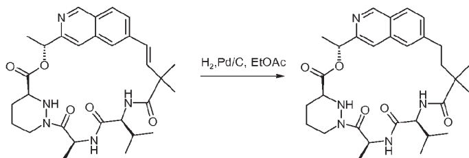
Compound 18
