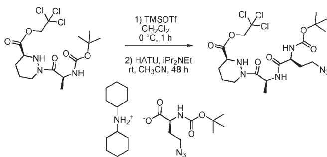
Compound 49a
