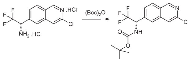
Compound 23g
