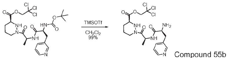
Compound 55b
