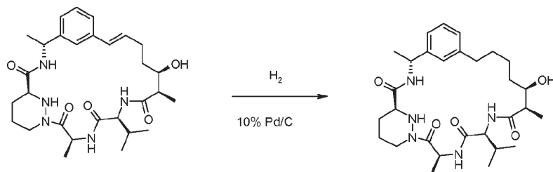
Compound 3
