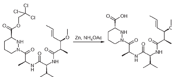
Compound 5k
