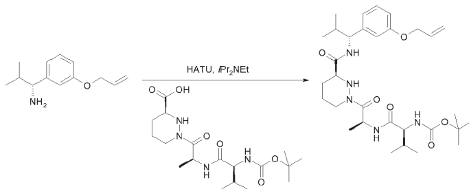
Compound 37d
