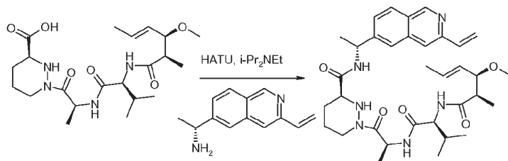
Compound 5I
