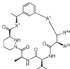
Formula (I-c)
