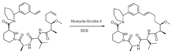
Compound 28
