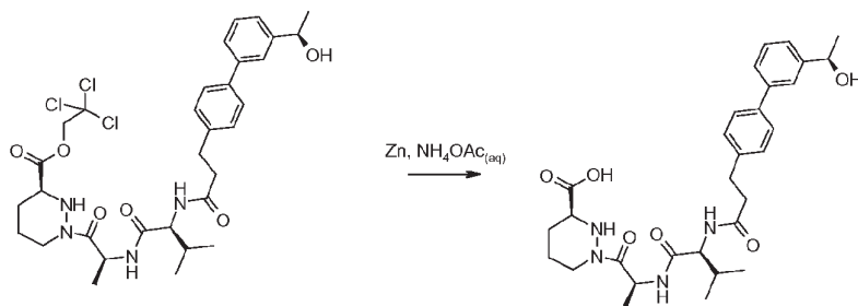
Compound 43d
