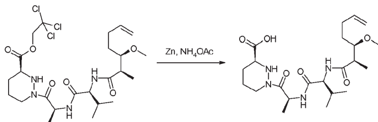
Compound 28f
