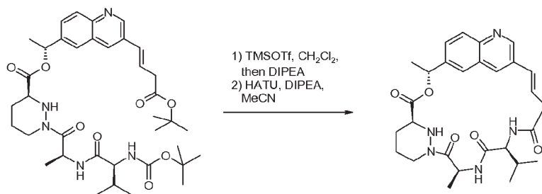
Compound 15
