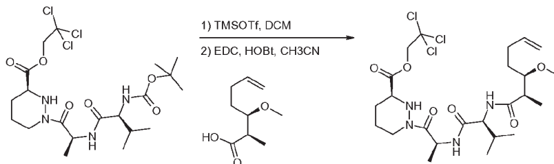
Compound 28e
