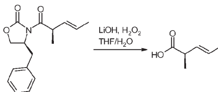
Compound 26b
