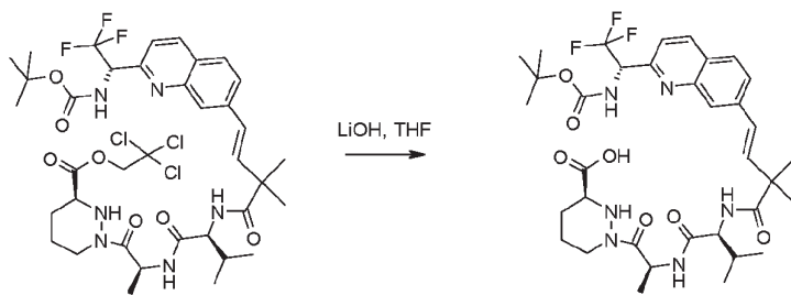
Compound 13e
