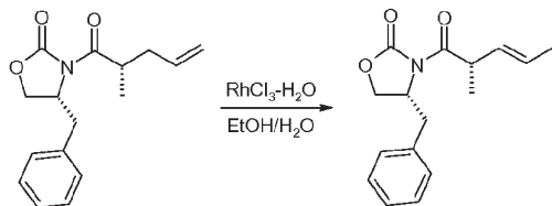
Compound 27b
