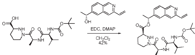
Compound 19a
