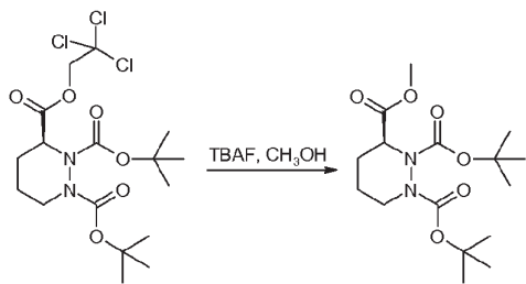
Compound 33a
