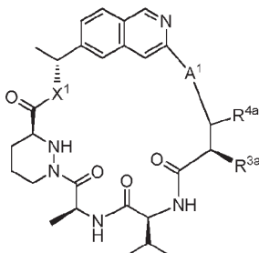
Formula (I-a)
