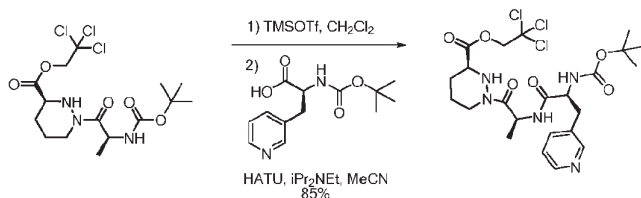
Compound 55a
