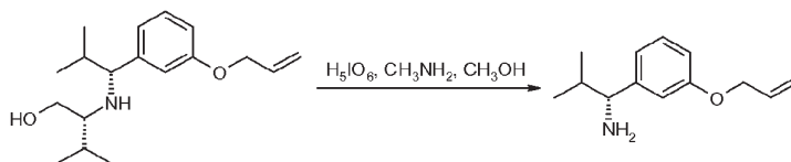
Compound 37c
