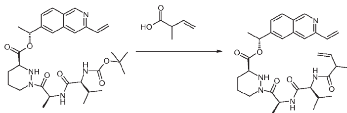
Compound 20a
