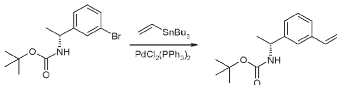
Compound 1h
