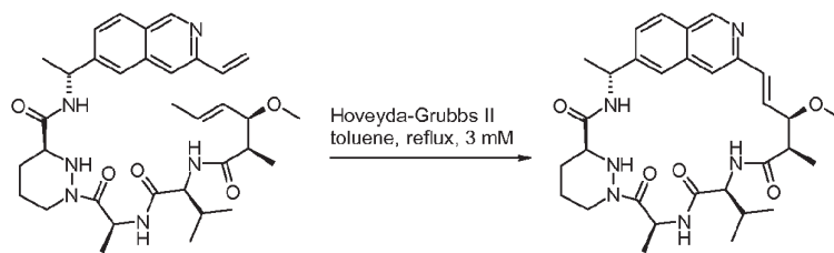
Compound 5
