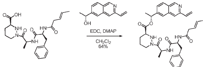
Compound 54d
