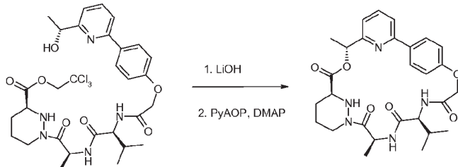
Compound 41
