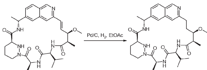
Compound 6
