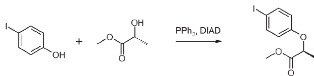
Compound 39a
