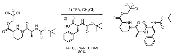
Compound 54a
