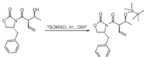
Compound 31a
