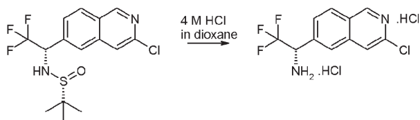
Compound 23f
