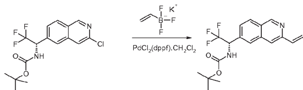
Compound 23h
