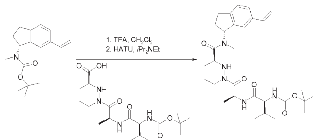
Compound 25d
