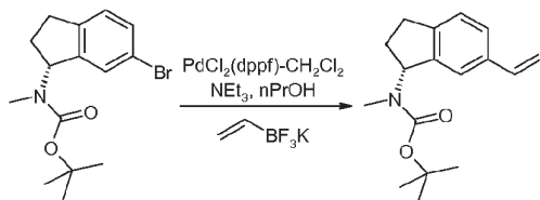
Compound 25c
