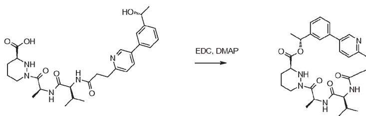
Compound 44
