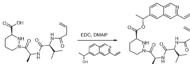
Compound 10c
