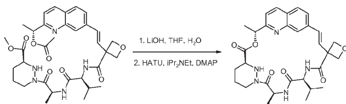
Compound 73
