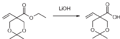
Compound 75e
