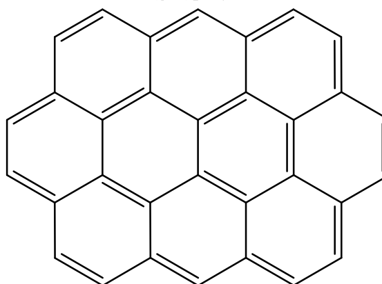
ovalene
