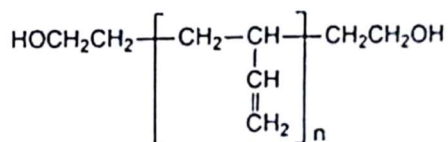
Structural Formula
