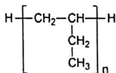
Structural Formula
