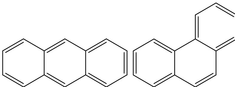
anthracene
