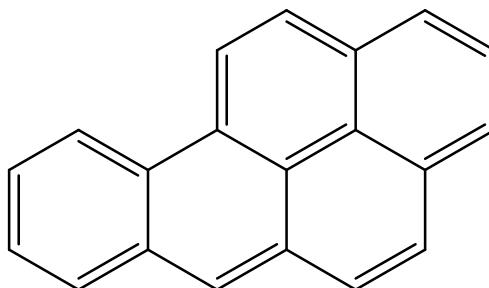
benzo(a)pyrene
