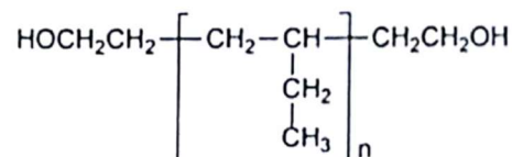
Structural Formula
