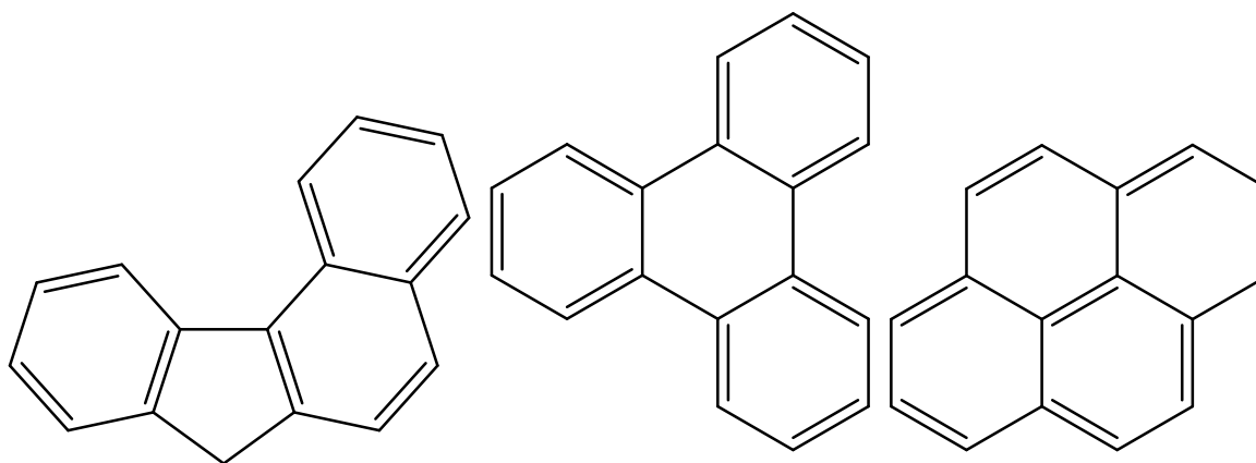
benzo(c)fluorene
