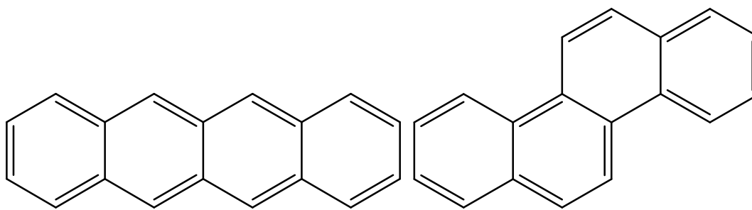
tetracene
