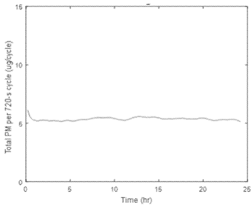
Baseline Fuel 3 + 200 ppmw inventive example 2
