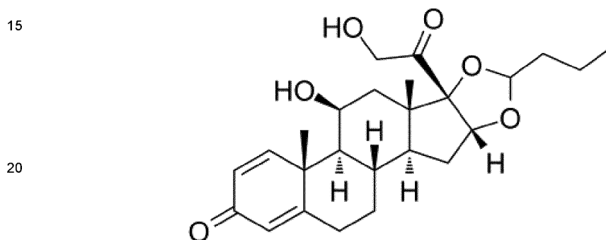
Formula (I)
