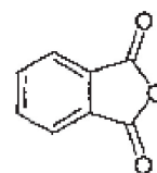
Phthalic anhydride (S9)
