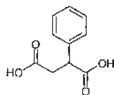
Phenylsuccinic acid (S8)
