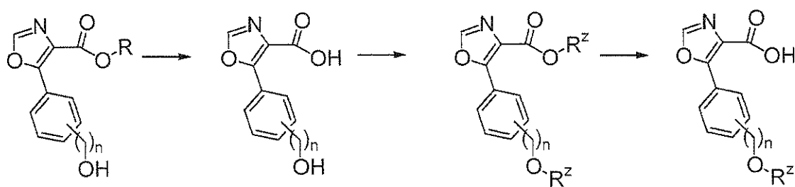
Scheme 4: Synthesis of (C_1-C_4) alkoxy- (C_1-C_2) alkyl substituted 5-phenyl-oxazole derivatives ( R^2 represents (C_1-C_4) alkyl and n represents 1 or 2).
