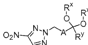
Structure 6
