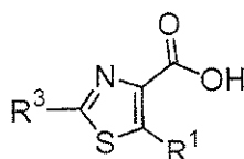
Structure 9
