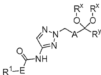
Structure 4
