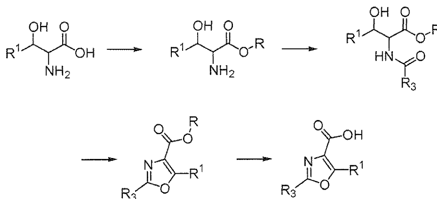
Scheme 3: Oxazole synthesis (4).
