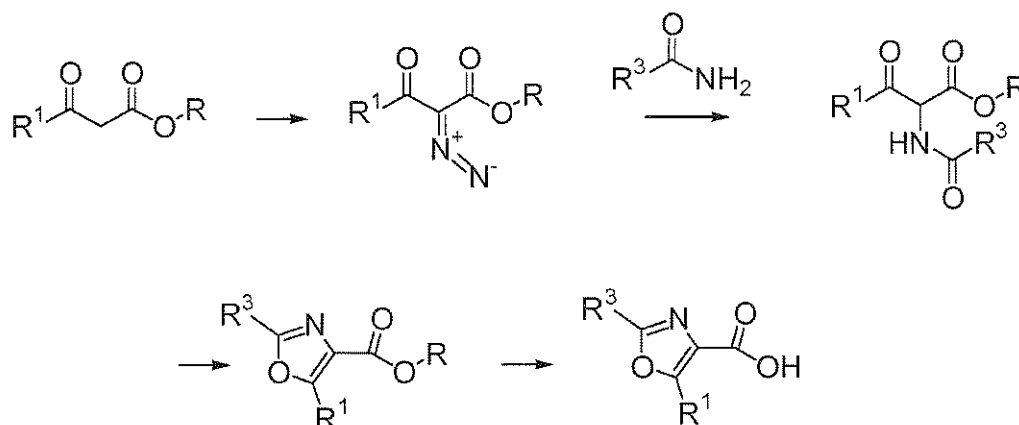
Scheme 2: Oxazole synthesis (2).
