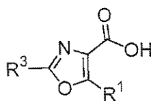
Structure 8
