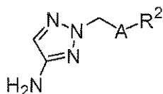
Structure 1
