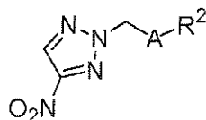
Structure 2
