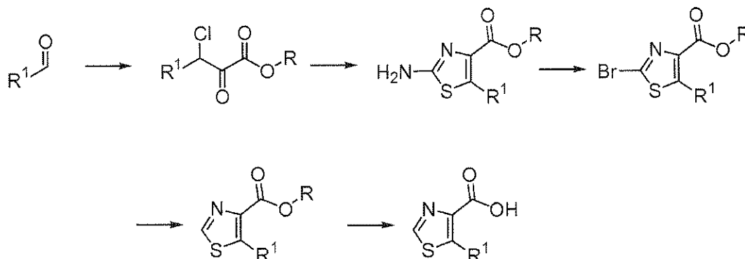
Scheme 8: Thiazole synthesis (2).
