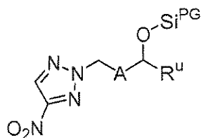
Structure 7
