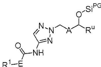
Structure 4c
