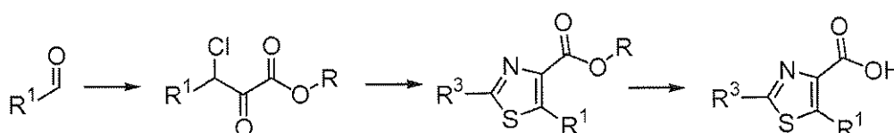
10 Scheme 7: Thiazole synthesis (1), wherein R 3 represents (C 1 -C 4 )alkyl or cyclopropyl.
