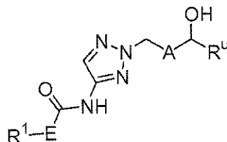
Structure 4b
