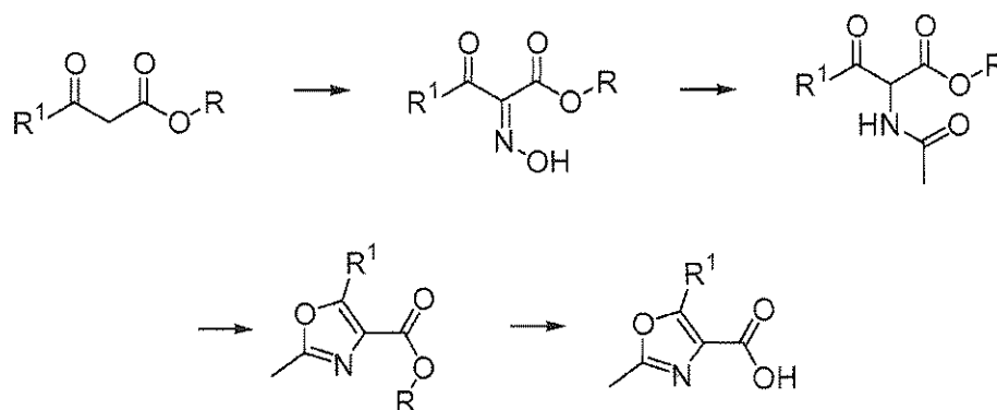
Scheme 1: Oxazole synthesis (1).
