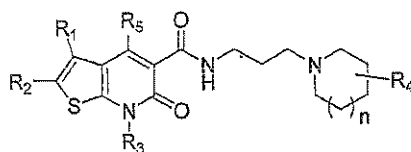
Thienopyridinone
