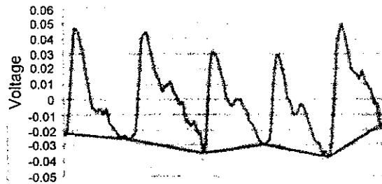
PPG waveform at pressure 299 mmHg
