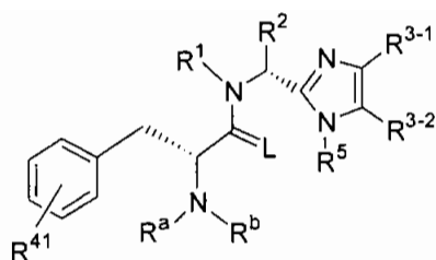
Formula (Ie)
