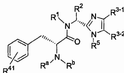
Formula (Ie)
