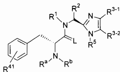
Formula (Id)
