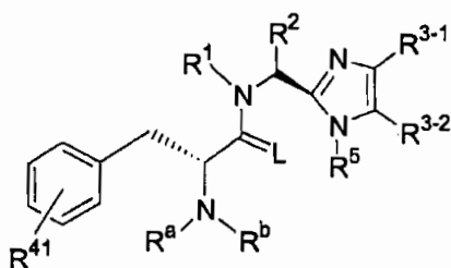
Formula (Id)
