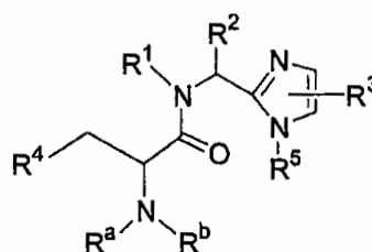
20 Formula (Ia)
