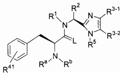
Formula (Ib)
