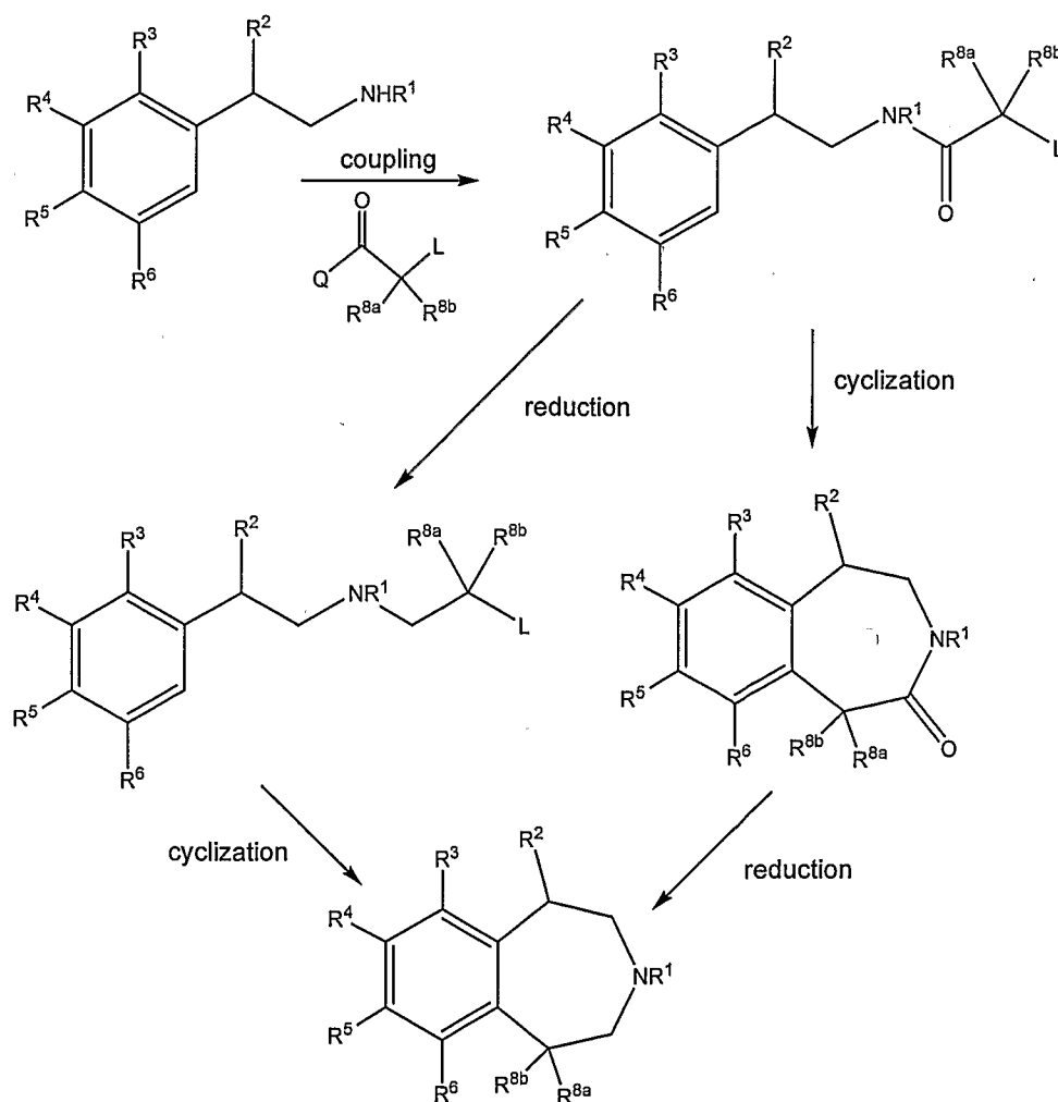
Scheme Ia
