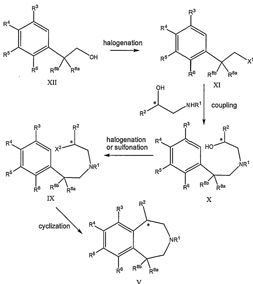
Scheme II
