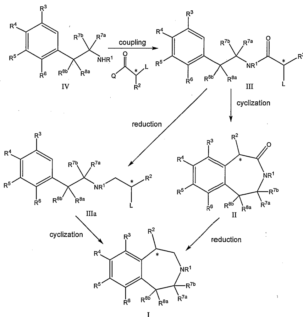
Scheme I
