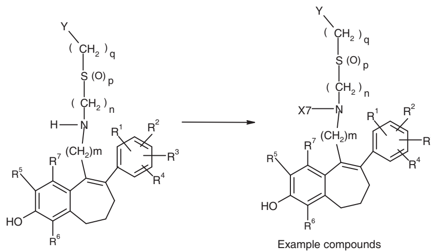
(Synthesis Scheme 11)
