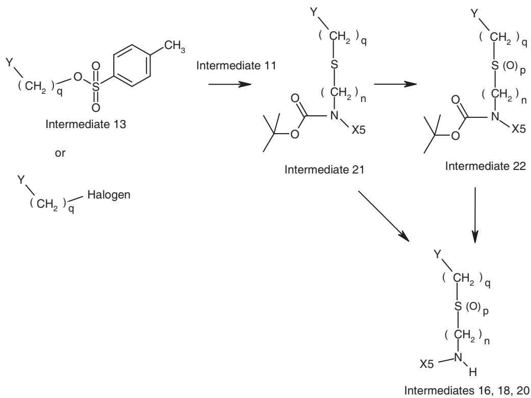
(Synthesis Scheme 9)
