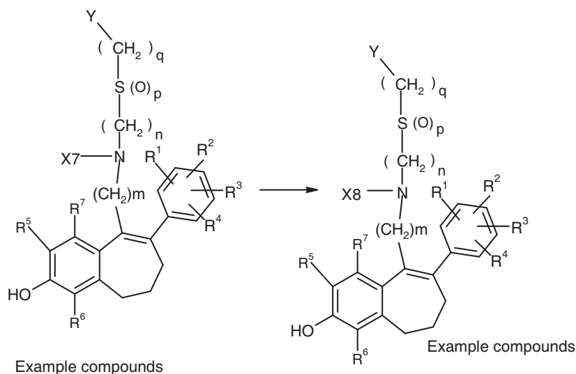
(Synthesis Scheme 12)
