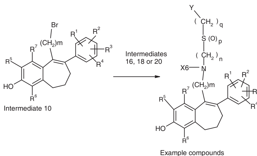
(Synthesis Scheme 10)
