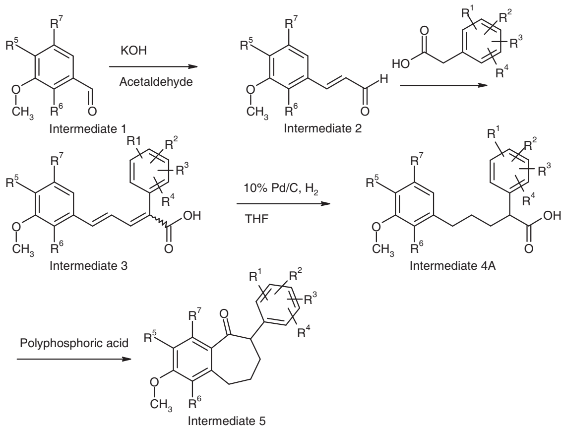
(Synthesis Scheme 1)
