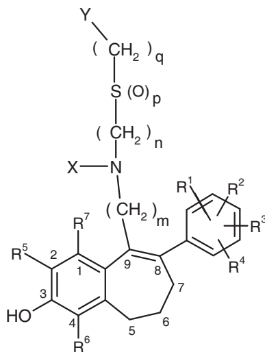
(I)
