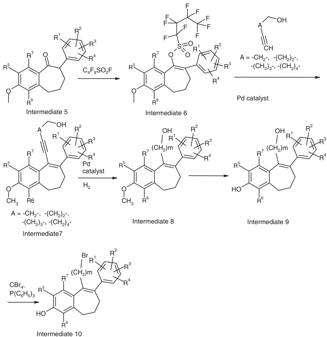
(Synthesis Scheme 3)
