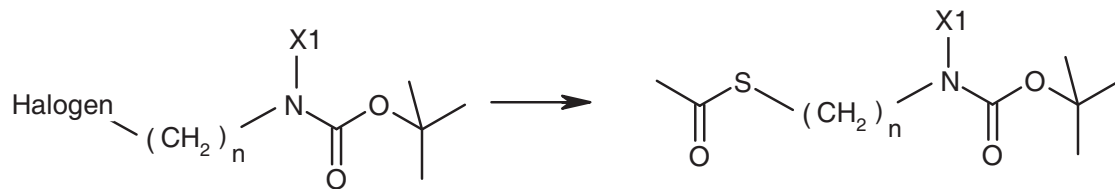
Intermediate 11
