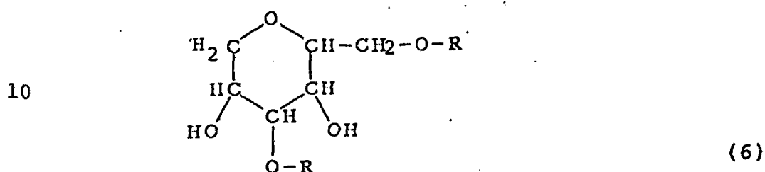
1,5-sorbitan derivative (b)
