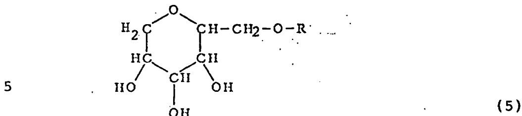
1,5-sorbitan derivative (a)
