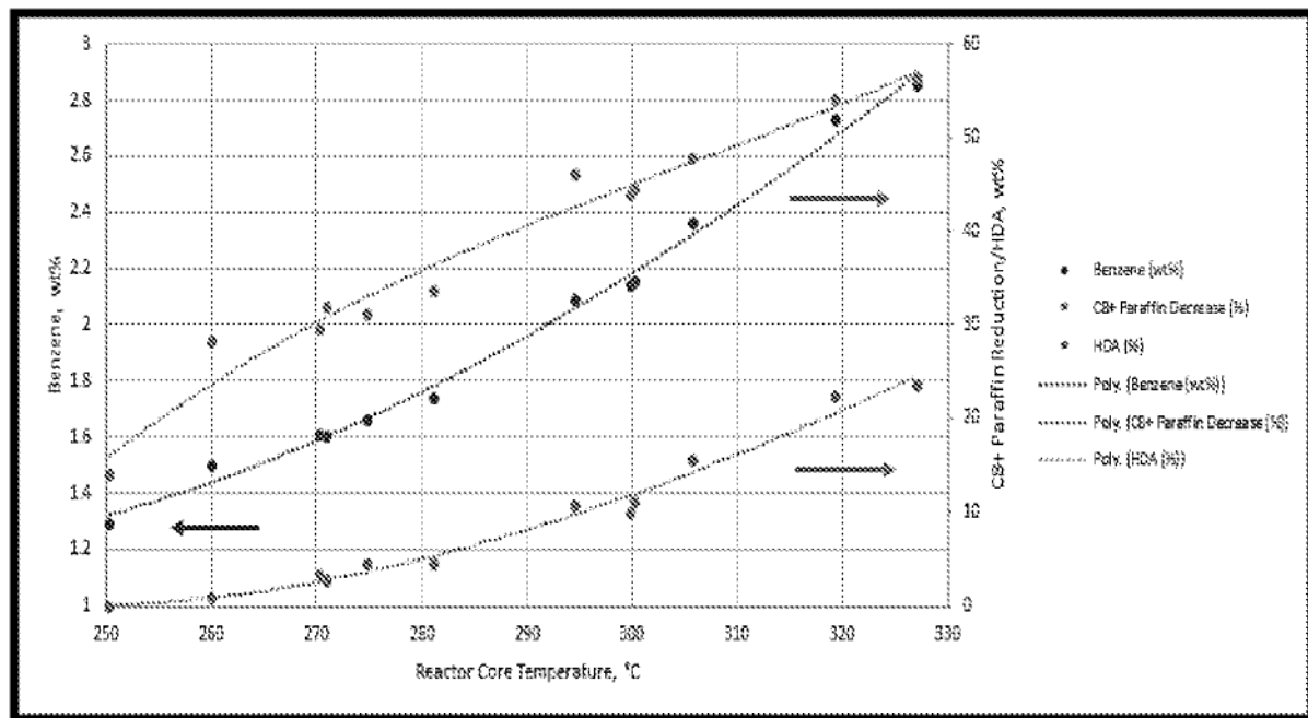
Diagram 7 - Benzene Reduction vs. I2FE Reactor Temperature
