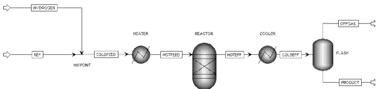
Diagram 3 – Cracking System
