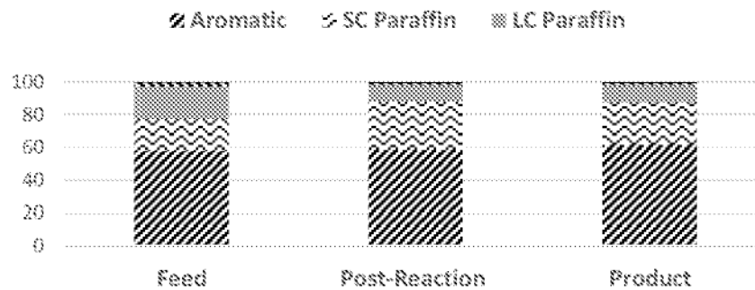
Diagram 4 – Paraffin Conversion
