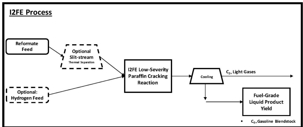
Diagram 6 – I2FE with Hydrogen Feed
