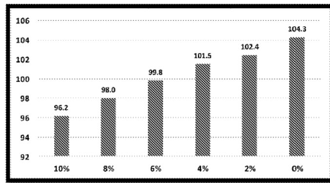
Diagram 2 – Impact of n-Paraffins (% wt.) on Reformate Octane Value
