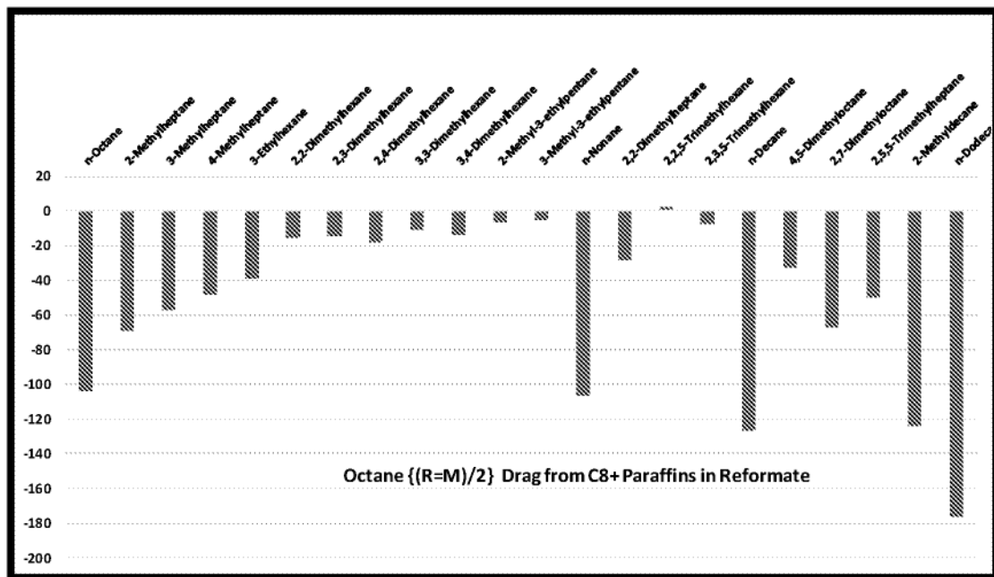
Diagram 1 – Octane Drag from C8 to C12 Paraffins Typical in Reformate
