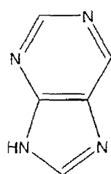
Purine
