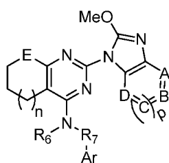
50 E = NR, O A, B, C, D = CR, CX, N, O, S Y, Z = CR, N R = H, C1-C6 alkyl or C1-C6 substituted alkyl X = halogen, alkoxy, or nitrile n = 0-3 p = 0,1
