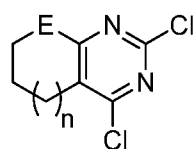
53 E = NR, O R = H, C1-C6 alkyl or C1-C6 substituted alkyl n = 0-3
