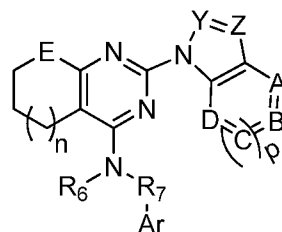
54 E = NR, O; A, B, C, D = CR, CX, N, O, S Y, Z = CR', N R = H, C1-C6 alkyl or C1-C6 substituted alkyl R' = H, alkoxy, C1-C6 alkyl or C1-C6 substituted alkyl X = halogen, alkoxy, or nitrile n = 0-3 p = 0,1
