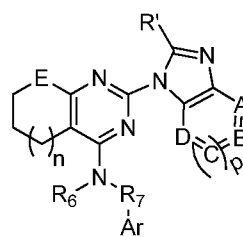
51 E = NR, O A, B, C, D = CR, CX, N, O, S Y, Z = CR, N R = H, C1-C6 alkyl or C1-C6 substituted alkyl X = halogen, alkoxy, or nitrile n = 0-3 p = 0,1
