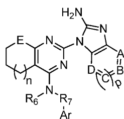
49 E = NR, O A, B, C, D = CR, CX, N, O, S Y, Z = CR, N R = H, C1-C6 alkyl or C1-C6 substituted alkyl X = halogen, alkoxy, or nitrile n = 0-3 p = 0,1
