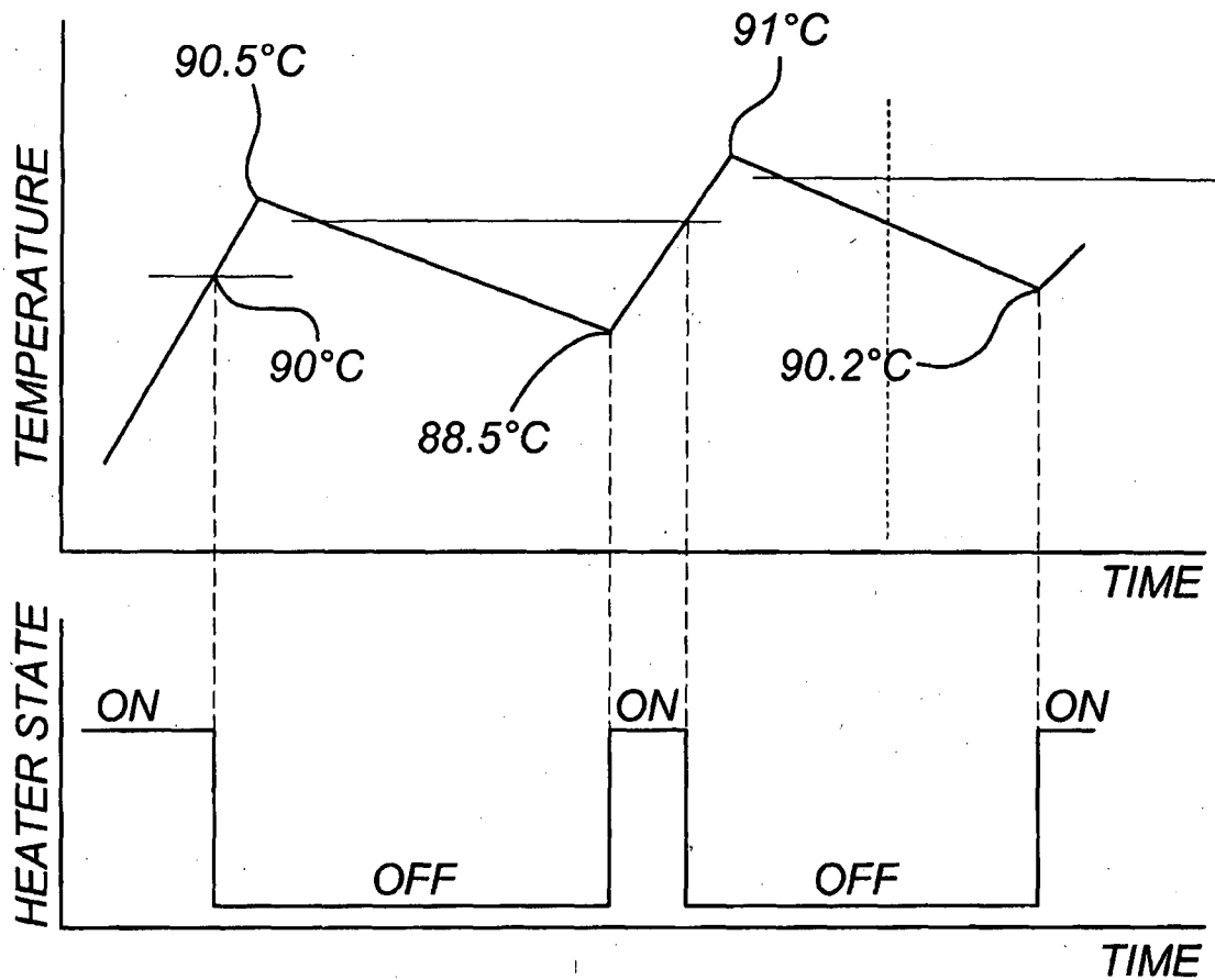
TYPICAL CALLIBRATION CYCLE
