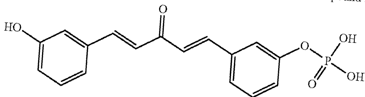
Compound 28
