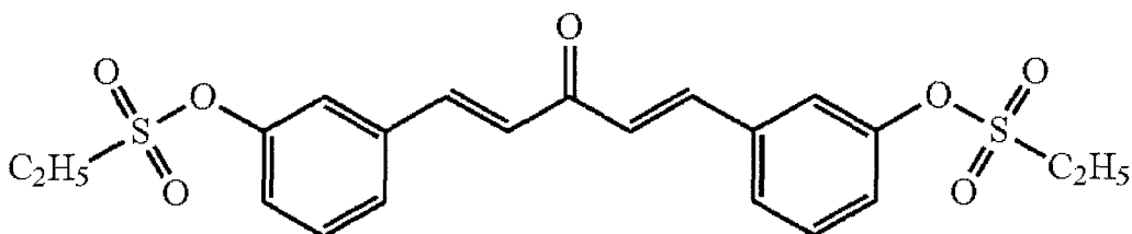
Compound 7
