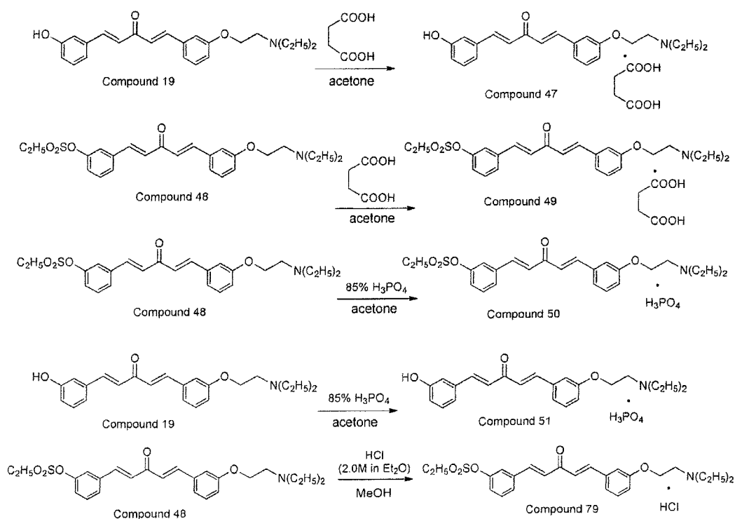
Scheme 9
