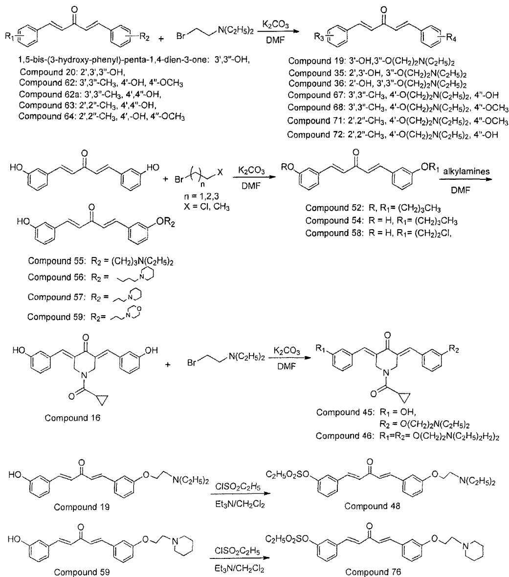
Scheme 8
