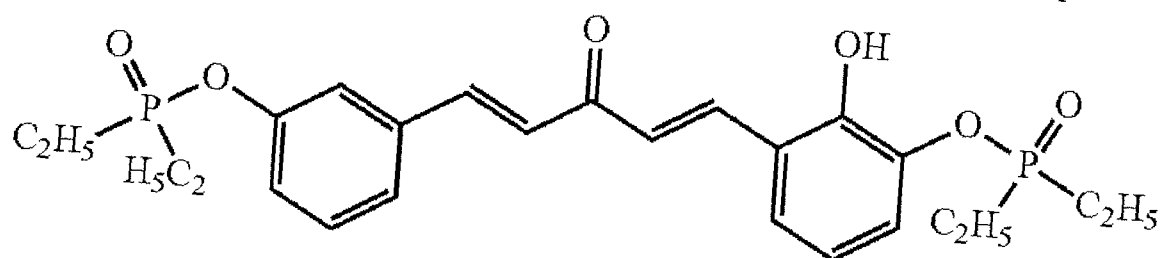
Compound 34
