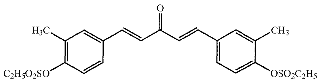
Compound 66
