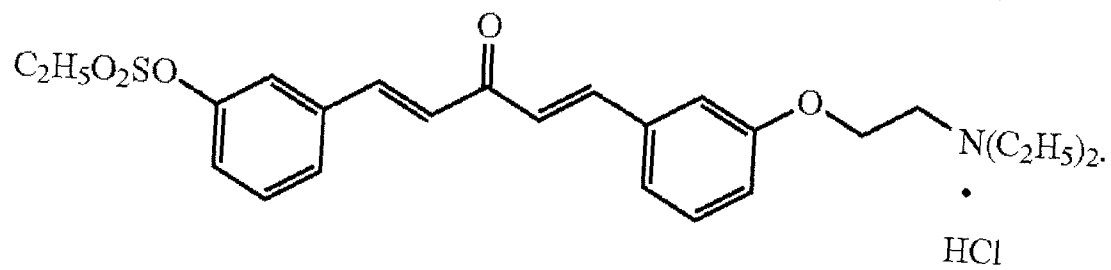
Compound 79
