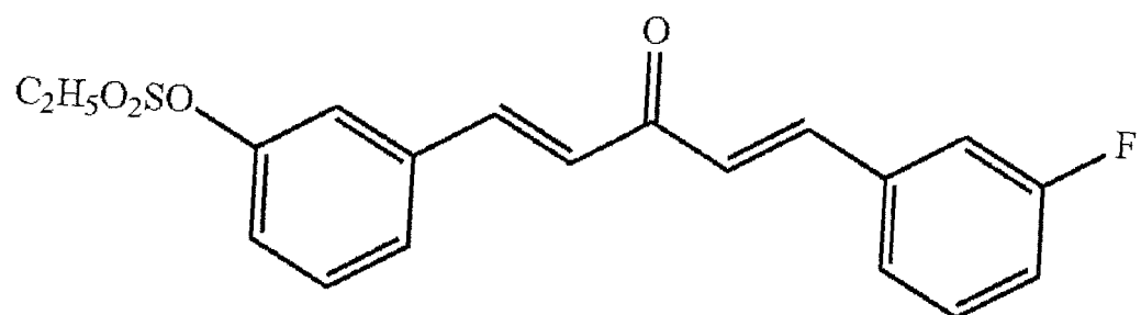
Compound 77
