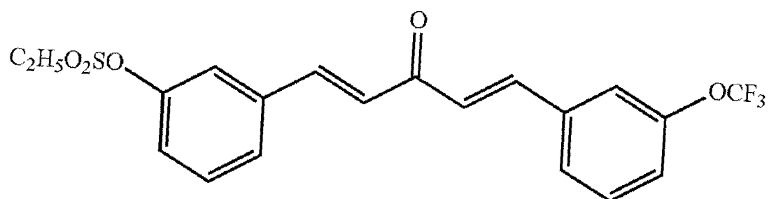
Compound 79
