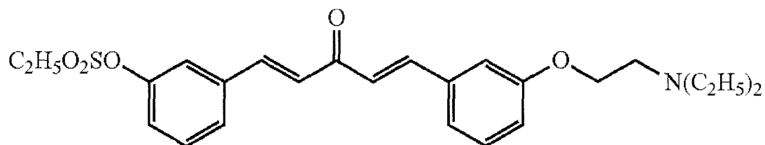
Compound 48
