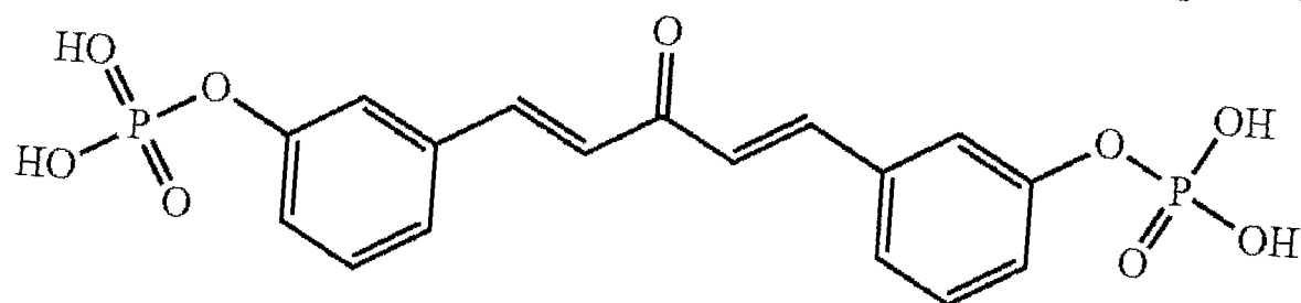
Compound 29
