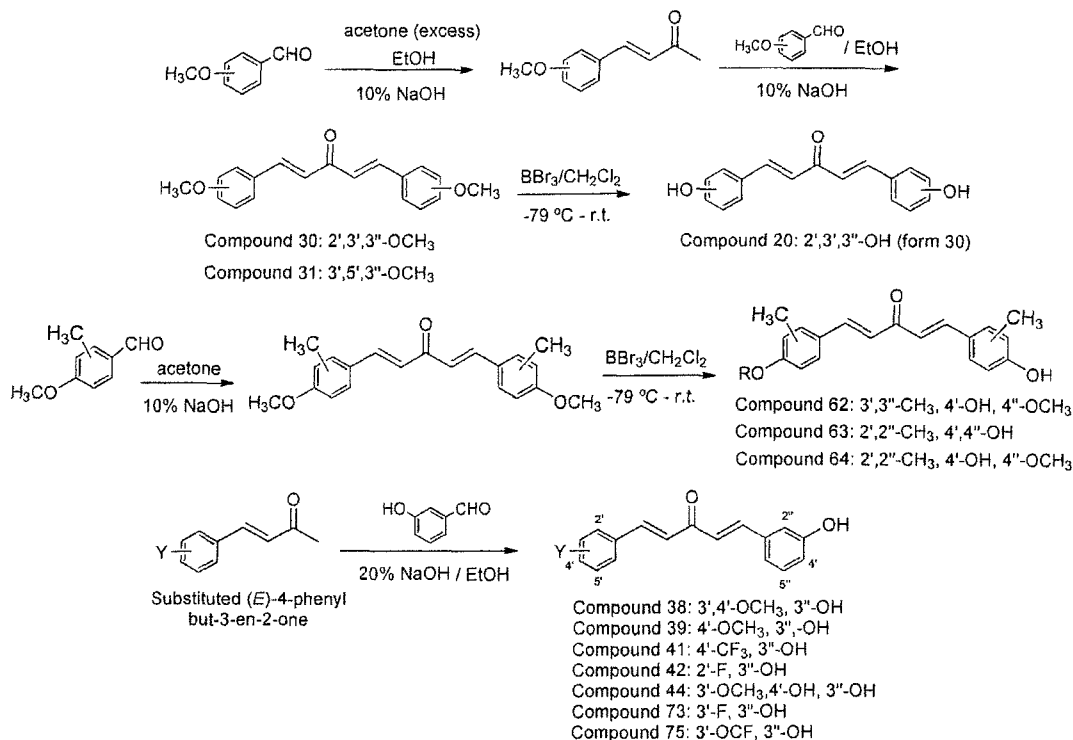
Scheme 5
