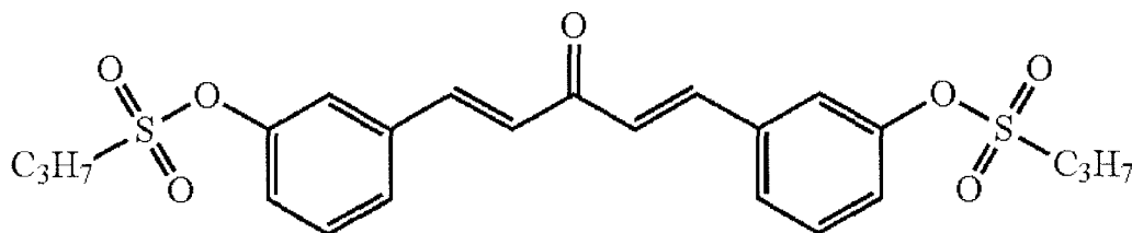
Compound 9
