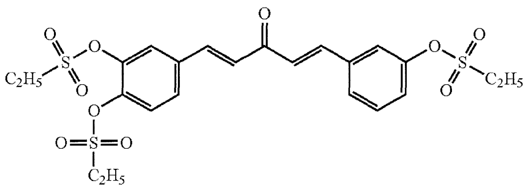
Compound 43
