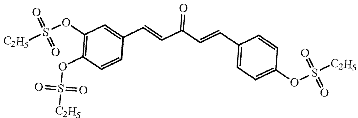
Compound 11
