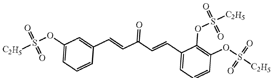
Compound 26
