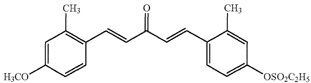
Compound 70
