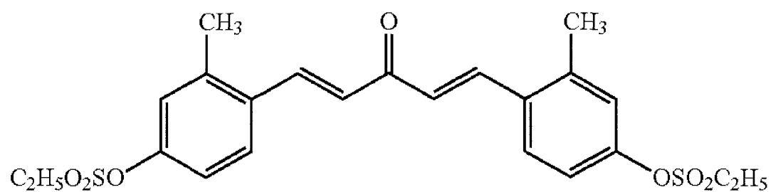
Compound 70
