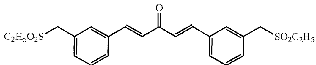
Compound 60
