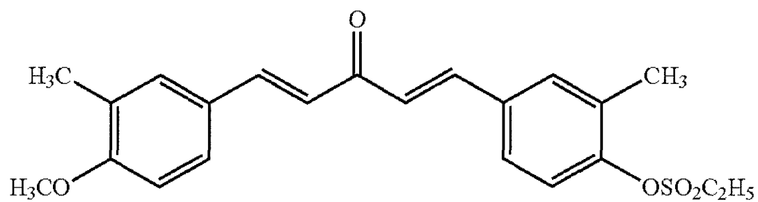
Compound 69
