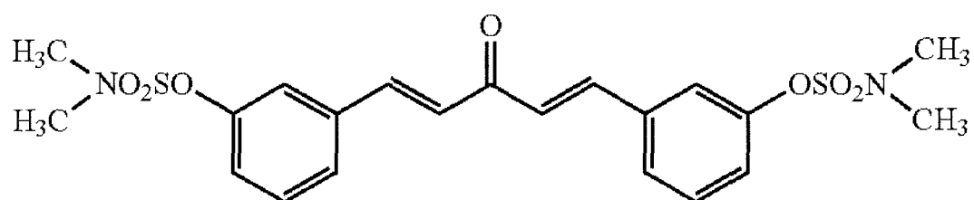
Compound 60
