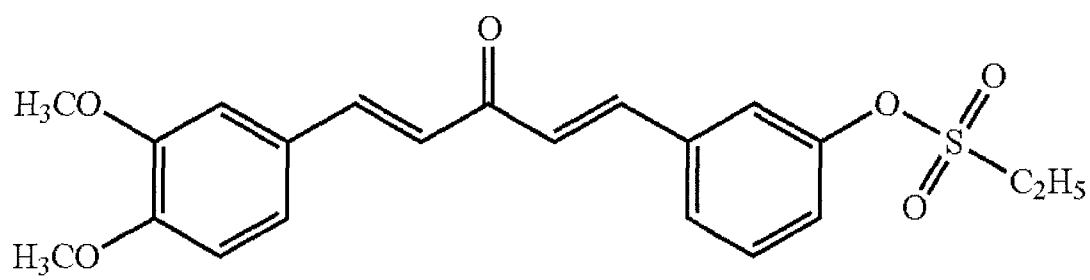
Compound 40
