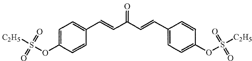
Compound 6
