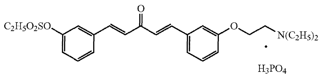
Compound 53
