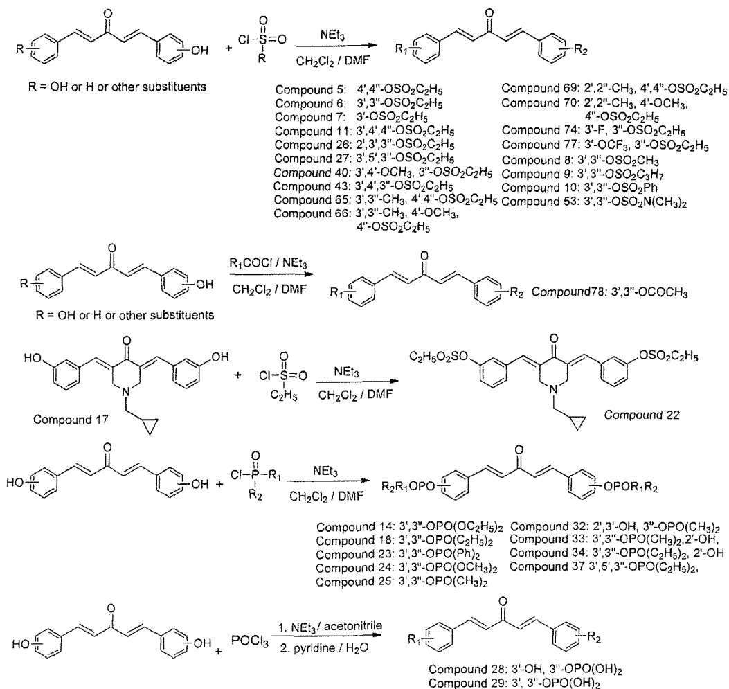
Scheme 7
