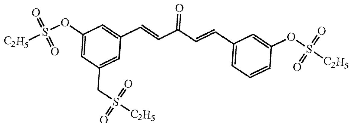
Compound 27
