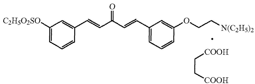
Compound 50
