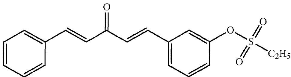
Compound 9
