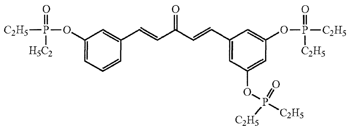
Compound 37
