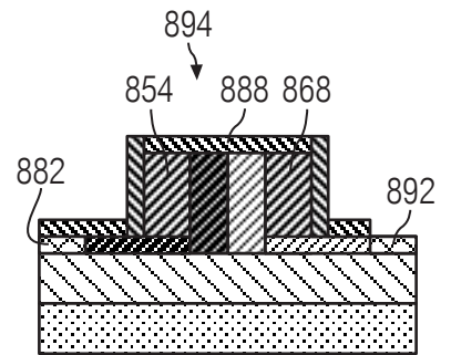
(15) N++ ION IMPLANTATION
