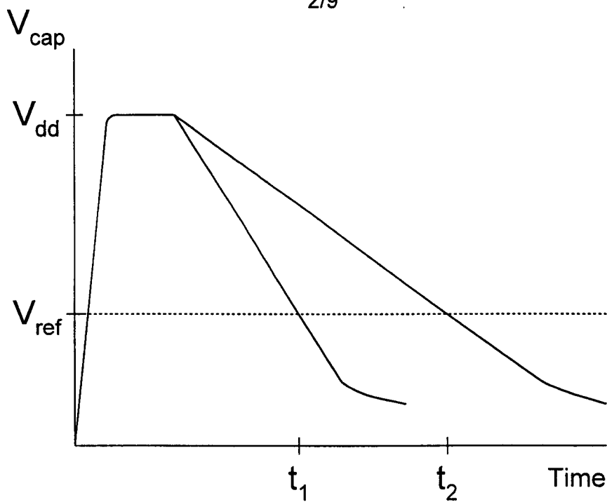
FIG. 3 (PRIOR ART)
