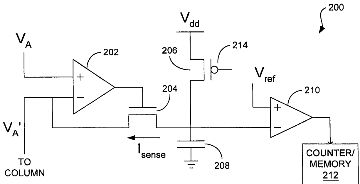
FIG. 2 (PRIOR ART)
