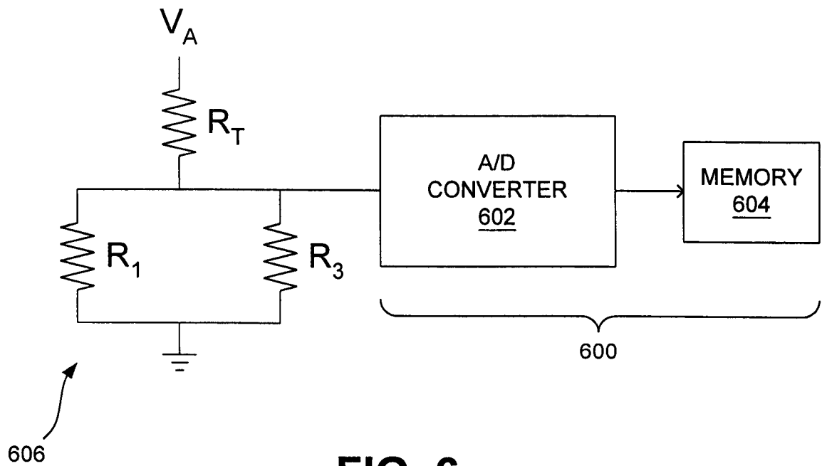
FIG. 6 (PRIOR ART)
