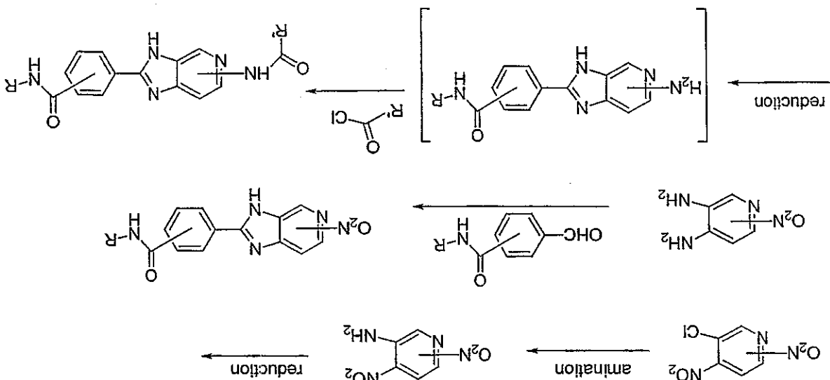
Synthetic Scheme 22
