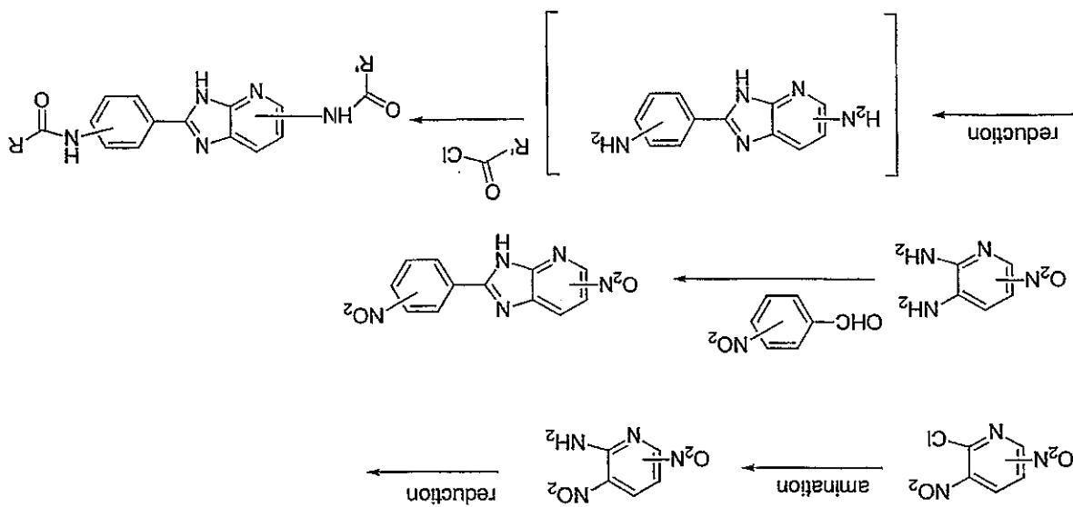
Synthetic Scheme 28
