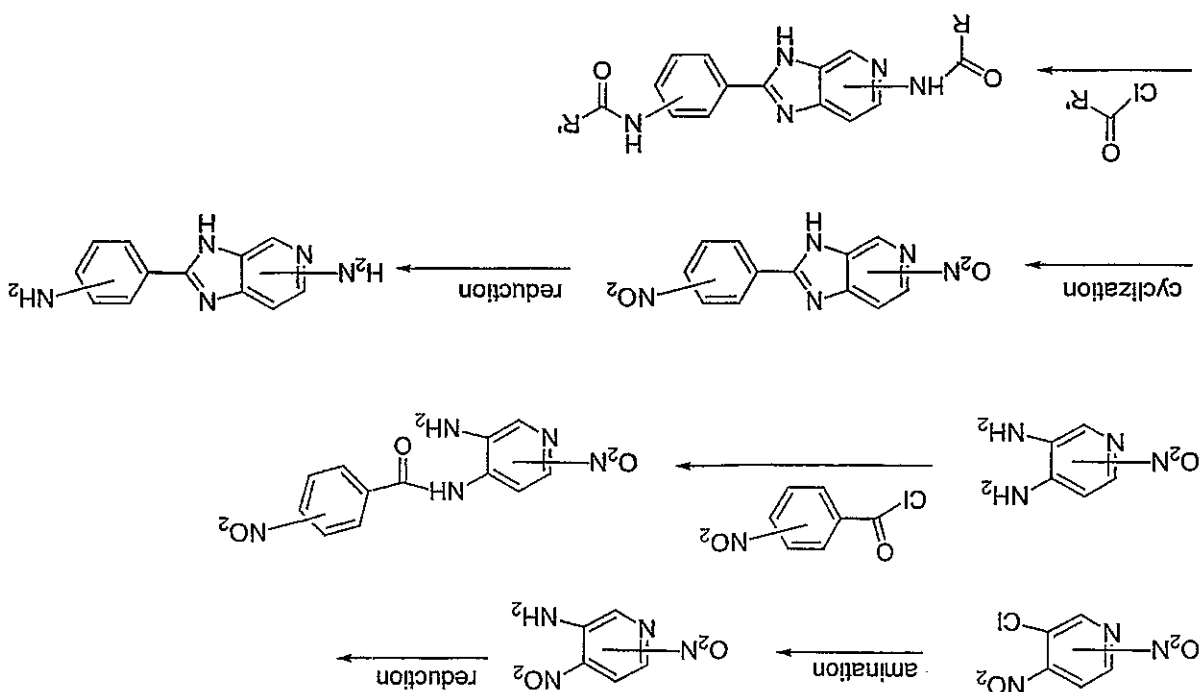
Synthetic Scheme 29
