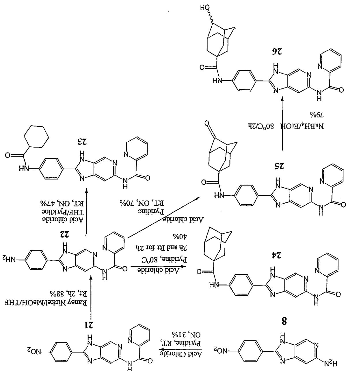
Scheme 41
