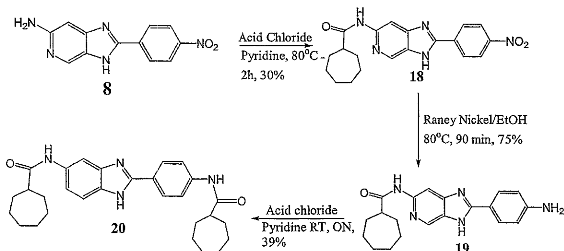
Scheme 40
