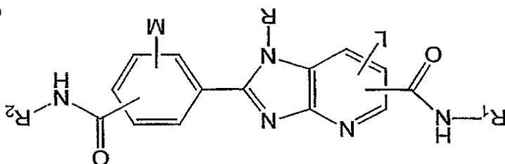
Genus B4
