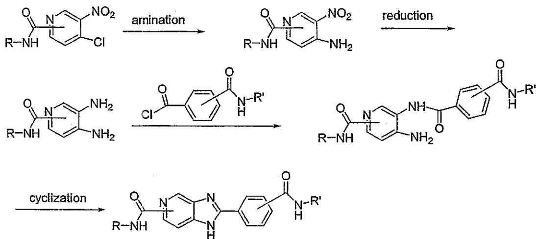
Synthetic Scheme 15
