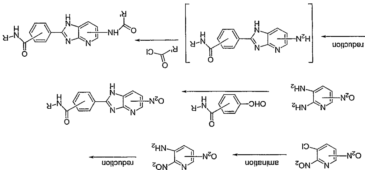
Synthetic Scheme 26
