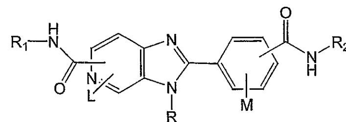
Genus B2;
