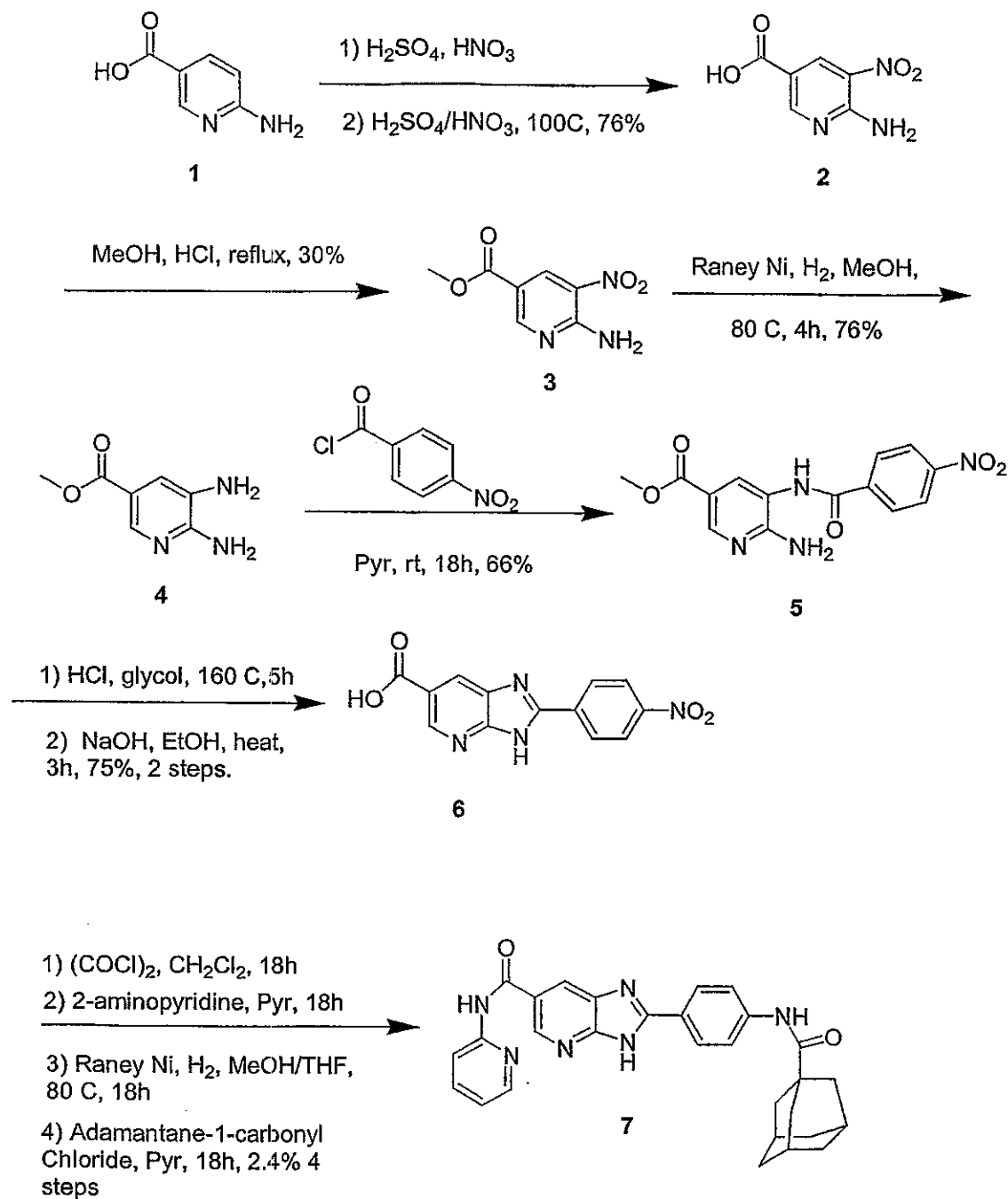
Scheme 42
