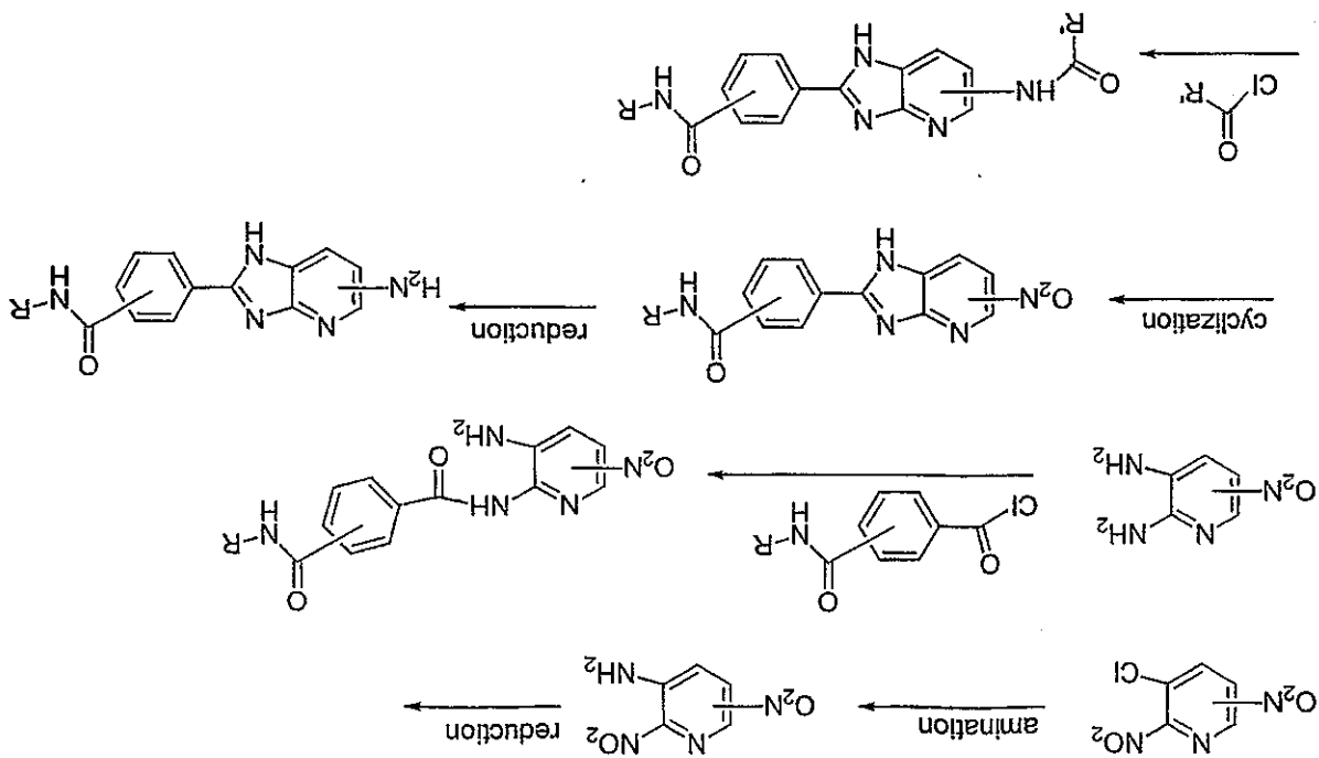
Synthetic Scheme 25
