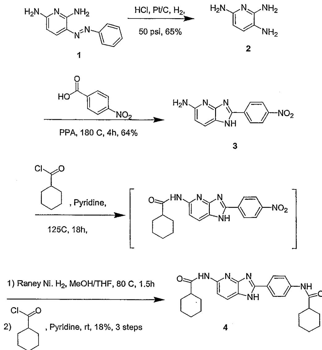
Scheme 43
