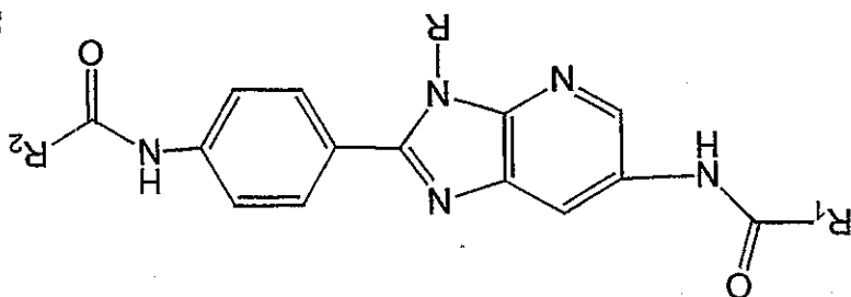
Subgenus Dia;
