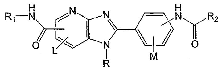
Genus A4;
