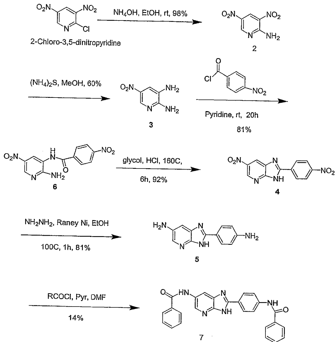
Scheme 36
