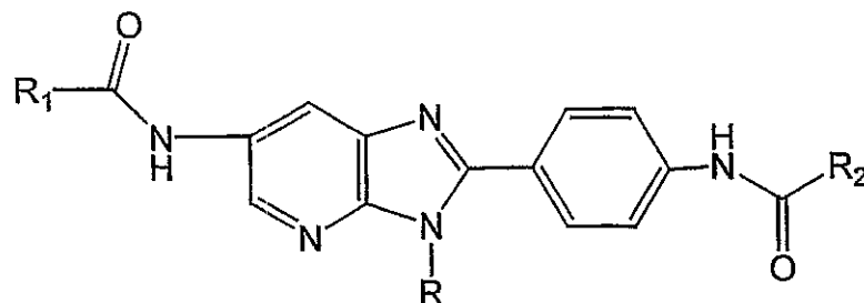
Subgenus D1a;
