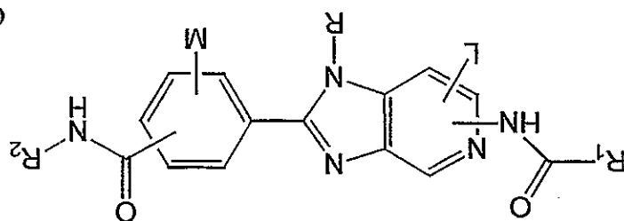
Genus C3;
