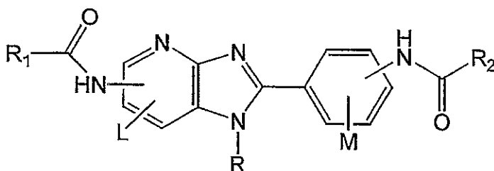
Genus D4;
