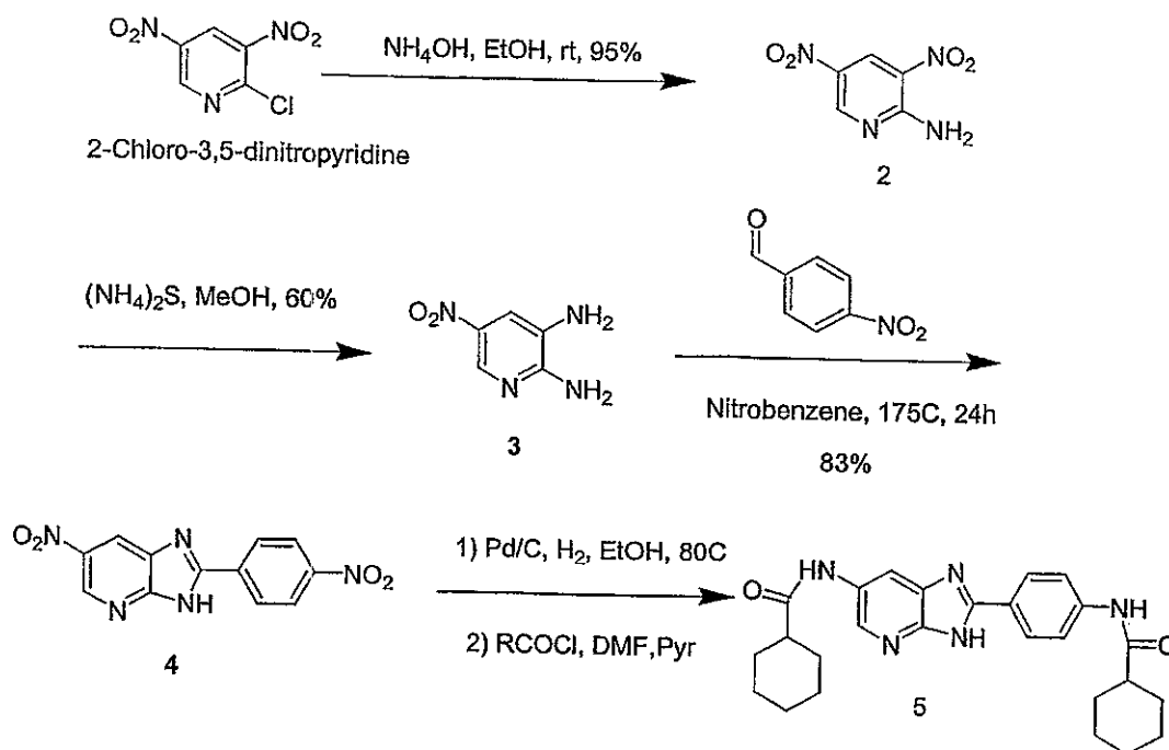
Scheme 35
