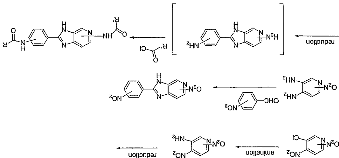
Synthetic Scheme 30
