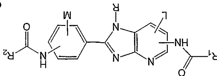
Genus D4
