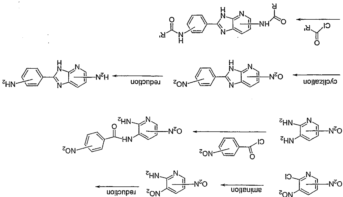
Synthetic Scheme 27
