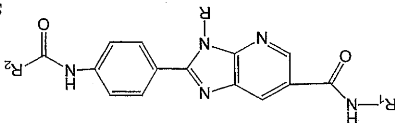
Subgenus A1a;
