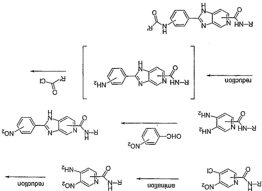
Synthetic Scheme 6
