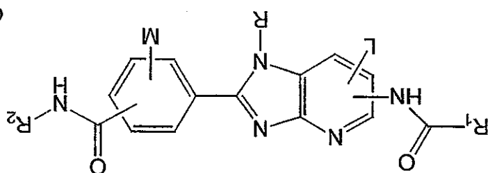
Genus C4;
