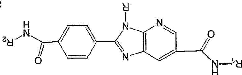
Subgenus B1a;
