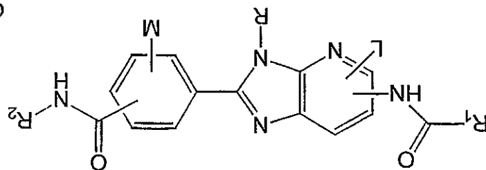
Genus C1;
