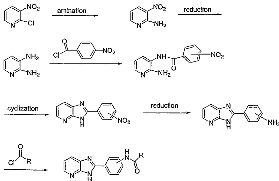
Synthetic Scheme 9
