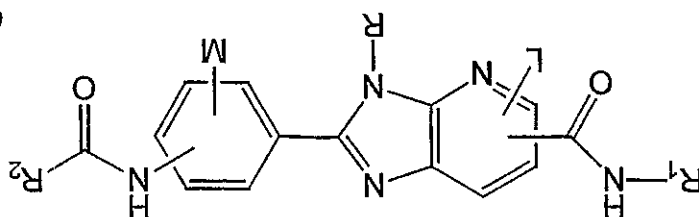
Genus A1;
