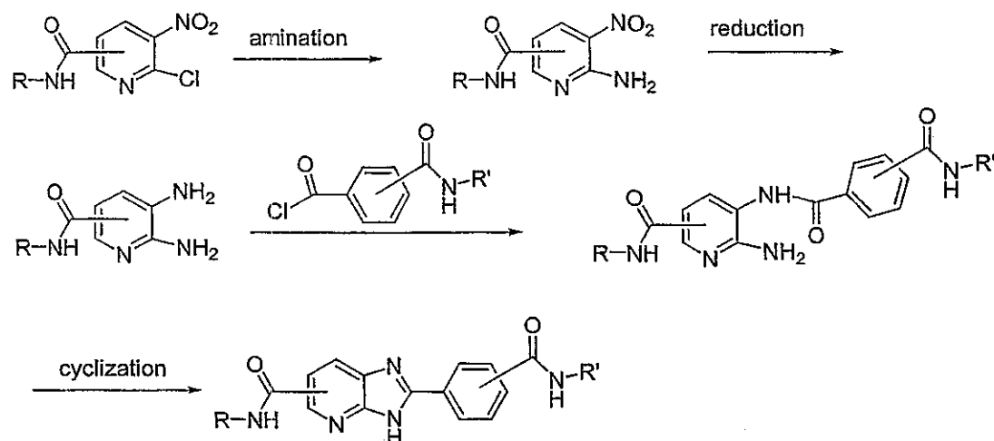
Synthetic Scheme 11
