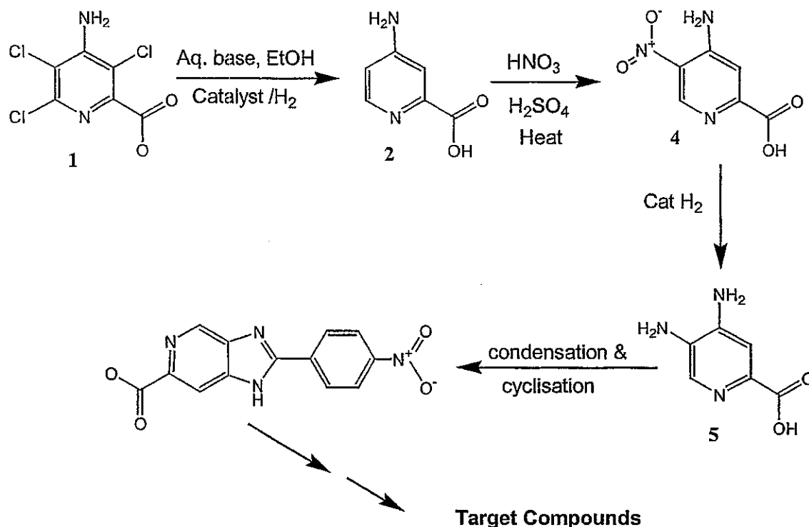
Scheme 44
