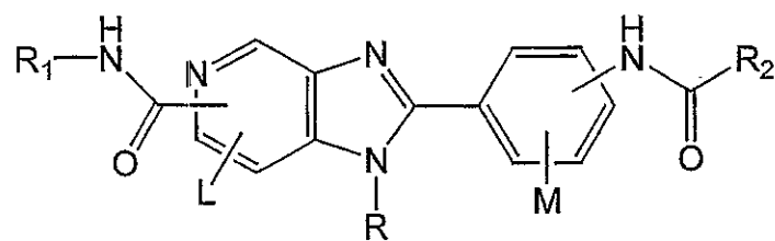
Genus A3;
