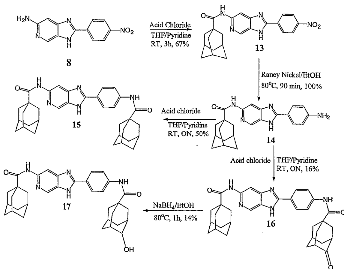
Scheme 39
