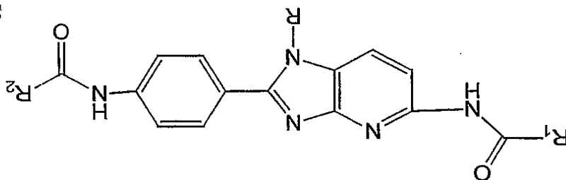
Subgenus D4a;
