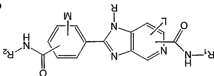
Genus B3
