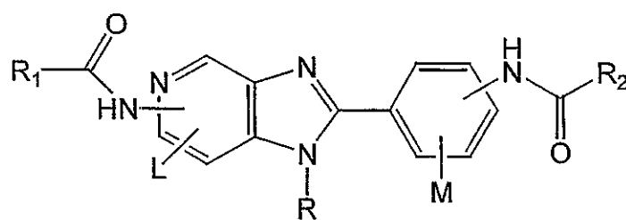
Genus D3
