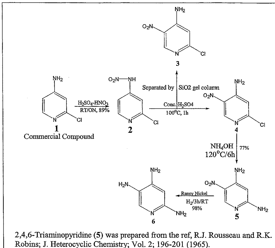
Scheme 37
