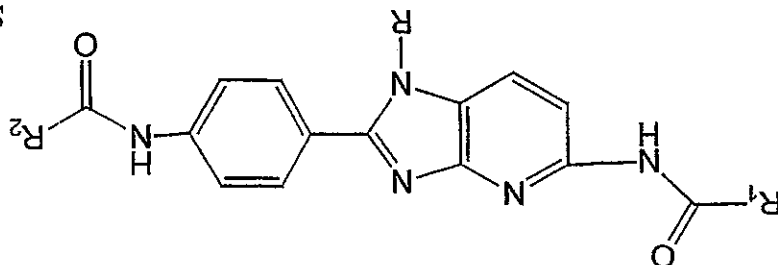
Subgenus D4a:
