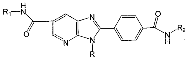
Subgenus B1a;
