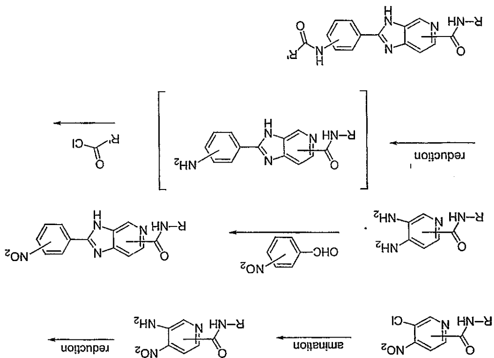
Synthetic Scheme 4
