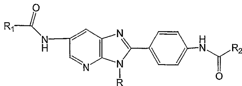
Subgenus D1a;
