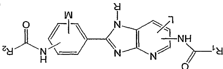
Genus D4
