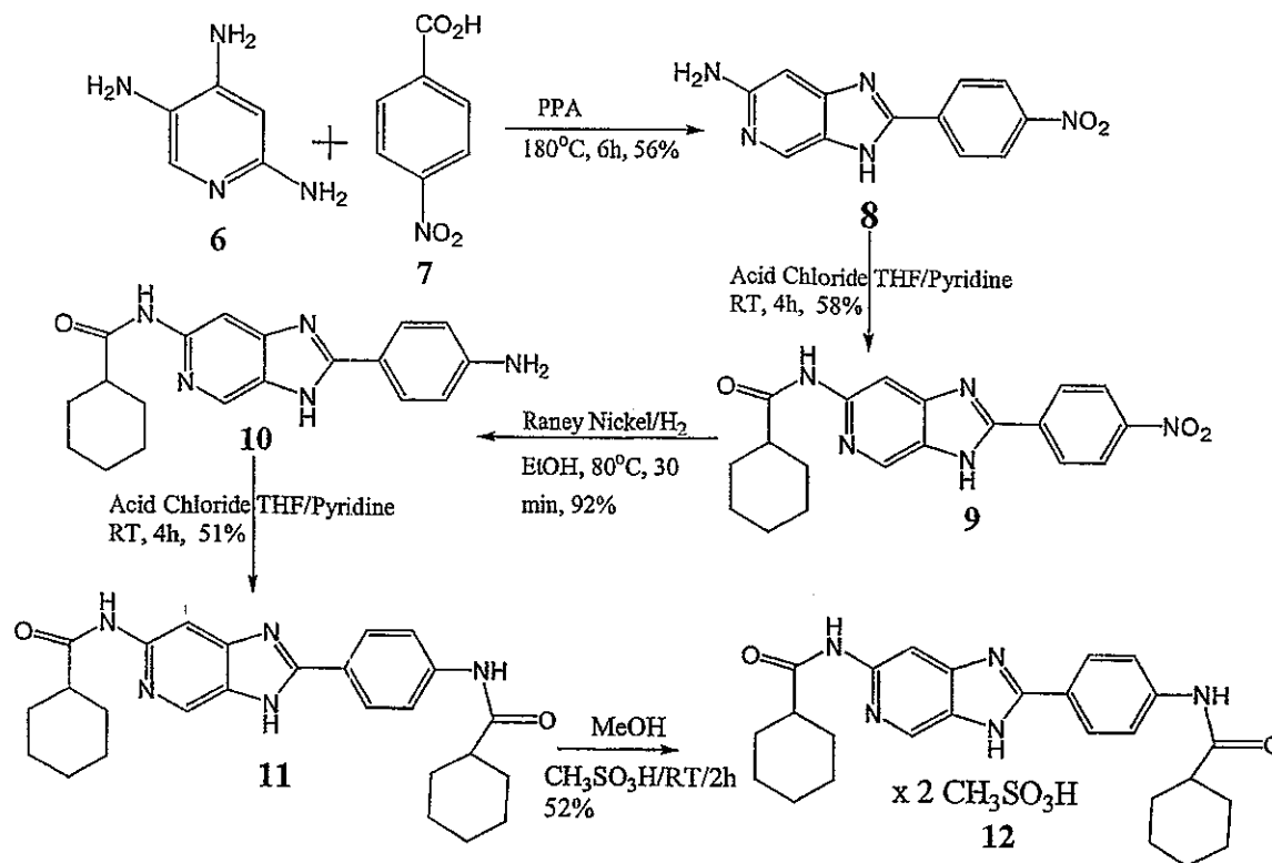
Scheme 38
