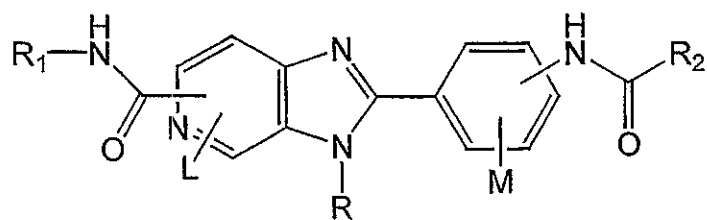
Genus A2;
