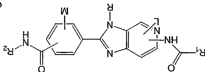
Genus C2;
