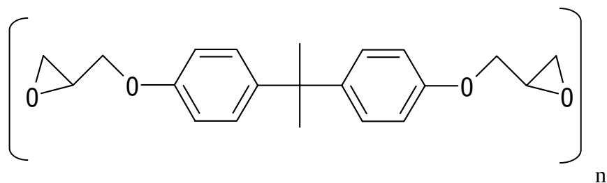
Formula 5
