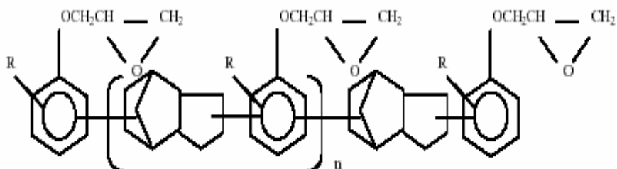
Formula 3
