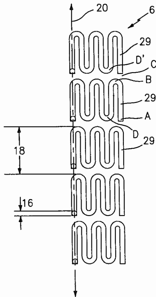
FIG. 4 (PRIOR ART)
