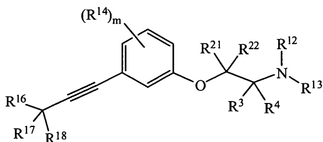
Formula (F)
