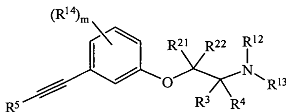
Formula (E)
