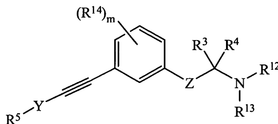
Formula (A)
