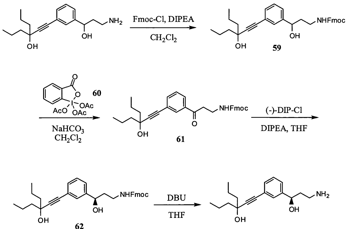
Scheme 15
