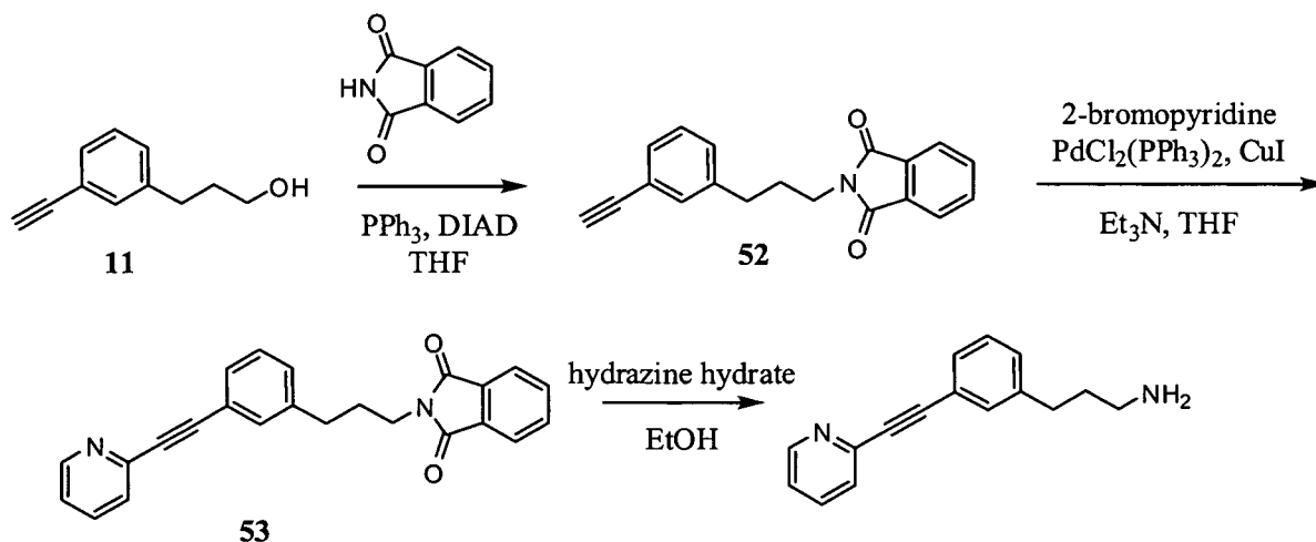
SCHEME 12
