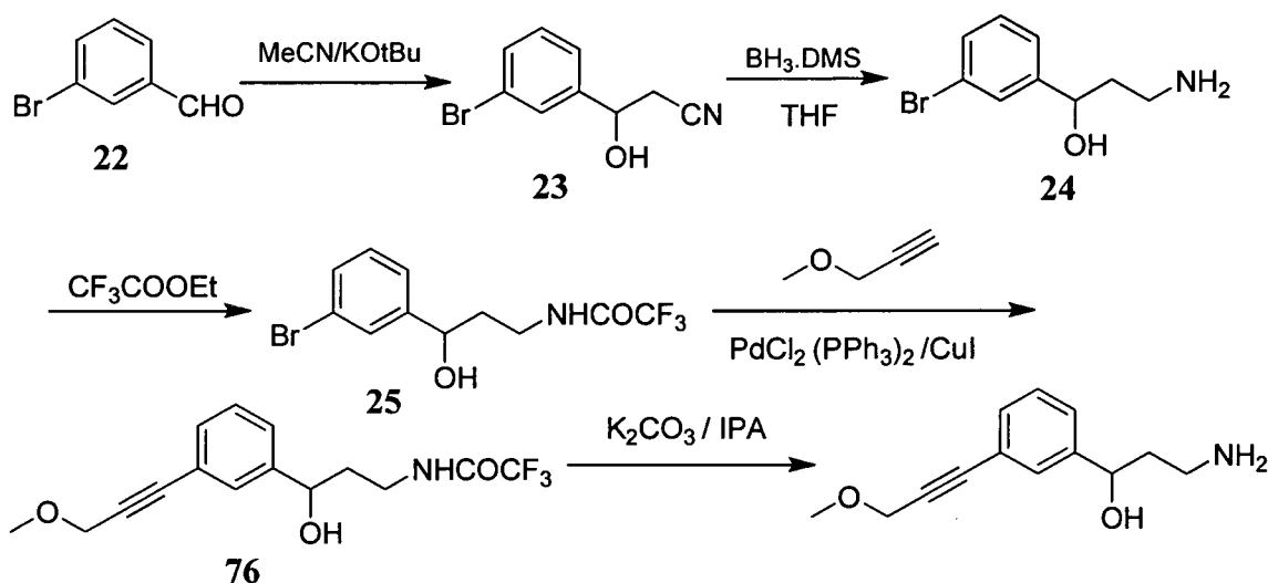
SCHEME 18
