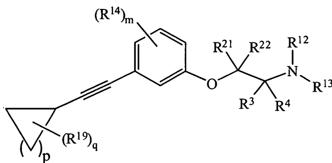
Formula (G)
