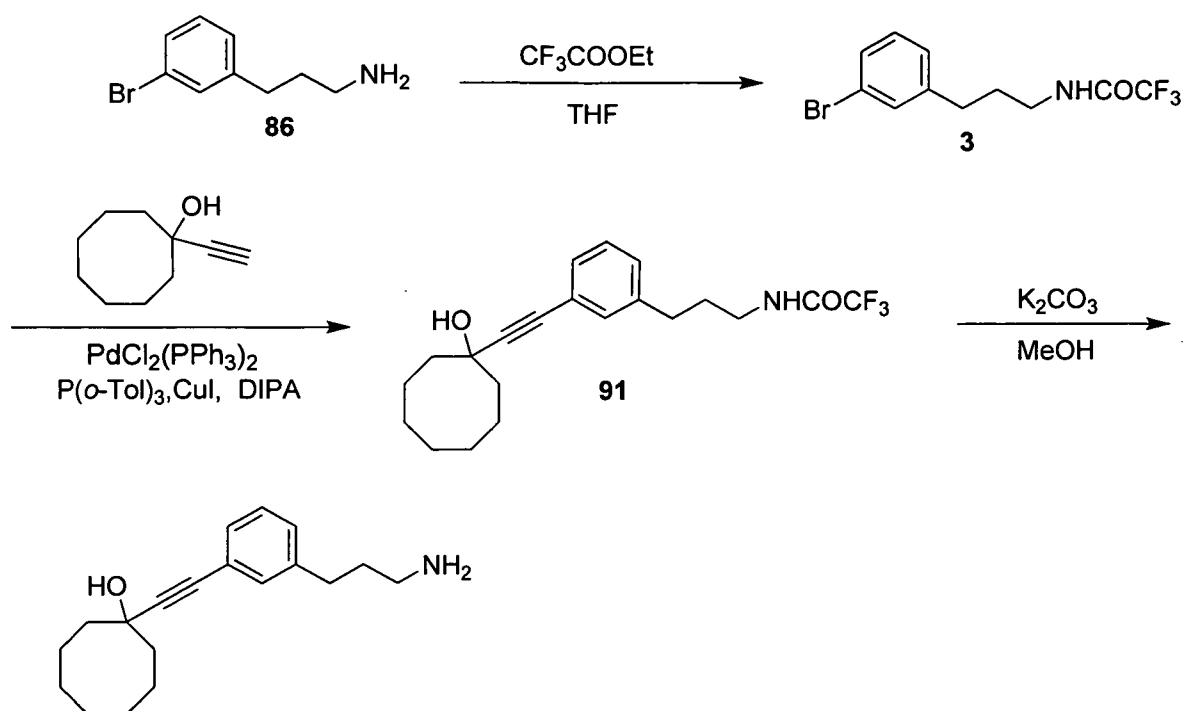
SCHEME 23
