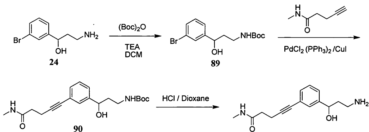
SCHEME 22
