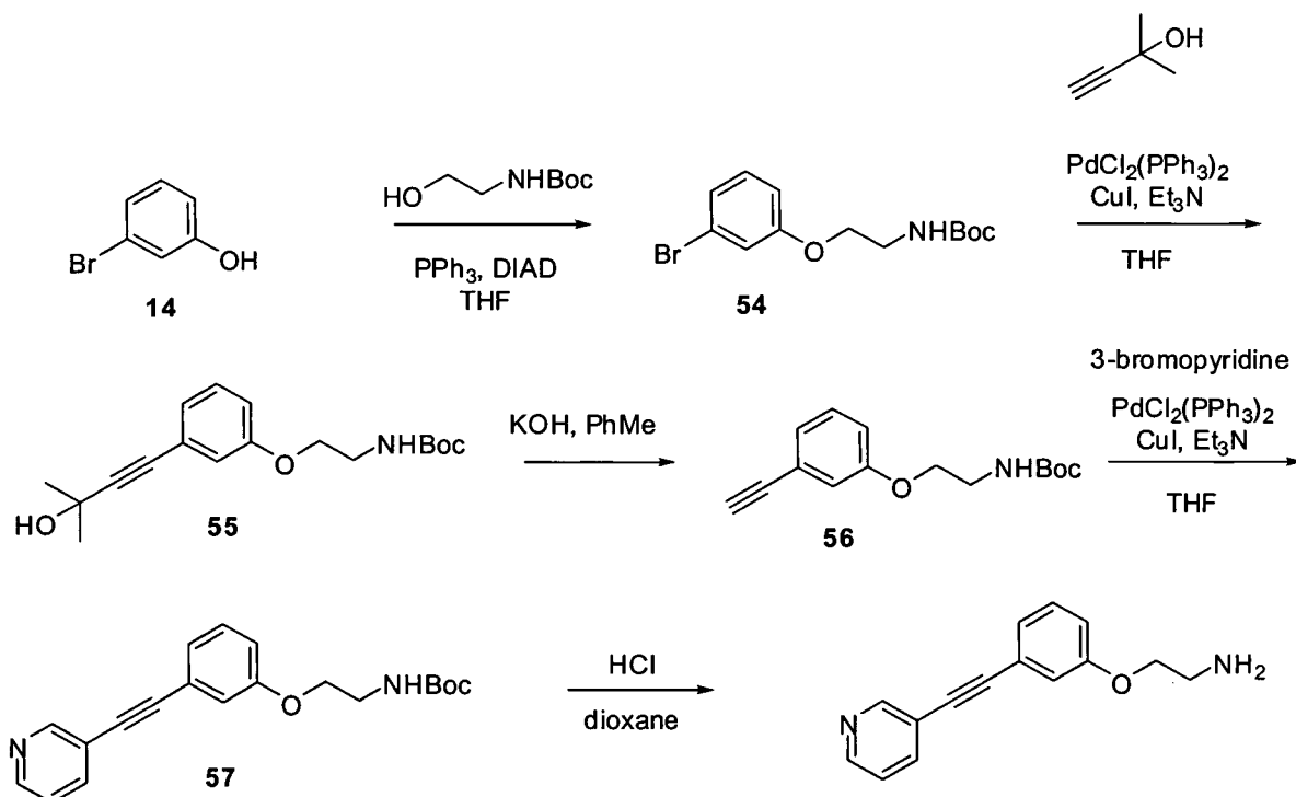
SCHEME 13
