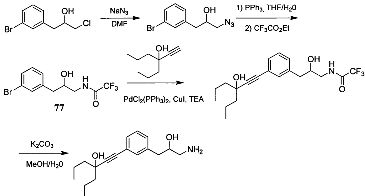
SCHEME 19
