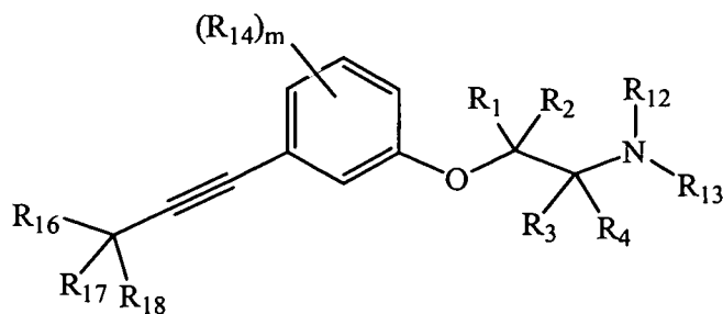
Formula (IIIa)
