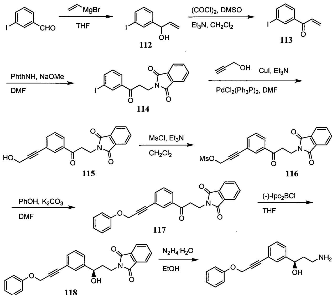
SCHEME 28
