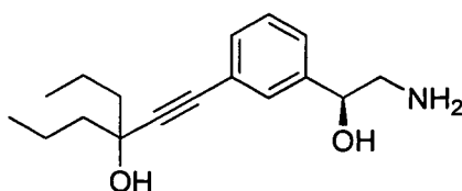
(S)-4-((3-(2-amino-1-hydroxyethyl)phenyl)-ethynyl)heptan-4-ol
