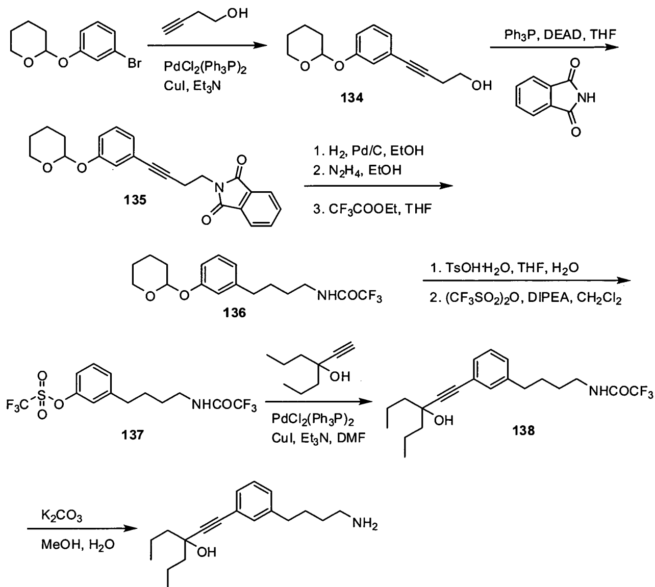
SCHEME 33
