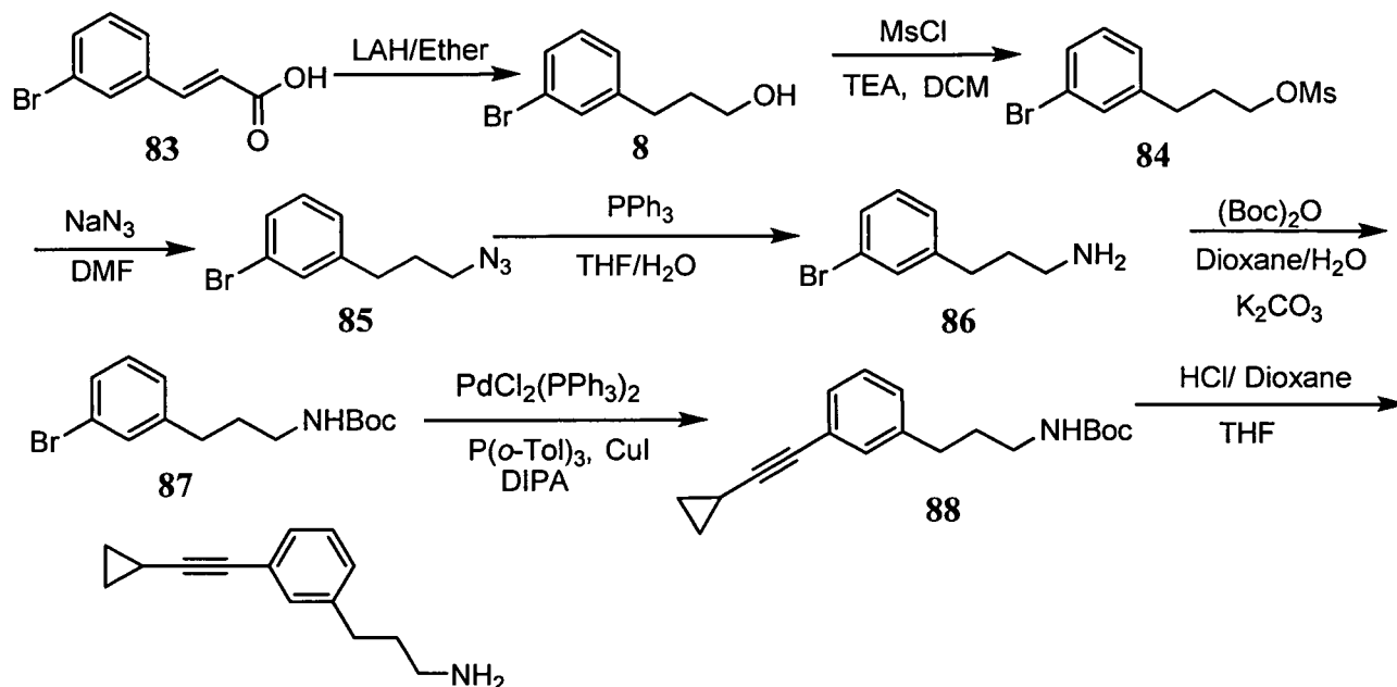
SCHEME 21
