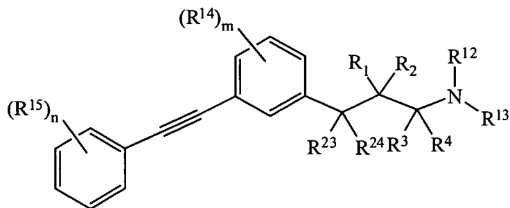
Formula (B)
