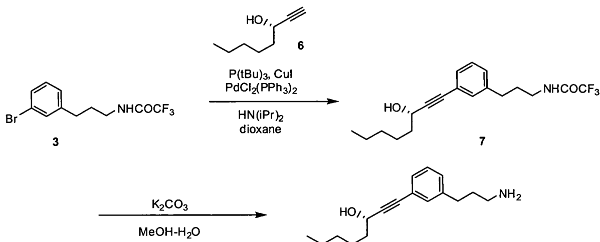
SCHEME 2
