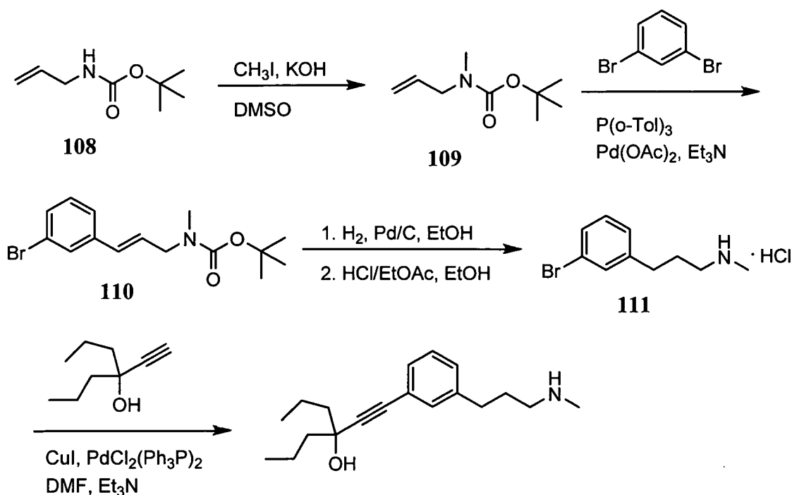
SCHEME 27
