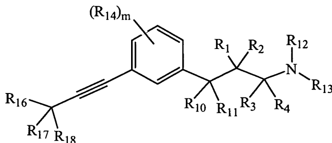
Formula (IIb)
