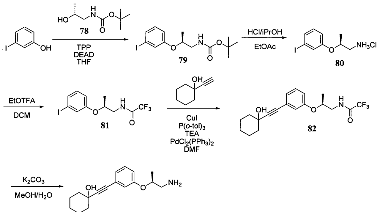
SCHEME 20
