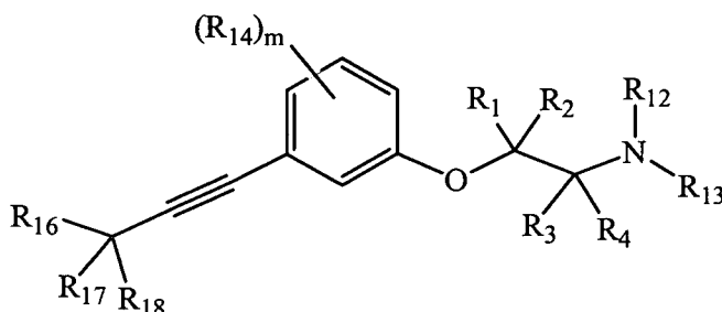
Formula (IIIa)
