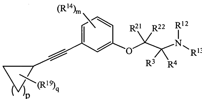
Formula (G)
