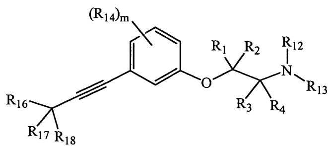
Formula (IIIa)
