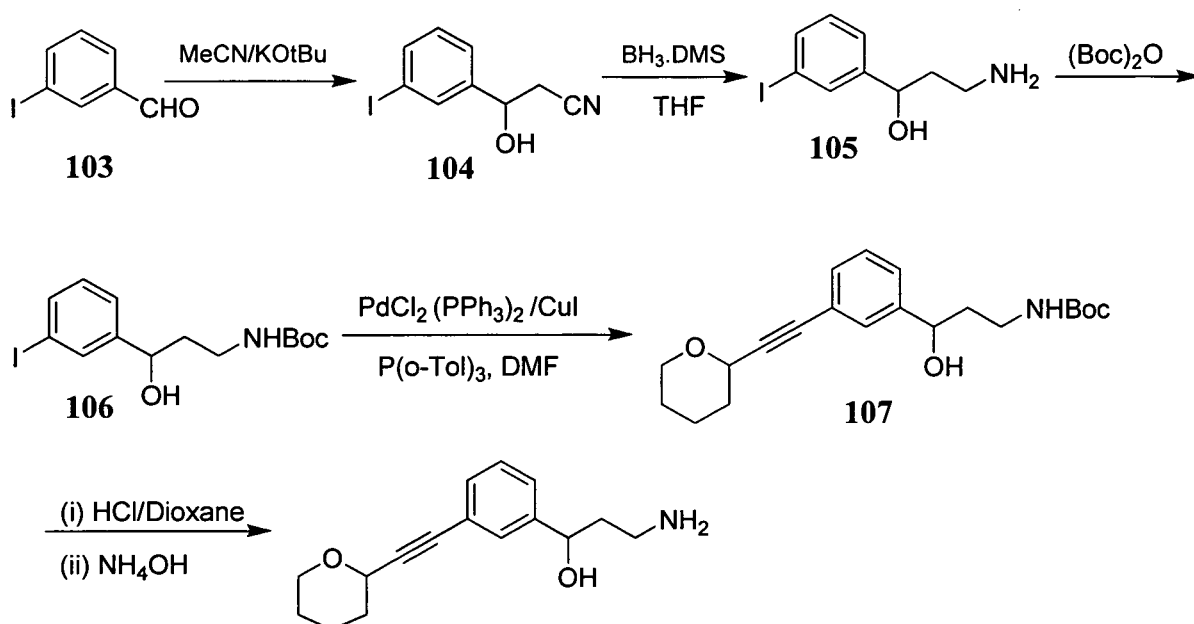
SCHEME 26
