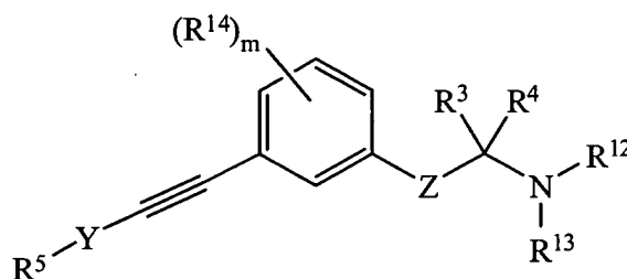
Formula (A)
