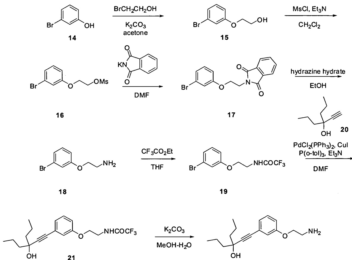
SCHEME 4
