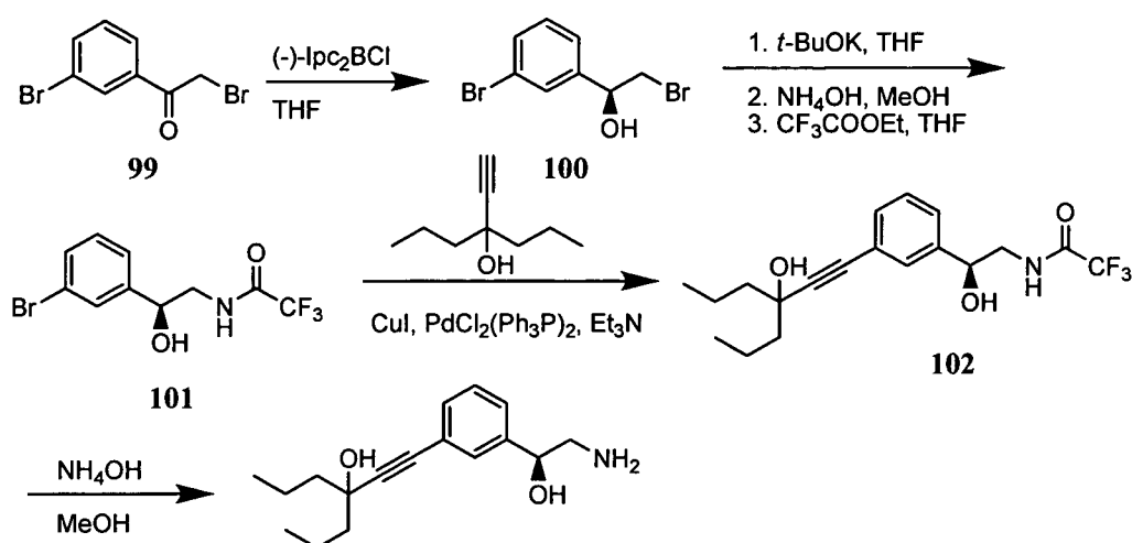
SCHEME 25
