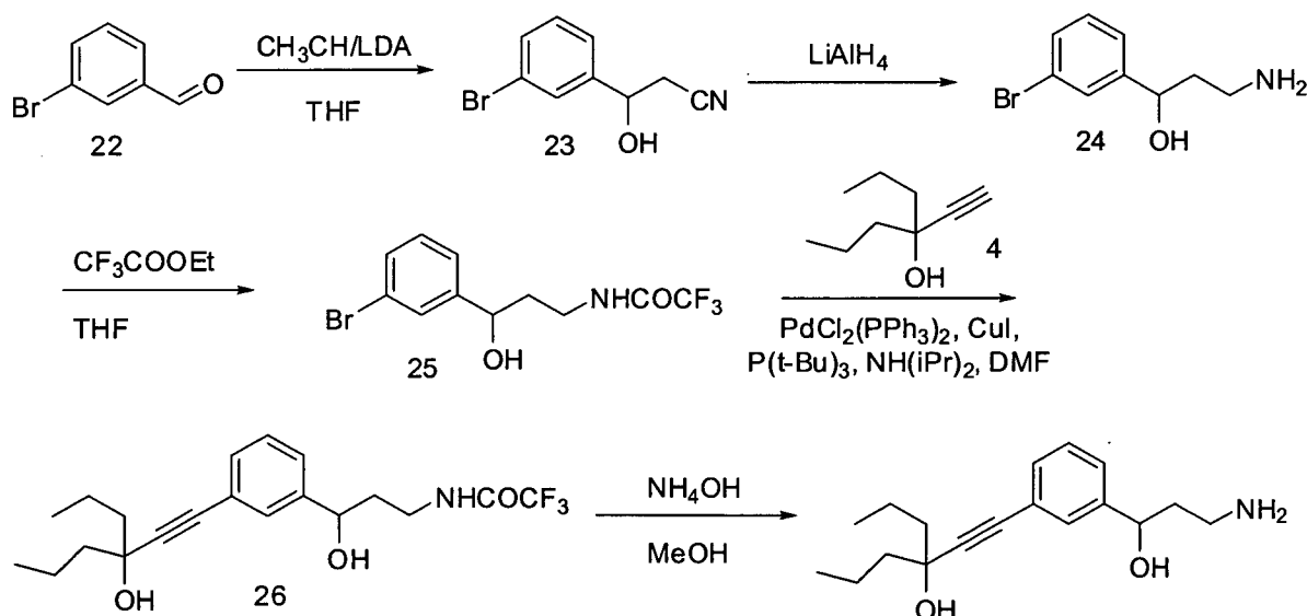
SCHEME 5
