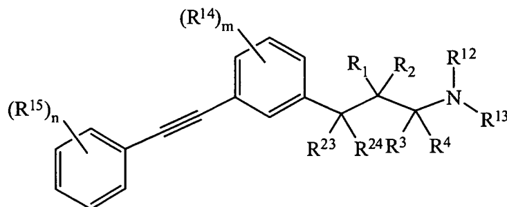
Formula (B)
