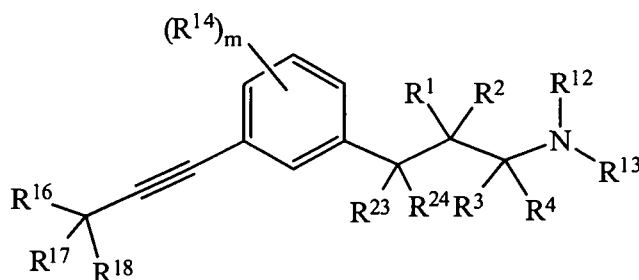
Formula (C)
