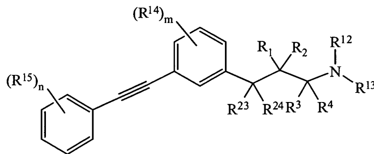
Formula (B)
