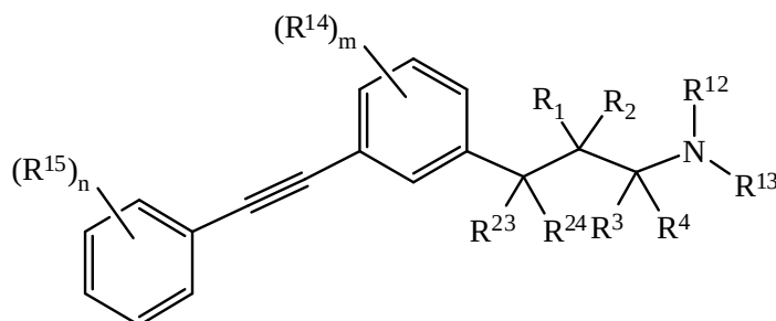
Formula (B)
