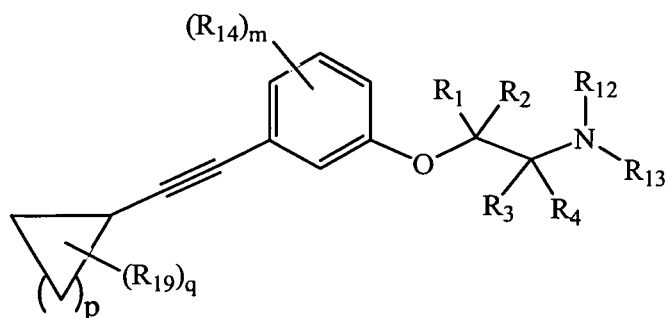
Formula (IIIb)
