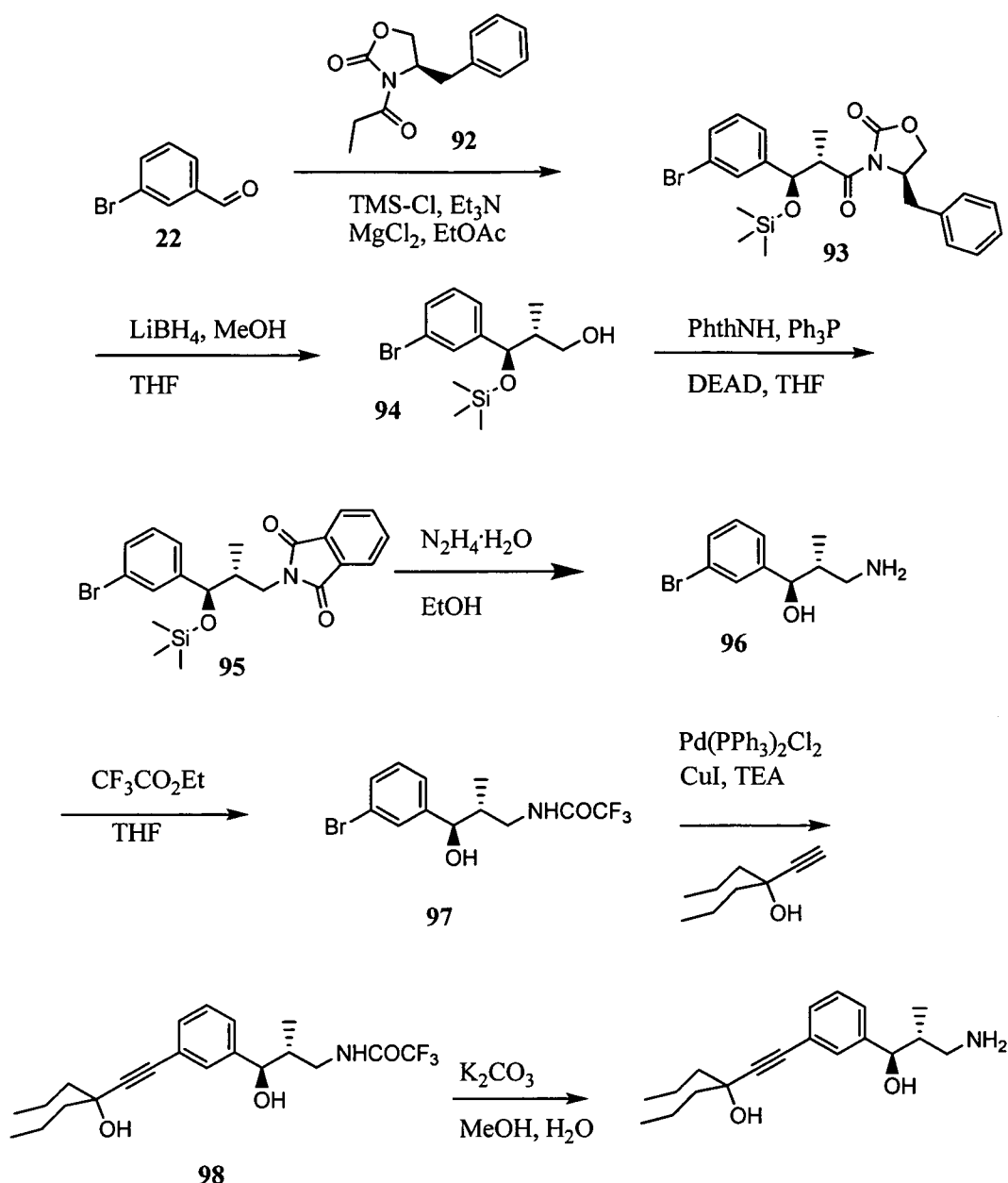
SCHEME 24
