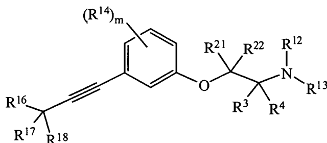
Formula (F)
