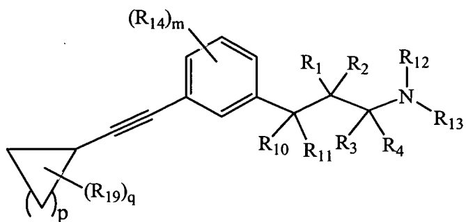
Formula (IIc)
