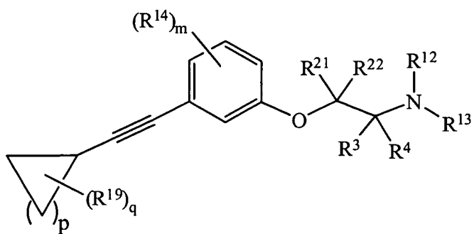
Formula (G)
