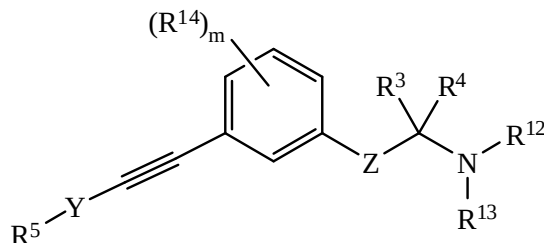
Formula (A)
