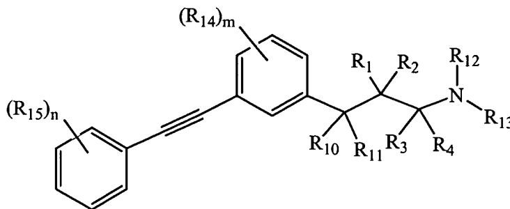
Formula (IIa)
