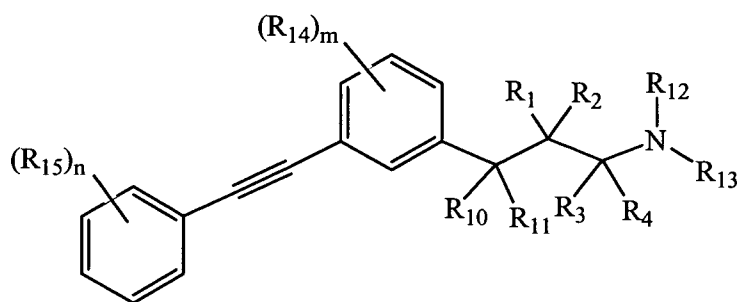
Formula (IIa)
