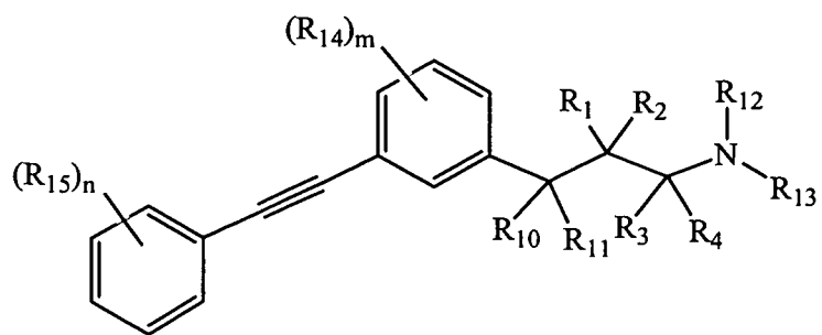
Formula (IIa)
