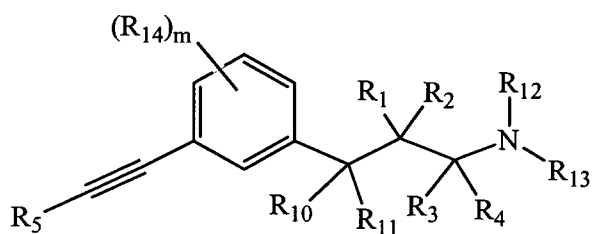
Formula (II)
