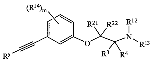
Formula (E)
