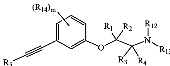
Formula (III)
