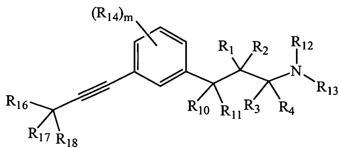
Formula (IIb)
