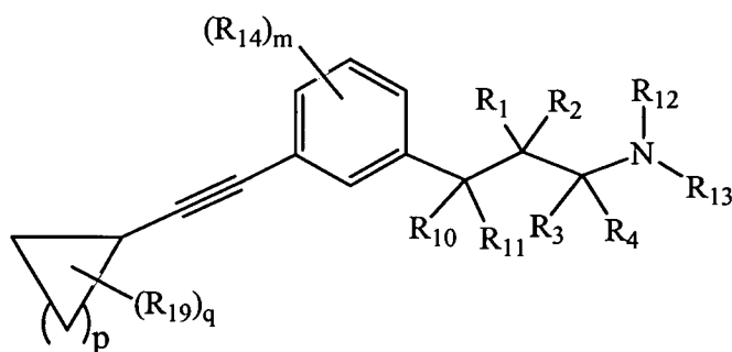
Formula (IIc)
