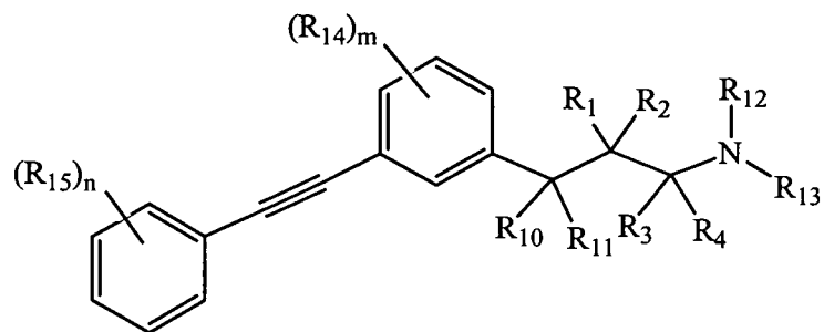
Formula (IIa)
