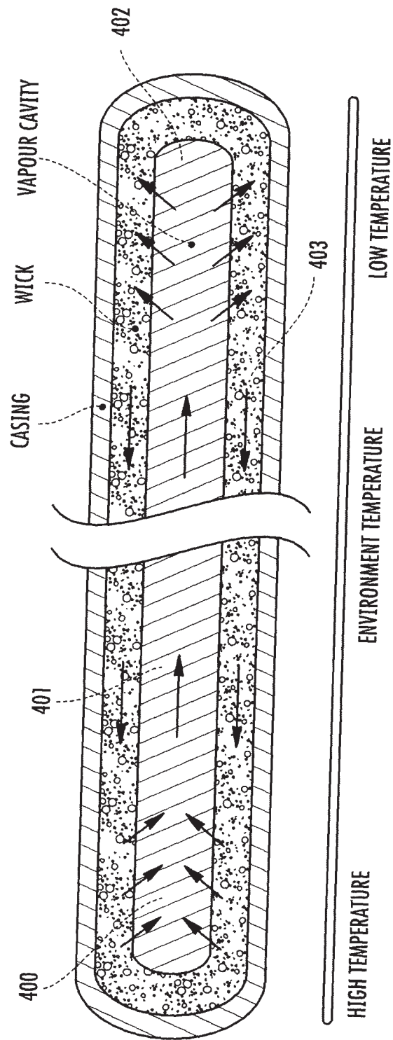
FIG. 7 PRIOR ART
